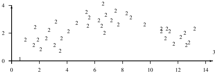
Figure 10.5 Single-link three-group solution for the data of Figure 10.4
