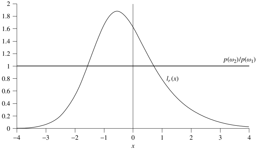
Figure 1.3 Likelihood function
