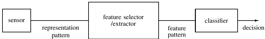
Figure 1.1 Pattern classifier
