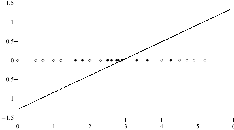
Figure 4.11 LDA regression for targets -1 and +1
