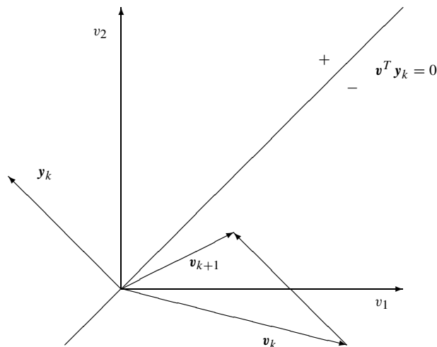
Figure 4.1 Perceptron training
