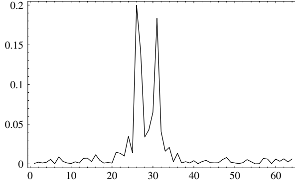
Figure 2.8 Proposal distribution
