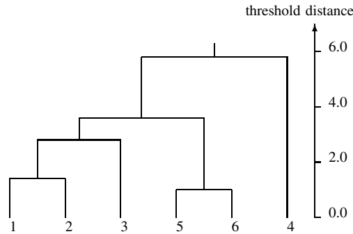
Figure 10.1 Dendrogram
