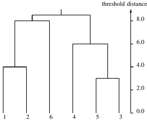
Figure 10.3 Single-link dendrogram
