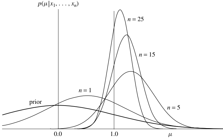
Figure 2.2 Bayesian learning of the mean of a normal distribution of known variance
