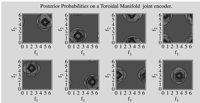
Figure 10.18 Joint encoding
