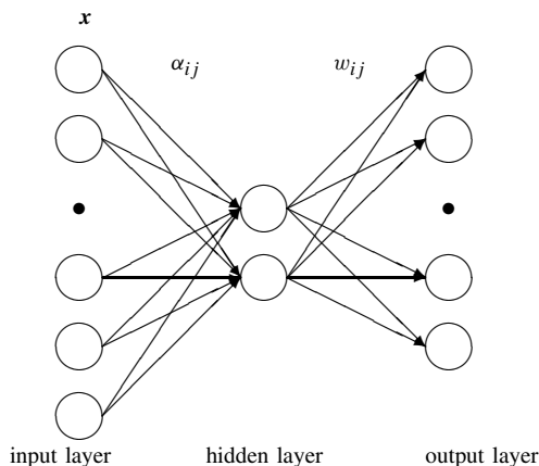
Figure 6.1 Multilayer perceptron
