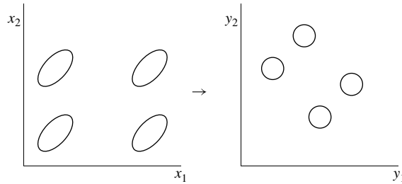
Figure 9.8 Illustration of the first stage of dimension reduction for four groups represented by contours \mathbf{x}^T \hat{\Sigma}_i^{-1} \mathbf{x} = \text{constant}
