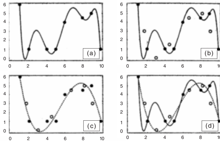
Figure 18. An example of over-training— (a) model with too many parameters to adjust the data, (b) a high error in the control data, (c) a model with less parameters approaches in the same way the training data and the validation data, (d) comparison of both models (Adapted from Castillo et al., 1999)
