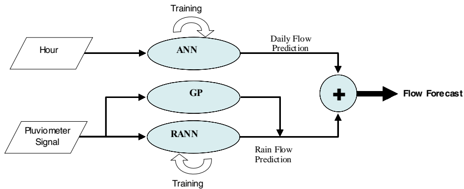
Figure 19. Diagram of the system's global functioning
