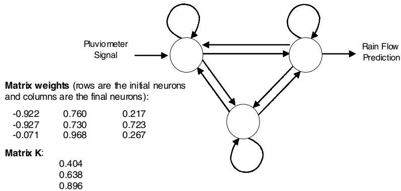
Figure 12. Architecture of the RANN
