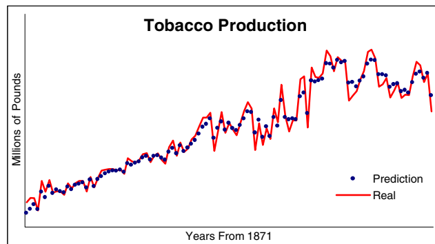
Figure 14. Tobacco series versus RANN predicted values
