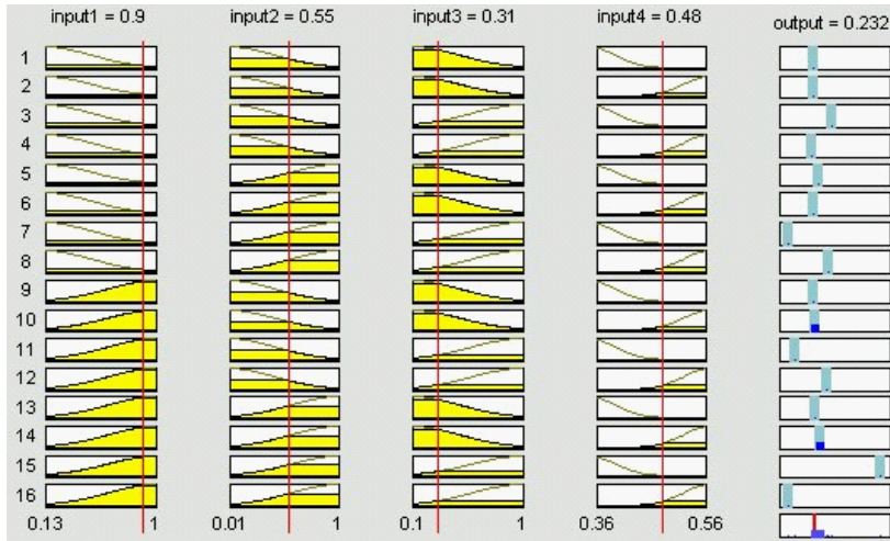
Figure 16. Behaviour of the system when it is presented with the following input pattern: SST=0.9, Thermic Anomaly=0.55, Chlorophyll=0.31, Altimetric Anomaly=0.48. The prediction of the system is 0.232. The real output is 0.22 and can be considered successful.
