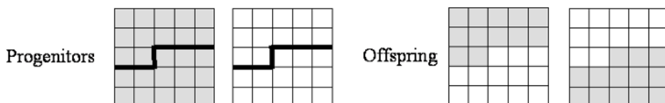
Figure 7. Crossover operator for weight matrices
