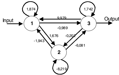
Figure 4. RANN that emulate the Mackey-Glass function
