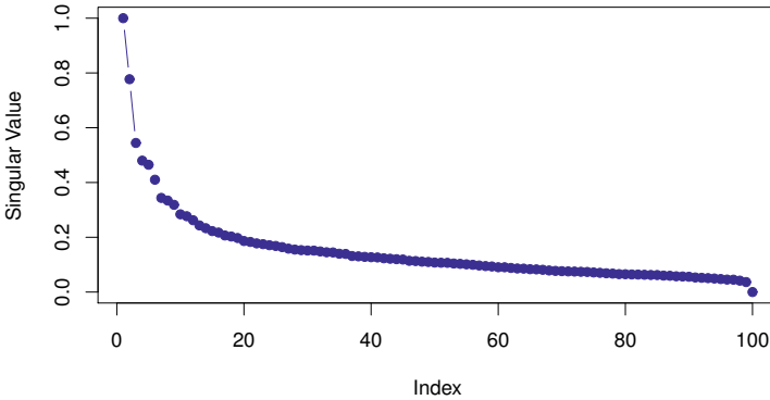
Figure 7.9 Singular values of the matrix \mathbf{Y} \in \mathbb{R}^{p \times K} using K = 100 frames from the video sequence. Note the rapid decay, showing that a low-rank approximation is possible.
