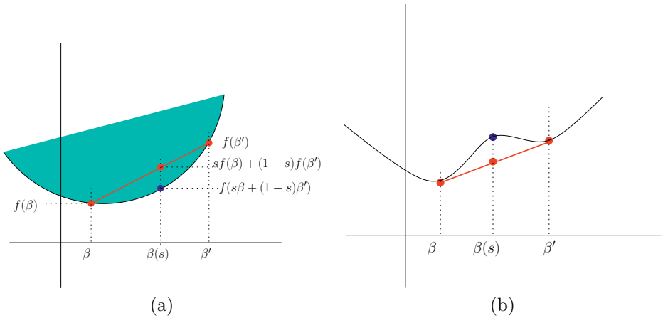
Figure 5.1 (a) For a convex function, the line sf(\beta) + (1 - s)f(\beta') always lies above the function value f(s\beta + (1 - s)\beta') . (b) A nonconvex function that violates the inequality (5.1). Without convexity, there may be local minima that are not globally minima, as shown by the point \beta' .
