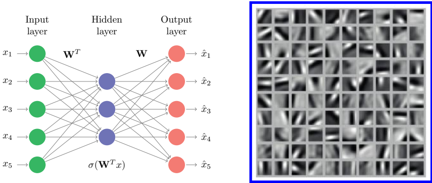
Figure 8.3 Left: Network representation of an autoencoder used for unsupervised learning of nonlinear principal components. The middle layer of hidden units creates a bottleneck, and learns nonlinear representations of the inputs. The output layer is the transpose of the input layer, and so the network tries to reproduce the input data using this restrictive representation. Right: Images representing the estimated columns of \mathbf{W} in an image modeling task.
