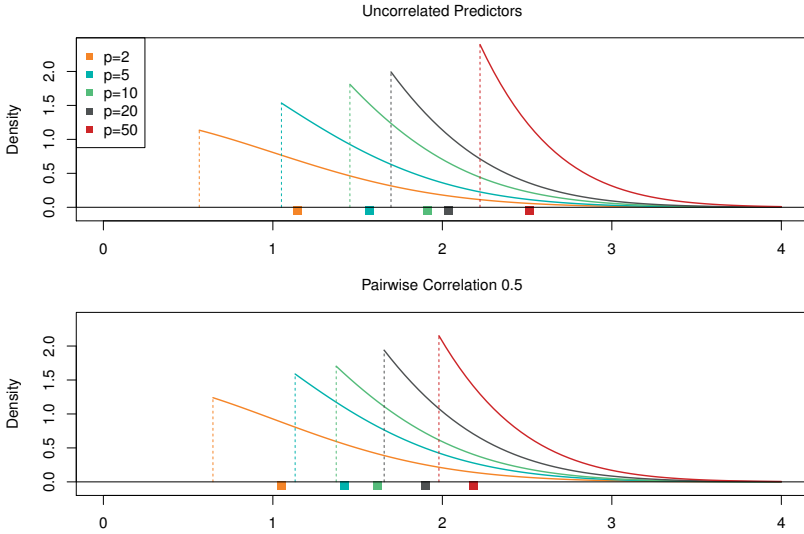
Figure 6.11 Simulation: N = 60 observations from the model with X_1, X_2, \dots, X_p \sim N(0, 1) , Y = \sum_j X_{ij} \beta_j + Z with Z \sim N(0, 1) , with all \beta_j = 0 ; two different predictor-correlation settings. The selection chooses the predictor j_1 having largest absolute inner product with \mathbf{y} . Shown is the truncated density on the left-hand side of (6.10) for p = 2, 5, 10, 20, 50 . The colored squares along the bottom show the average largest inner product in each setting.
