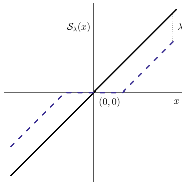
Figure 2.4 Soft thresholding function \mathcal{S}_\lambda(x) = \text{sign}(x)(|x| - \lambda)_+ is shown in blue (broken lines), along with the 45° line in black.
