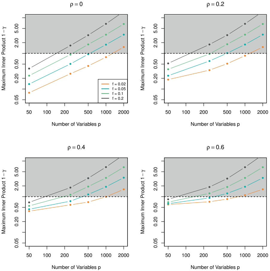
Figure 11.5 Irrepresentability condition in practice. Each plot shows values for 1 - \gamma in (11.27) for simulated Gaussian data. Values less than one are good, and the smaller the better. The sample size N = 1000 is fixed, and the number of predictors p varies along the horizontal axis. The fraction f = k/p of true nonzero coefficients (the sparsity level) varies within each panel, and finally, the correlation between each true predictor and its null predictor partner (as described in the text) varies across the four panels. A horizontal broken line is drawn at 1 - \gamma = 1 , below which the irrepresentability condition holds. Each point is a mean of 1 - \gamma over five simulations; the standard errors of the means are small, averaging about 0.03.
