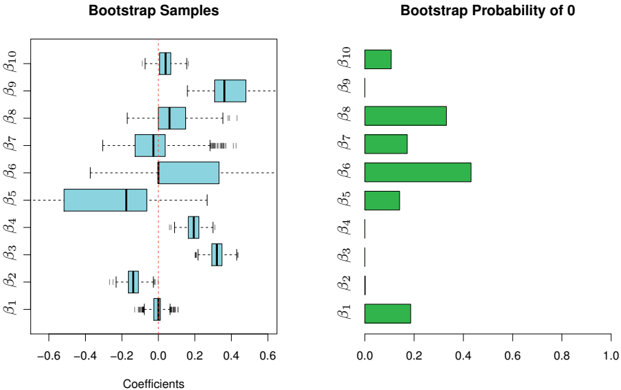
Figure 6.7 [Left] Boxplots of 1000 parametric bootstrap realizations of \widehat{\beta}^*(\widehat{\lambda}_{CV}) . Comparing with the corresponding Bayesian posterior distribution in Figure 6.3, we again see a close correspondence. [Right] Proportion of times each coefficient is zero in the bootstrap distribution.
