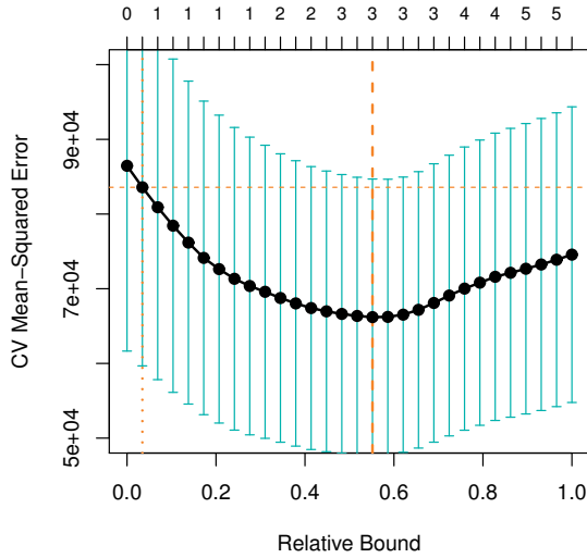
Figure 2.3 Cross-validated estimate of mean-squared prediction error, as a function of the relative \ell_1 bound \hat{t} = \|\hat{\beta}(t)\|_1 / \|\tilde{\beta}\|_1 . Here \hat{\beta}(t) is the lasso estimate corresponding to the \ell_1 bound t and \tilde{\beta} is the ordinary least-squares solution. Included are the location of the minimum, pointwise standard-error bands, and the “one-standard-error” location. The standard errors are large since the sample size N is only 50.
