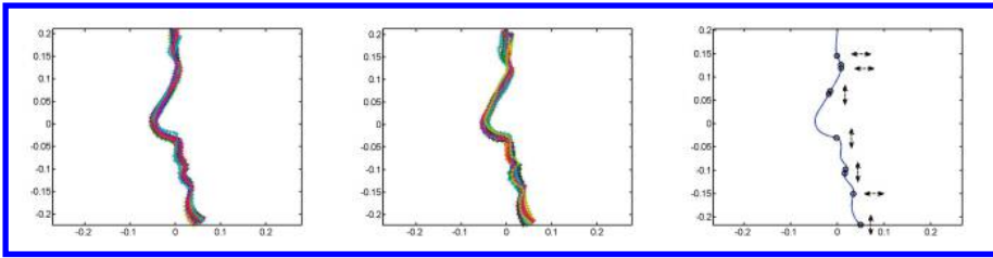
Figure 8.8 The silhouettes and the 65 (x, y) -coordinates for females (left) and males (middle). Right: The mean shape of the silhouettes, and the 10 (x, y) -coordinates in the SDA model. The superimposed dots indicate the landmarks retained in the sparse discriminant vector. The arrows illustrate the directions of the differences between male and female classes.
