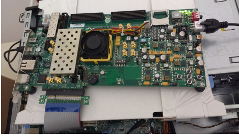
Figure 7. Development platform
