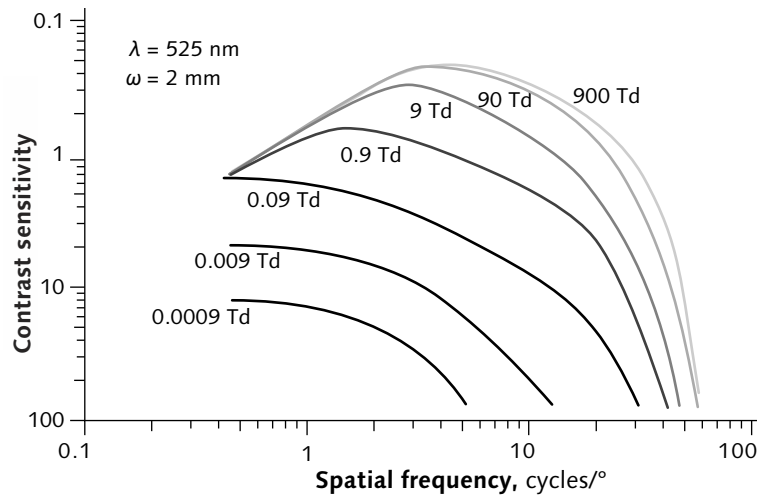
Figure 19.5 Contrast sensitivity function (CSF) varies with retinal illuminance, here shown in units of troland (Td). The curve at 9 Td, which typifies television viewing, peaks at about 4 cycles per degree (CPD, or \sim/^\circ ). Below that spatial frequency, the eye acts as a differentiator; above it, the eye acts as an integrator.
