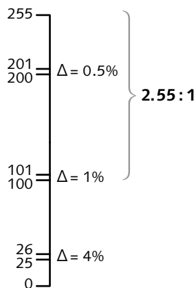
Figure 1.15 The “ code 100 ” problem with linear-light coding is that at code levels below 100, the steps between code values have ratios larger than the visual threshold: The steps are liable to be visible.
