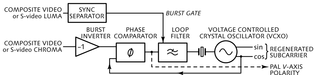
Figure 28.9 Subcarrier regeneration
