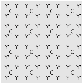
Figure 10.2 Subsampling schemes are summarized here. C indicates a [C B , C R ] sample pair when located at the same site; otherwise (as in the DV schemes) individual C B and C R notations indicate the centers of the respective chroma samples. Y' indicates the center of a luma sample. The schemes in the left column are progressive. The schemes in the right column are interlaced; there, black letters indicate top field samples and gray letters indicate bottom field samples.
