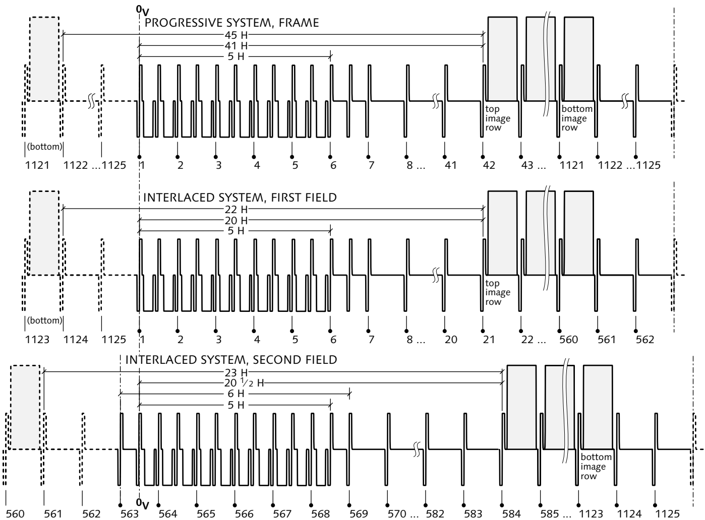
Figure 4.7.2 1080i and 1080p vertical blanking interval
