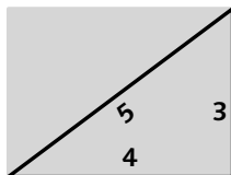
Figure 1.12 Picture height at an aspect ratio of 4:3 is 3/5 of the diagonal; optimum viewing distance for conventional video is 4.25 times the diagonal. Picture height at 16:9 is about half the diagonal; optimum viewing distance for 2 Mpx HDTV is 1.5 times the diagonal.
