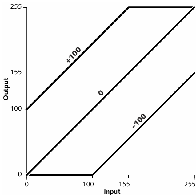
Figure 3.7 BRIGHTNESS control in Photoshop applies an offset of -100 to +100 to R'G'B' components ranging from 0 to 255. If a result falls outside the range 0 to 255, it saturates; headroom and footroom are absent. The function is evidently linear, but depending upon the image coding standard in use, the input and output values are generally nonlinearly related to luminance (or tristimulus values).
