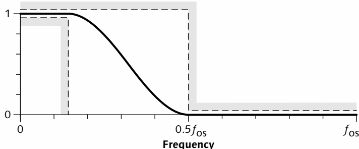
Figure 17.5 Analog filter for 2x-oversampling is much less demanding than a filter for direct sampling, because the difficult part of filtering – achieving a response comparable to that of Figure 17.4 – is relegated to the digital domain.
