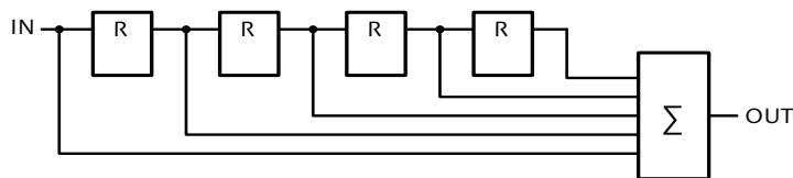
Figure 16.16 Block diagram of 5-tap FIR filter
