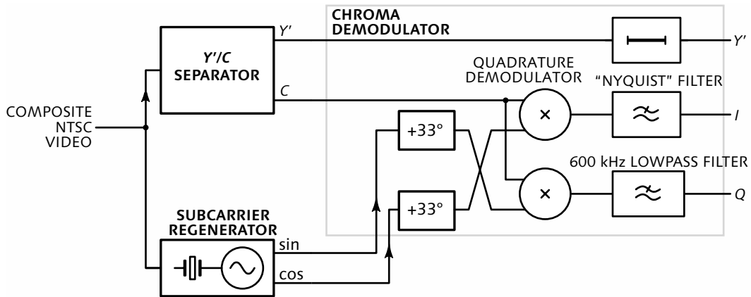
Figure 30.3 NTSC decoder using Y'I/Q is similar to the decoder using Y'UV that I presented in Figure 28.5, on page 341. Phase shifts of 33^\circ are applied to the sine and cosine phases of subcarrier. The Q lowpass filter has a corner of 600 kHz; the I lowpass filter has a special "Nyquist" shape detailed in Figure 30.4 overleaf. The 33^\circ phase shifters and the Nyquist filter are useful only if the signal was encoded on [I, Q] axes with wideband I and narrowband Q . Because proper Y'I/Q encoding has not been practiced since about 1970, using this textbook Y'I/Q decoder is pointless.
