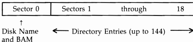
Figure 15-5. Track 18, the Directory Track
