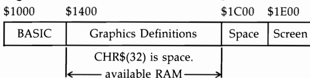
Figure 12-16. Incomplete Graphics Memory Maps
