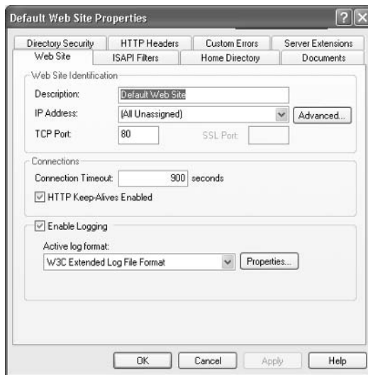
FIGURE 6.18 The website Properties dialog box
