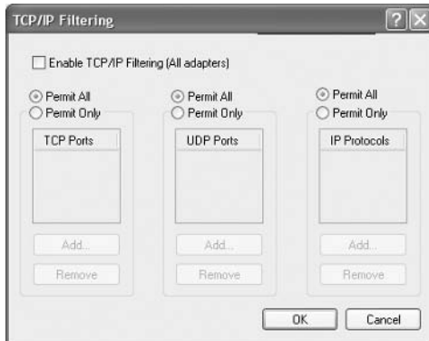
FIGURE 6.6 The TCP/IP Filtering dialog box
