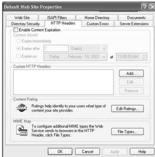
FIGURE 6.24 The HTTP Headers tab of the website Properties dialog box
