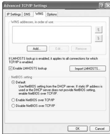
FIGURE 6.4 The WINS tab of the Advanced TCP/IP Settings dialog box
