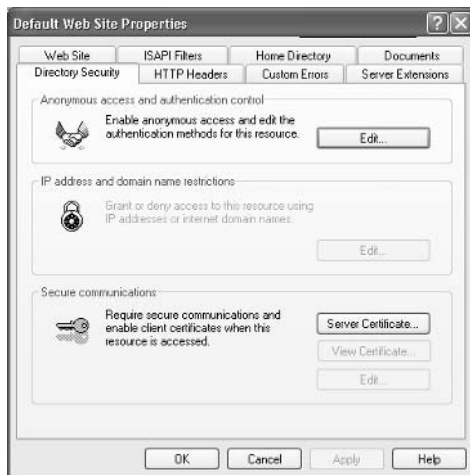
FIGURE 6.22 The Directory Security tab of website Properties dialog box
