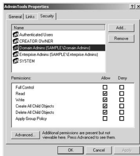
FIGURE 5.6 The Security tab of the GPO's Properties dialog box, with default settings
