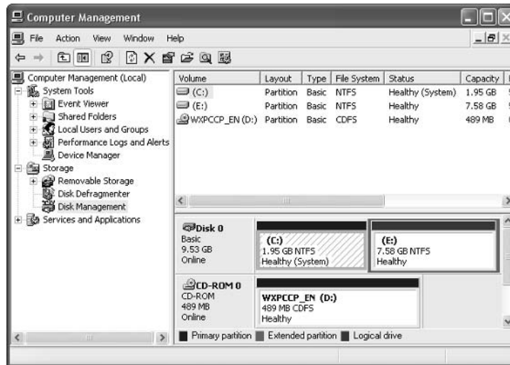
FIGURE 3.1 The Disk Management window
