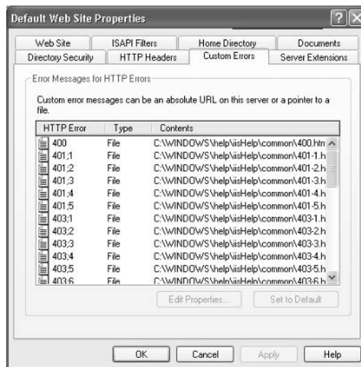
FIGURE 6.25 The Custom Errors tab of the website Properties dialog box
