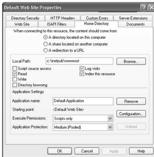
FIGURE 6.20 The Home Directory tab of the website Properties dialog box
