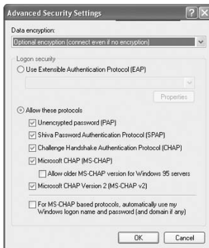
FIGURE 6.14 Connection Properties, Security tab, Advanced Settings dialog box
