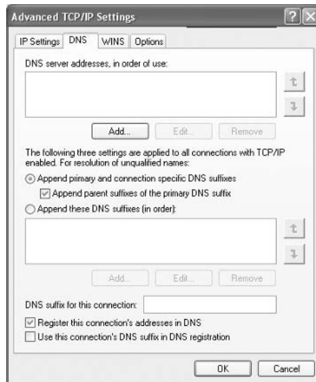
FIGURE 6.3 The DNS tab of the Advanced TCP/IP Settings dialog box
