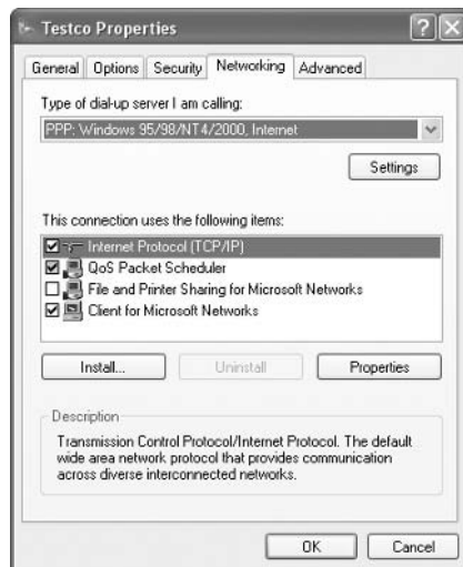
FIGURE 6.15 The Networking tab of the Connection Properties dialog box
