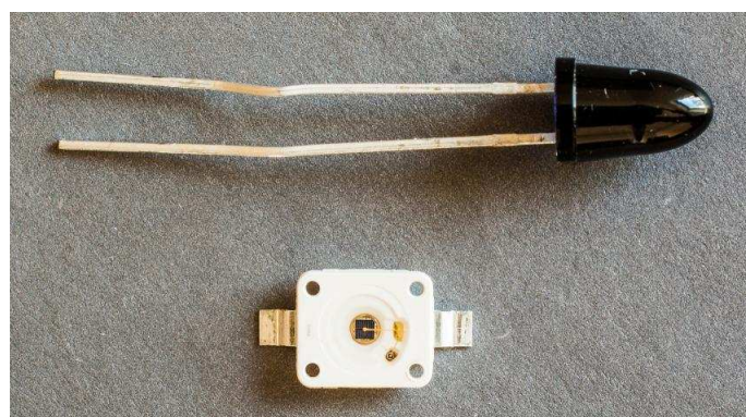
Figure 3 – Infrared Emitters – Top: SFH4545, Bottom: SFH4233
