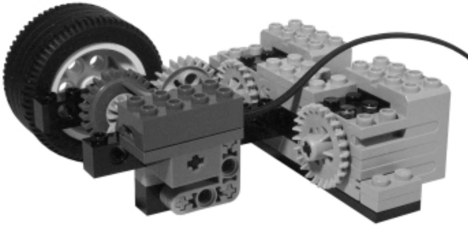
Figure 27.3 Flipping Light Sensor Assembly (Side View, Left Wheel Removed)
