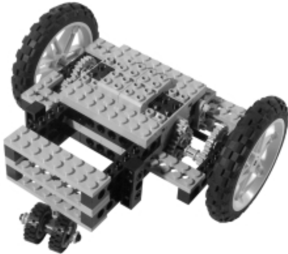
Figure 24.6 The Differential Drive that Controls Motion
