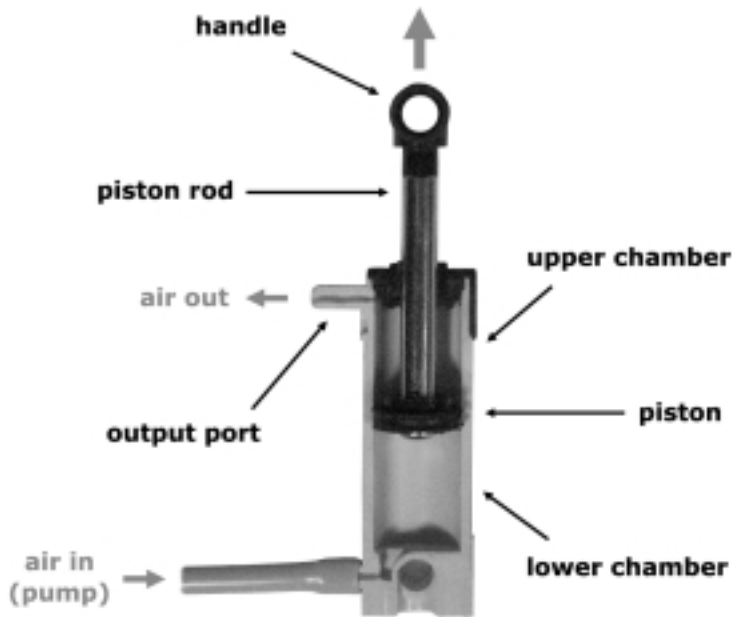
Figure 10.3 Cutaway of the Large Cylinder in Action
