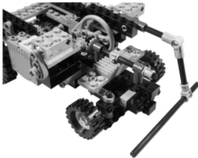
Figure 14.19 Detail of the Rack and Pinion Steering Assembly
