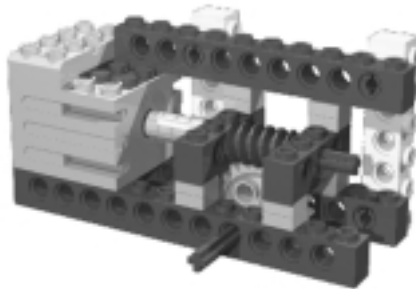
Figure 3.3 A Motor Connected to a Worm Gear
