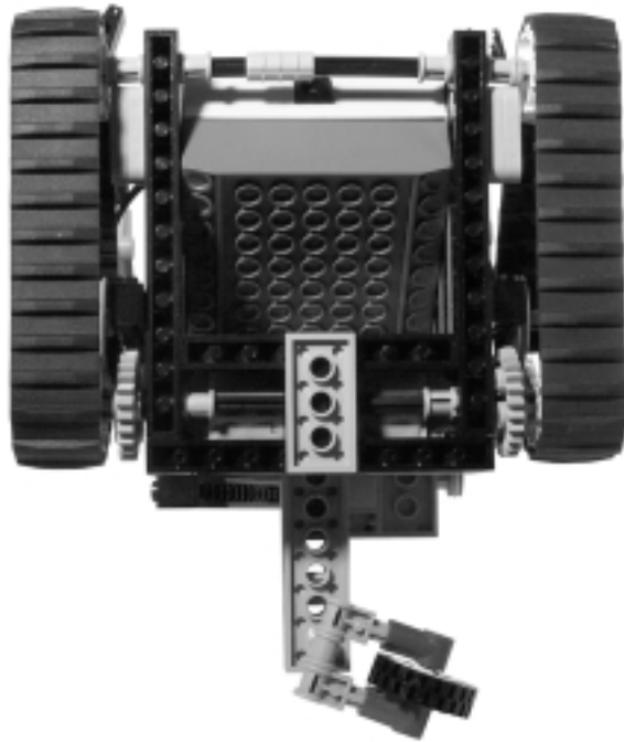
Figure 18.15 Johnny Five Bottom View
