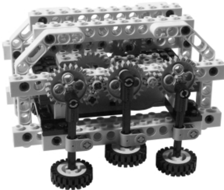
Figure 15.22 The Left Leg Group
