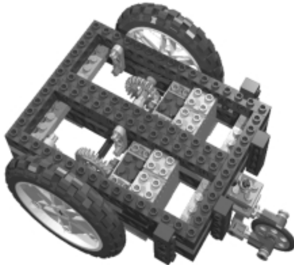
Figure 5.7 A Complete Platform
