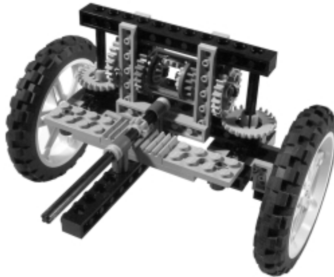
Figure 14.23 A MINDSTORMS-Only Front-Wheel Drive Assembly
