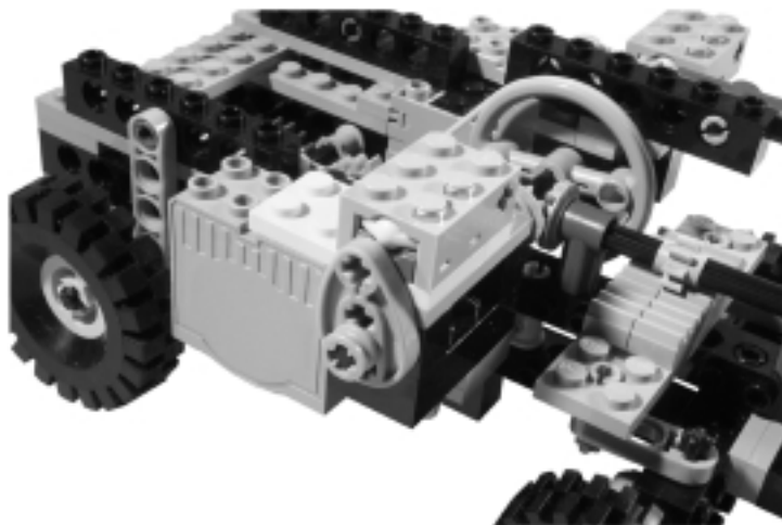
Figure 14.21 The Touch Sensor that Monitors the Steering
