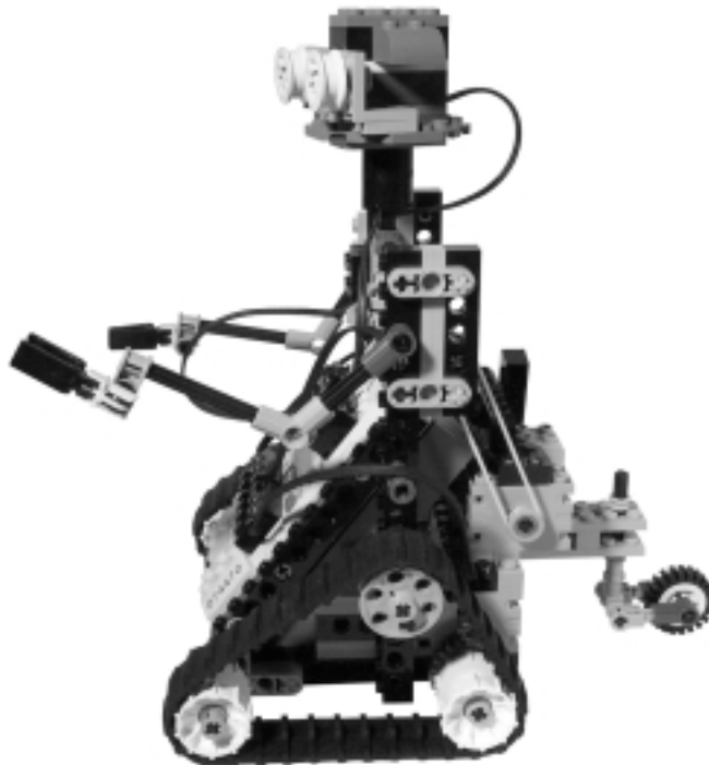
Figure 18.13 Johnny Five Side View
