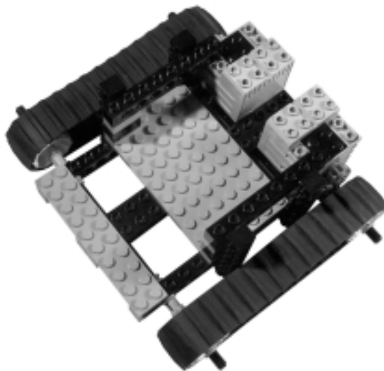
Figure 8.10 A Tracked Skid-Steer Drive
