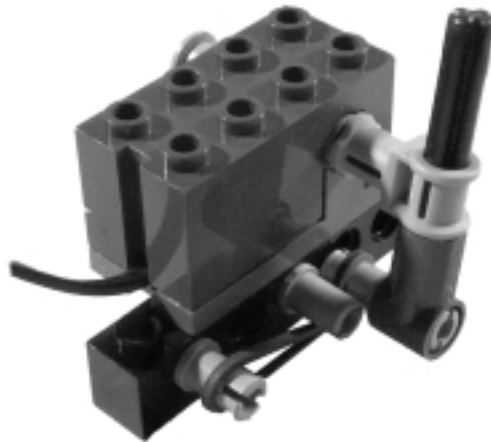
Figure 4.10 Emulating a Touch Sensor with a Rotation Sensor
