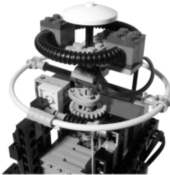
Figure 18.8 The Head Mechanism
