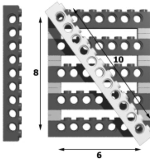
Figure 1.9 Pythagoras' Theorem
