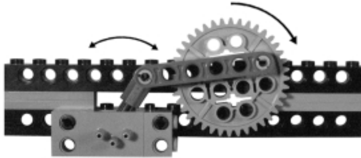
Figure 10.9 A Cycling Valve
