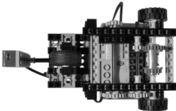
Figure 14.10 Bottom View: The Gearings
