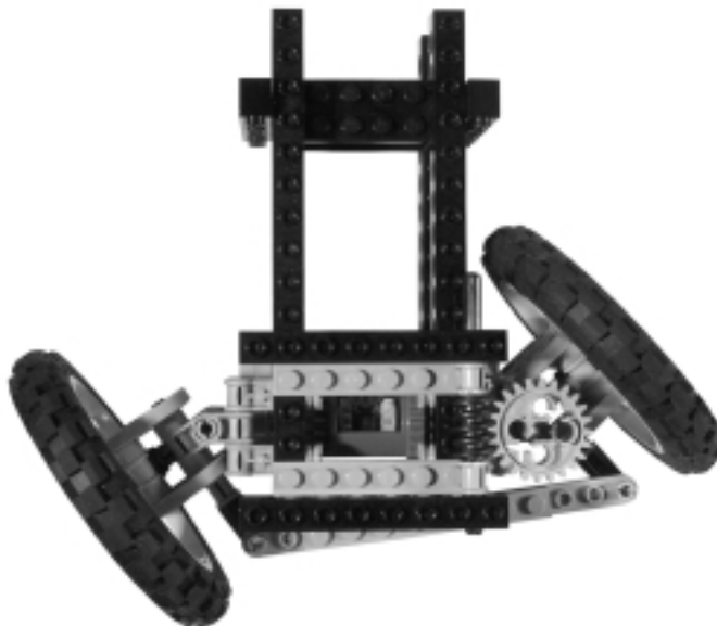
Figure 14.26 This Design Features Ackerman Correction
