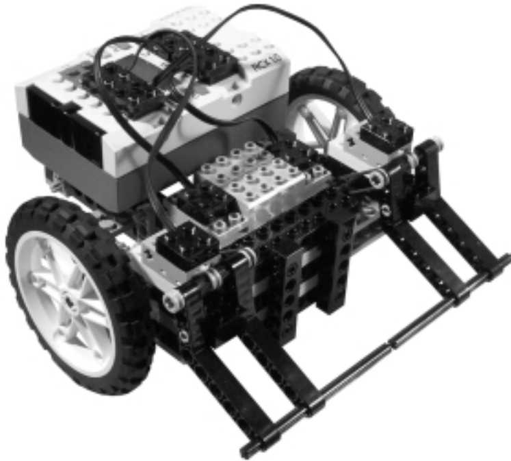
Figure 14.4 The Robot, Complete with RCX and Bumpers
