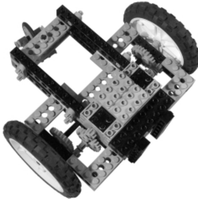
Figure 14.2 Detail of the Two-Stage Gear Train
