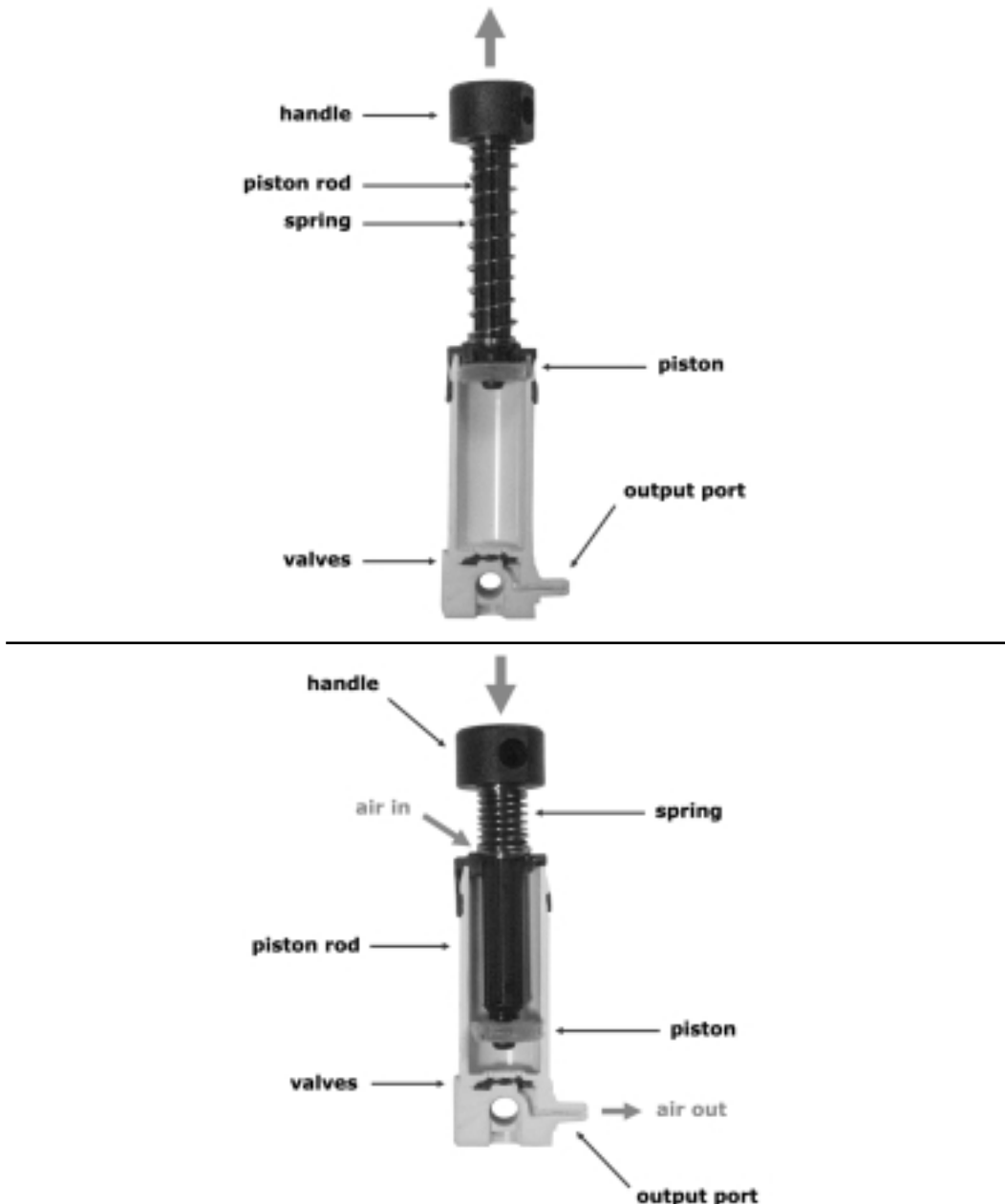
Figure 10.2 Cutaway of the Large Pump in Action
