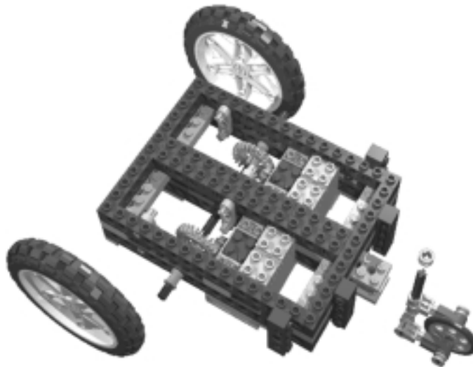
Figure 5.10 ...and the Wheels
