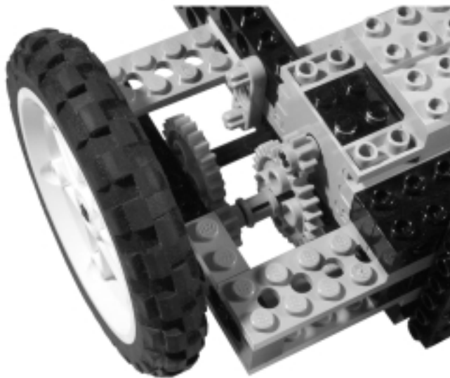
Figure 14.2 Detail of the Two-Stage Gear Train
