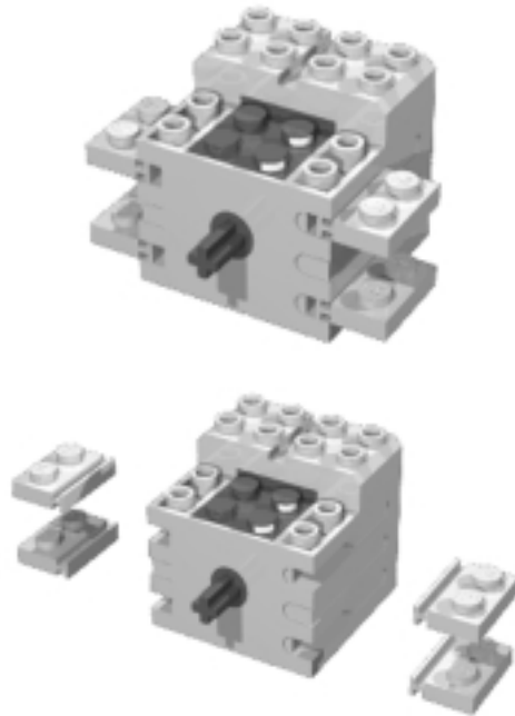
Figure 3.5 An Easily Removable Motor
