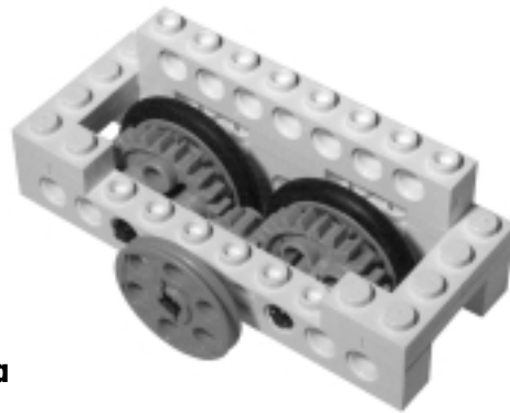
Figure 18.11 A Double-Wheeled Leg
