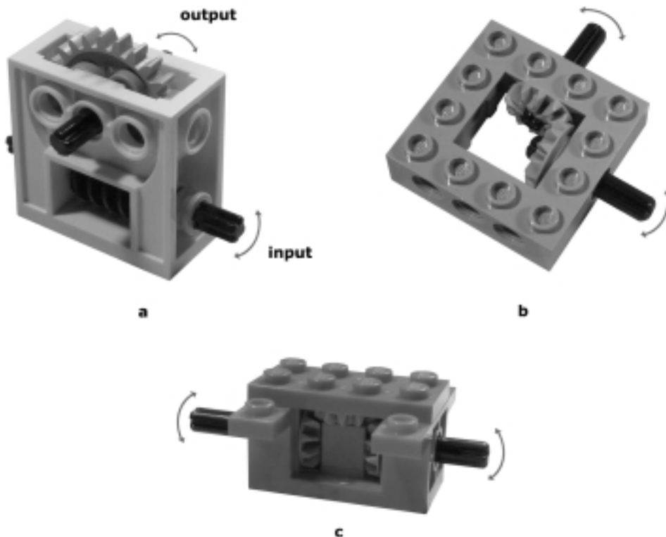
Figure 9.3 Gearboxes
