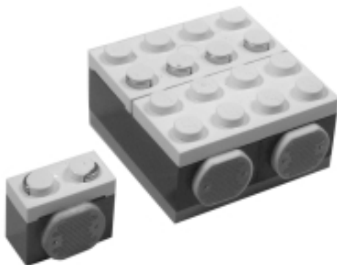
Figure 9.10 Single and Double CdS Light Sensors
