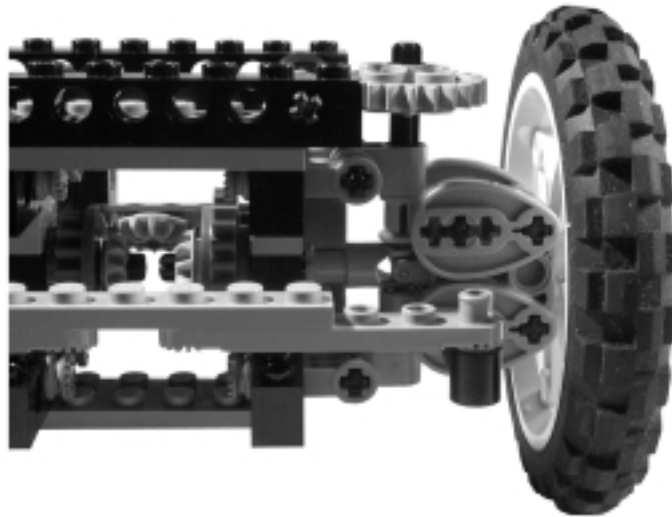
Figure 14.26 This Design Features Ackerman Correction
