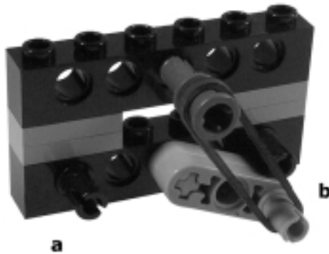
Figure 11.4 A Simple Bi-Stable Mechanism
