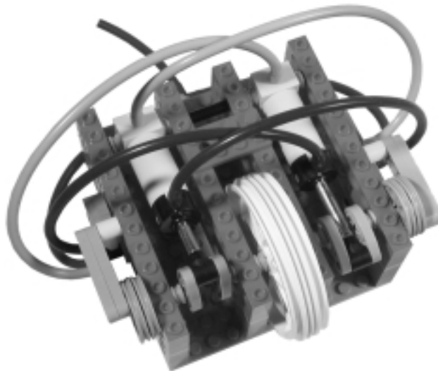
Figure 10.20 Soh's Pneumatic Engine
