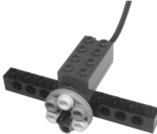
Figure 4.12 Emulating a Rotation Sensor with a Light Sensor
