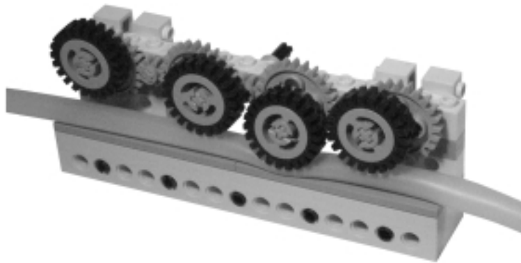
Figure 25.15 A Possible Setup for an Indirect Pumping Technique
