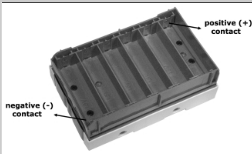
Figure 25.13 Opening Your RCX
