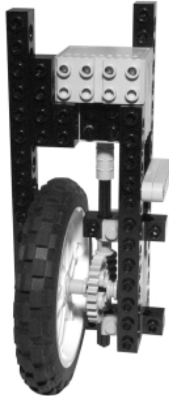
Figure 16.12 A Wheel Assembly
