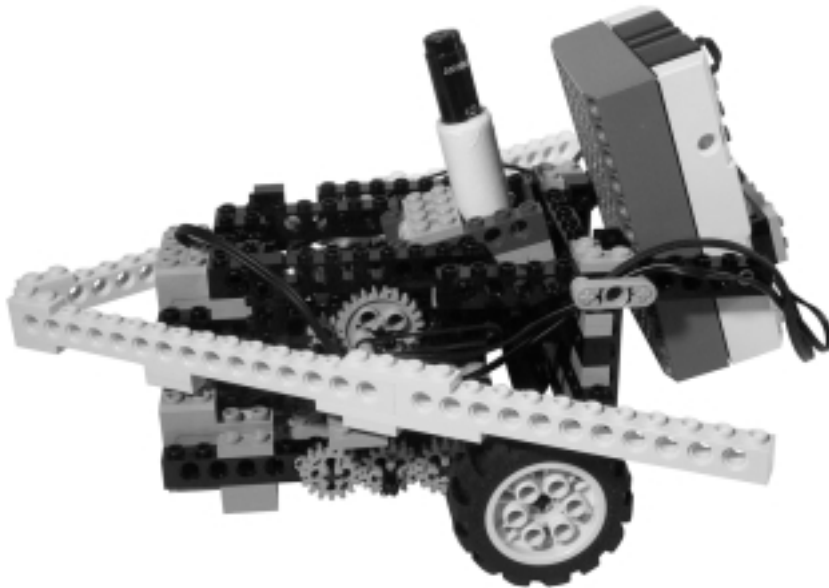
Figure 23.6 Side View of the Turtle Ready for Operation
