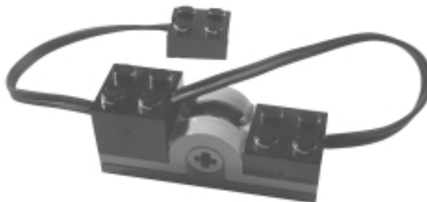
Figure 4.13 Emulating a Rotation Sensor with a Polarity Switch
