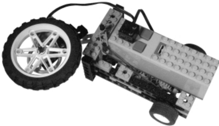
Figure 19.10 A Purely Mechanical Wall Follower
