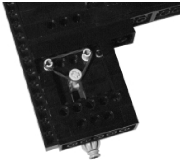
Figure 22.5 Detail of the Launching Mechanism (Bottom View)
