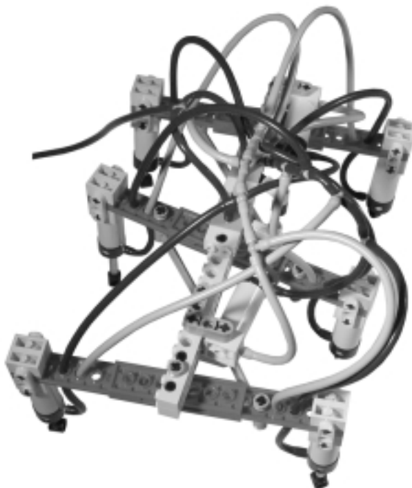
Figure 10.18 Bert van Dam's Pneumatic Insect
