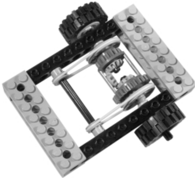
Figure 8.16 A Limited Slip Differential
