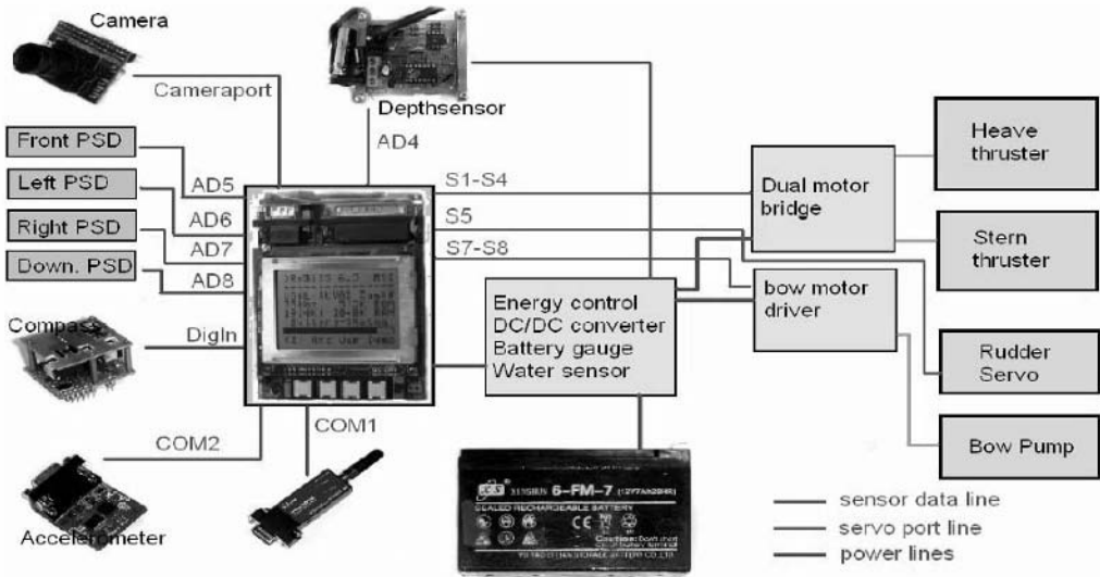
Figure 12.10: USAL system overview
