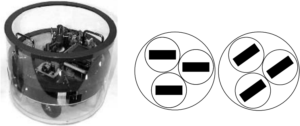
Figure 7.8: Xenia, University of Kaiserslautern, with schematic diagrams
