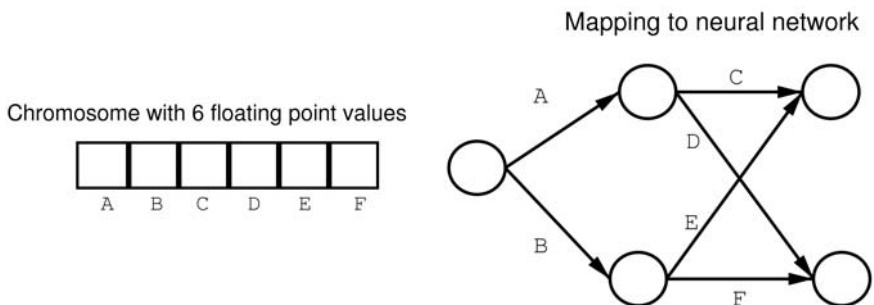
Figure 22.8: Chromosome encoding
