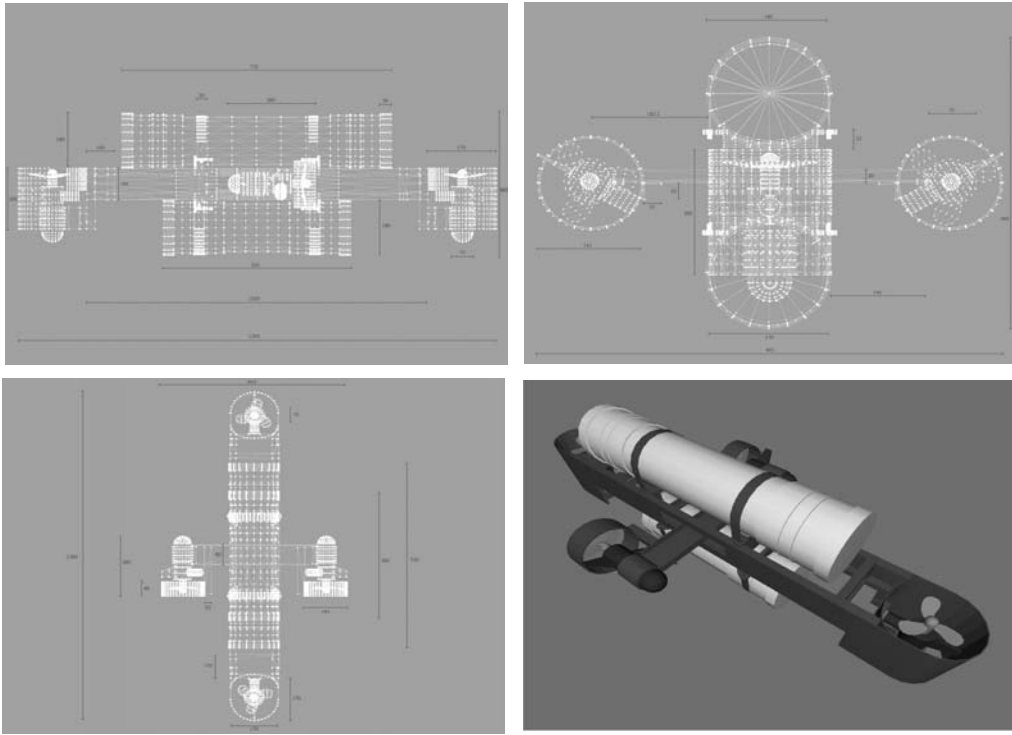
Figure 12.3: Mako design
