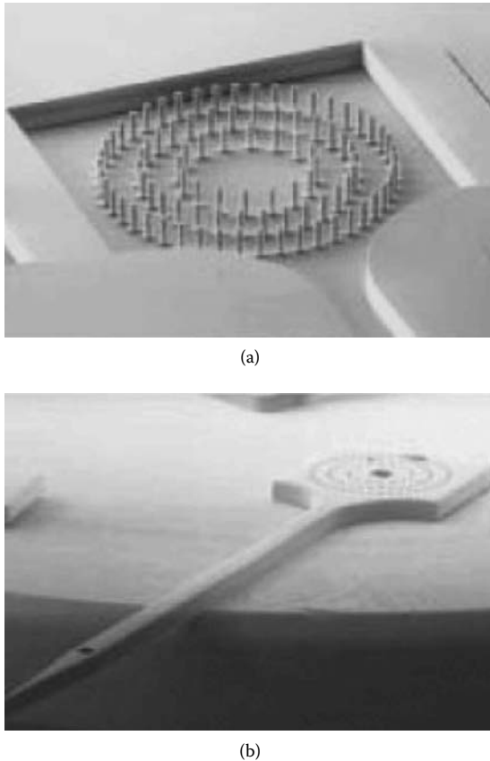
FIGURE 12.4 (a) SEM of a microneedle mold. (b) SEM of a polysilicon hypodermic microneedle fabricated by polymolding technique. (From J. Zahn, N. Talbot, D. Liepmann, and A. Pisano, Biomedical Microdevices , 2, 295–303, 2000. With permission.)
