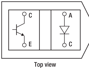
Figure 4-7. IR sensor schematic (detector or photo-transistor = Left, Emitter = Right)
