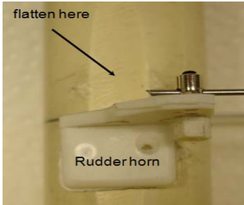
Figure 9-30. A rudder horn, glued to the tube
