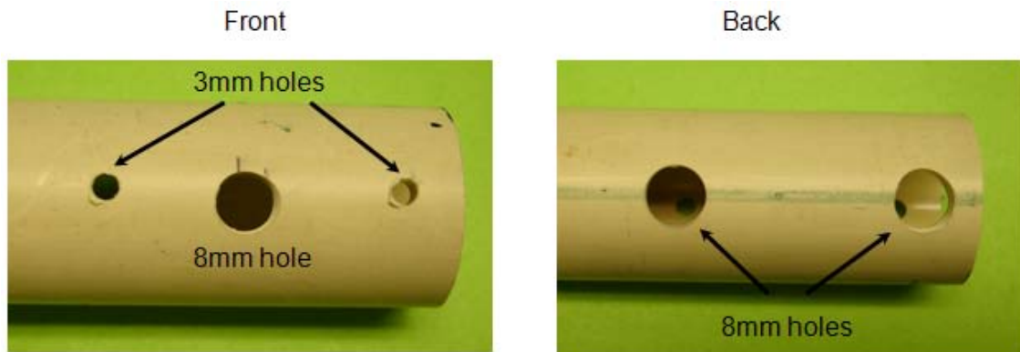
Figure 9-29. Mounting holes for the motor
