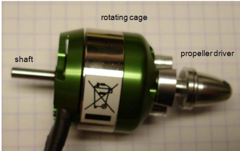
Figure 9-31. A BLDC outrunner motor
