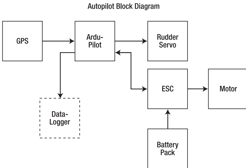
Figure 9-32. Block diagram of the electronics
