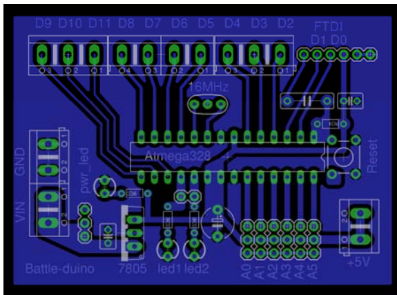
Figure 12-4. The Battle-duino Eagle layout file
