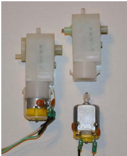
Figure 3-5. Here you can see a small DC gear motor (left) and again with the DC motor removed from the plastic gear box.
