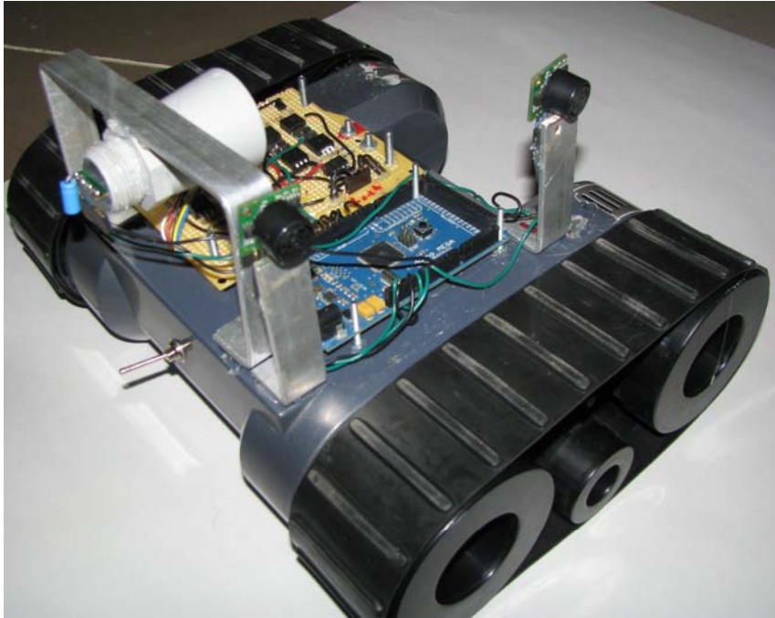
Figure 5-18. This is a photo of all three sensors installed on Wally. The two side sensors are a different model than the larger center sensor, but they are all three made by Maxbotix and have the same output pins, meaning that they are read by the Arduino in the same way.
