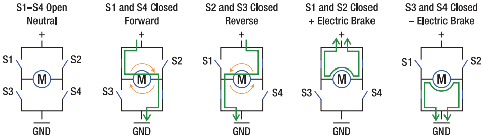
Figure 3-11. Acceptable H-bridge states
