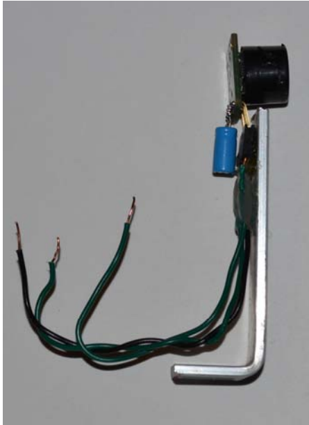
Figure 5-16. This image shows the sensor glued to the sensor bracket.
