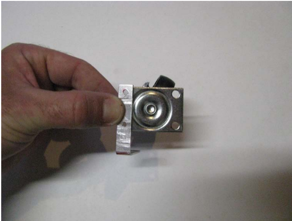
Figure 4-24. Drill holes through “L” bracket where marked.
