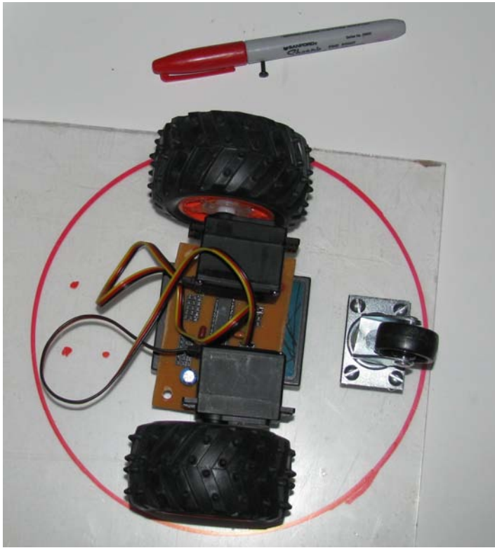
Figure 7-10. Lay the motors and castor wheels onto the plexiglass, and mark the outline of the drive wheels and the mounting holes for the castor wheels.
