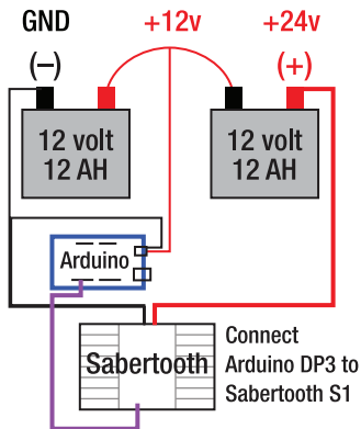
Figure 11-17. Here you can see the basic wiring diagram between the Arduino, Sabertooth, and batteries. The Sabertooth requires a 24v supply whereas the Arduino requires a 12v supply.
