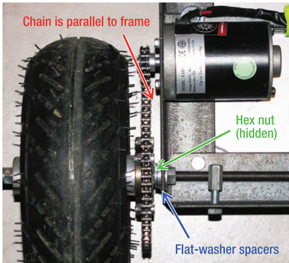
Figure 12-19. Drive-train installation
