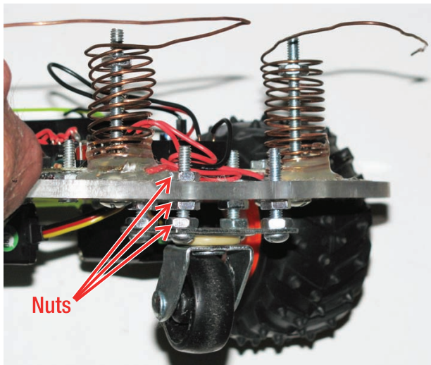
Figure 7-14. Use three nuts on each bolt to make both castor wheels adjustable in height.
