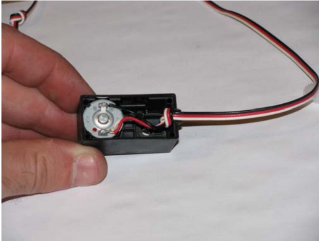
Figure 4-19. Solder the red and white wires to the motor terminal with the red dot beside it, and the black wire to the other terminal. Now it is ready to be re-assembled.
