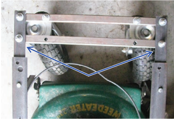
Figure 10-8. The main frame rails connected to the front caster wheel support braces
