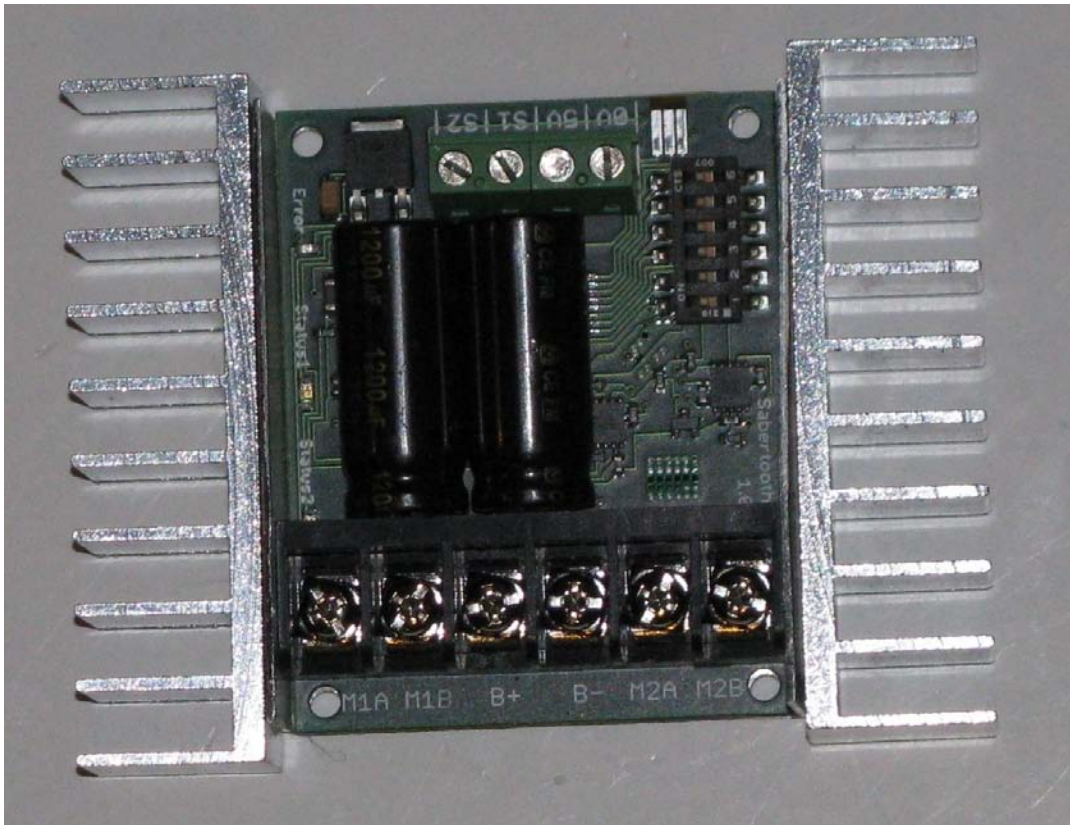
Figure 11-13. The Sabertooth 2x25 motor controller
