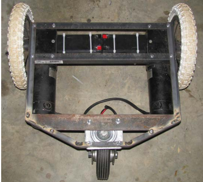
Figure 8-3. Explorer-bot frame
