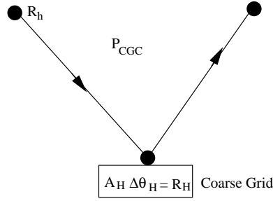
Figure 7.36: Schematic of the coarse-grid correction stage.
