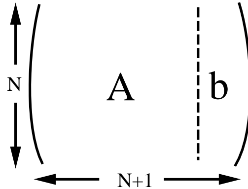
Figure 9.8: The augmented matrix consists of the original matrix A with the right-hand-side vector \mathbf{b} appended as an additional column.
