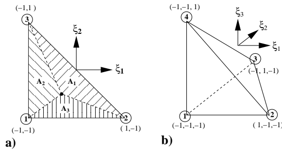
Figure 3.14: (a) The area coordinate system in the standard triangular region. Each coordinate l_1, l_2 , and l_3 can be interpreted as the ratio of areas A_1, A_2 , and A_3 over the total area. (b) The standard tetrahedral region for the definition of volume coordinates.
