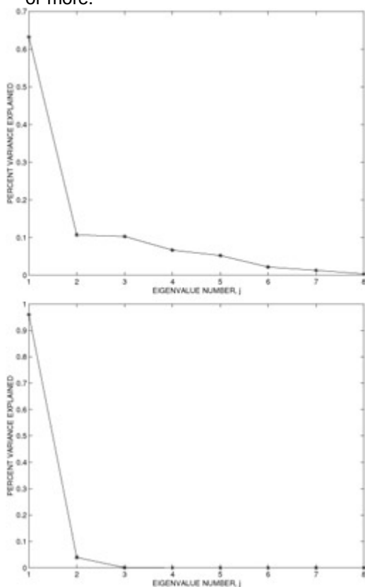
Figure 3.17: Scree Plots for the Computer CPU Data Set. The Upper Plot Displays the Eigenvalues From the Correlation Matrix, and the Lower Plot is for the Covariance Matrix.
