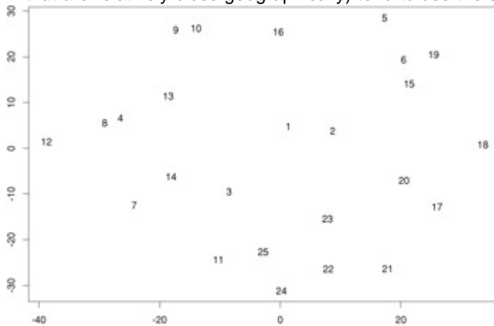
Figure 3.19: A Multidimensional Scaling Plot of the Village Dialect Similarities Data.
