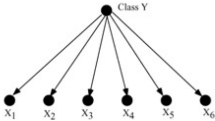
Figure 6.10: The First-Order Bayes Graphical Model Structure, With a Single Class Y and 6 Conditionally Independent Feature Variables X_1, \dots, X_6 .
