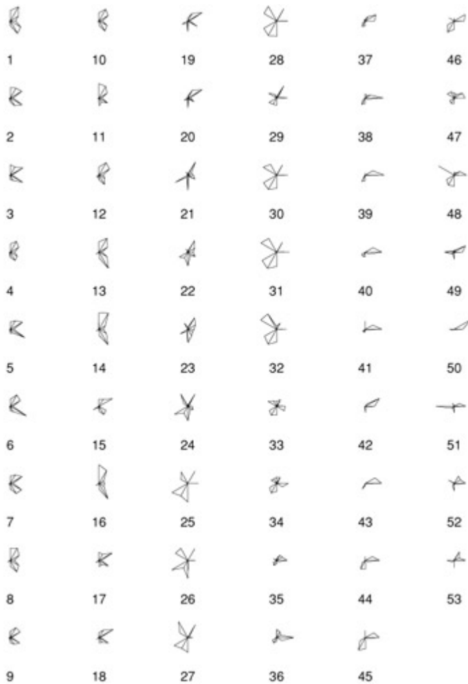
Figure 3.15: An Example of a Star Plot.
