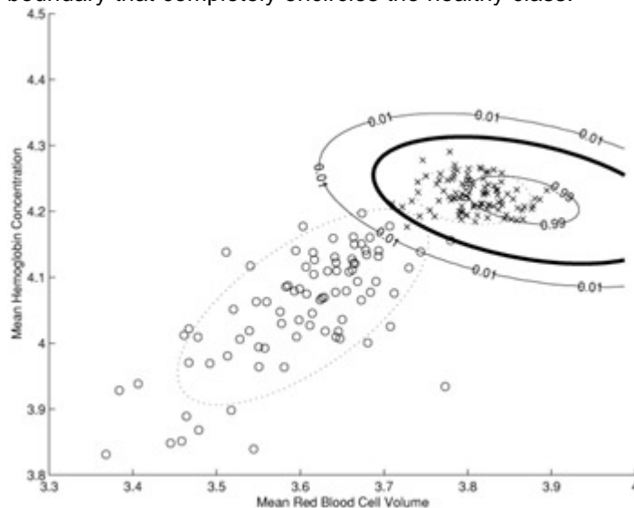
Figure 10.2: Posterior Probability Contours for p(c_1|x) Where c_1 is the Label for the Healthy Class for the Red Blood Cell Data Discussed in Chapter 9. The Heavy Line is the Decision Boundary ( p(c_1|x) = p(c_2|x) = 0.5 ) and the Other Two Contour Lines Correspond to p(c_1|x) = 0.01 and p(c_1|x) = 0.99 . Also Plotted for Reference are the Original Data Points and the Fitted Covariance Ellipses for Each Class (Plotted as Dotted Lines).
