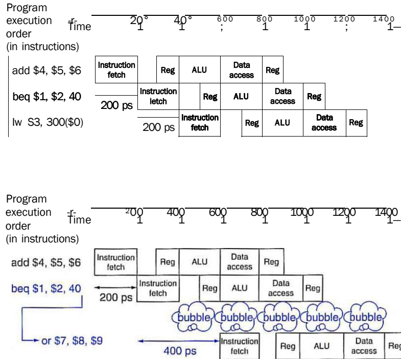
FIGURE 4.32 Predicting that branches are not taken as a solution to control hazard. The top drawing shows the pipeline when the branch is not taken. The bottom drawing shows the pipeline when the branch is taken. As we noted in Figure 4.31, the insertion of a bubble in this fashion simplifies what actually happens, at least during the first clock cycle immediately following the branch. Section 4.8 will reveal the details.
