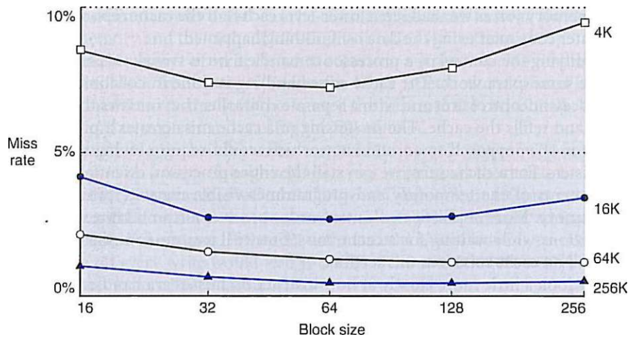
FIGURE 5.8 Miss rate versus block size. Note that The miss rate actually goes up if the block size is too large relative to the cache size. Each line represents a cache of different size. (This figure is independent of associativity, discussed soon.) Unfortunately, SPEC2000 traces would take too long if block size were included, so this data is based on SPEC92.
