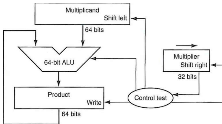
FIGURE 3.4 First version of the multiplication hardware. The Multiplicand register, ALU, and Product register are all 64 bits wide, with only the Multiplier register containing 32 bits. (Appendix C describes ALUs.) The 32-bit multiplicand starts in the right half of the Multiplicand register and is shifted left 1 bit on each step. The multiplier is shifted in the opposite direction at each step. The algorithm starts with the product initialized to 0. Control decides when to shift the Multiplicand and Multiplier registers and when to write new values into the Product register.
