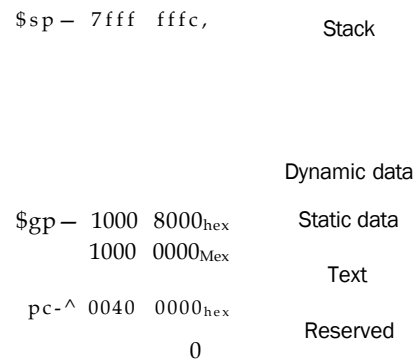
FIGURE 2.13 The MIPS memory allocation for program and data. These addresses are only a software convention, and not part of the MIPS architecture. The stack pointer is initialized to 7fff\ fffc_{hex} and grows down toward the data segment. At the other end, the program code ("text") starts at 0040\ 0000_{hex} . The static data starts at 1000\ 0000_{hex} . Dynamic data, allocated by malloc in C and by new in Java, is next. It grows up toward the stack in an area called the heap. The global pointer, $gp , is set to an address to make it easy to access data. It is initialized to 1000\ 8000_{hex} so that it can access from 1000\ 0000_{hex} to 1000\ ffff_{hex} using the positive and negative 16-bit offsets from $gp . This information is also found in Column 4 of the MIPS Reference Data Card at the front of this book.
