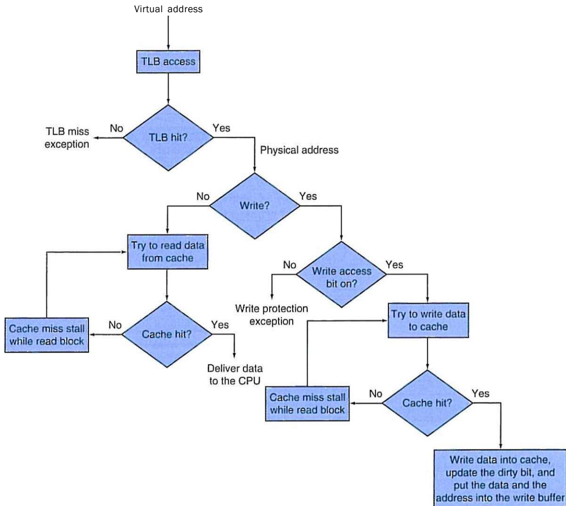
FIGURE 5.25 Processing a read or a write-through in the Intrinsity FastMATH TLB and cache. If the TLB generates a hit, the cache can be accessed with the resulting physical address. For a read, the cache generates a hit or miss and supplies the data or causes a stall while the data is brought from memory. If the operation is a write, a portion of the cache entry is overwritten for a hit and the data is sent to the write buffer if we assume write-through. A write miss is just like a read miss except that the block is modified after it is read from memory. Write-back requires writes to set a dirty bit for the cache block, and a write buffer is loaded with the whole block only on a read miss or write miss if the block to be replaced is dirty. Notice that a TLB hit and a cache hit are independent events, but a cache hit can only occur after a TLB hit occurs, which means that the data must be present in memory. The relationship between TLB misses and cache misses is examined further in the following example and the exercises at the end of this chapter.
