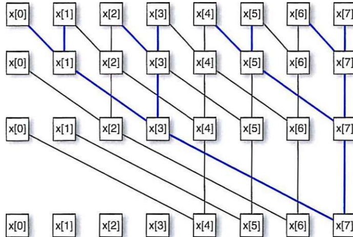
FIGURE A.8.8 Tree-based parallel scan data references.
