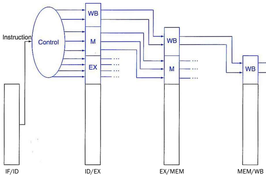
FIGURE 4.50 The control lines for the final three stages. Note that four of the nine control lines are used in the EX phase, with the remaining five control lines passed on to the EX/MEM pipeline register extended to hold the control lines; three are used during the MEM stage, and the last two are passed to MEM/WB for use in the WB stage.
