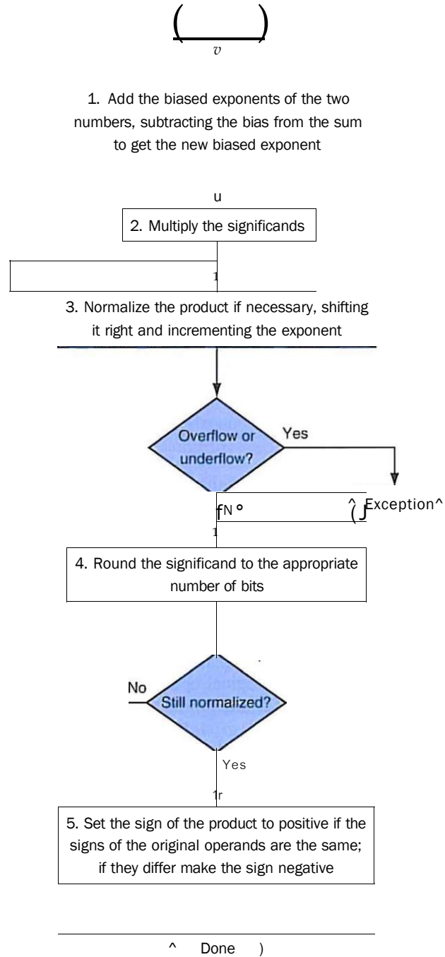
FIGURE 3.17 Floating-point multiplication. The normal path is to execute steps 3 and 4 once, but if rounding causes the sum to be unnormalized, we must repeat step 3.
