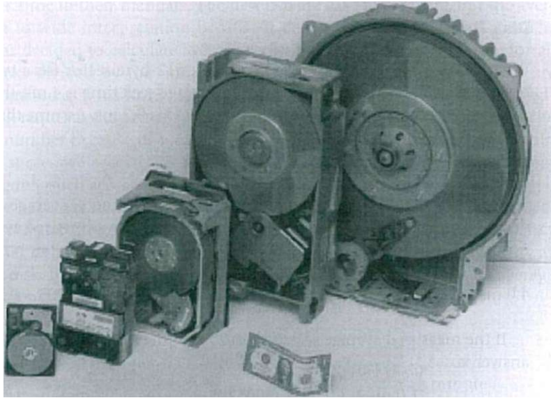
FIGURE 6.4 Six magnetic disks, varying in diameter from 14 inches down to 1.8 inches.
