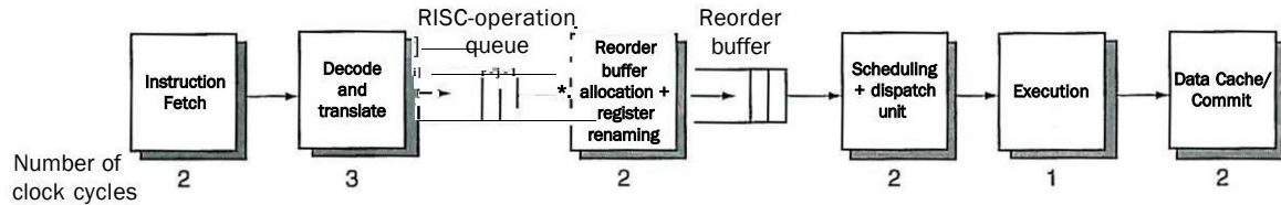
FIGURE 4.75 The Opteron X4 pipeline showing the pipeline flow for a typical instruction and the number of clock cycles for the major steps in the 12-stage pipeline for integer RISC-operations. The floating point execution queue is 17 stages long. The major buffers where RISC-operations wait are also shown.
