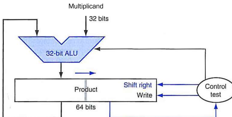
FIGURE 3.6 Refined version of the multiplication hardware. Compare with the first version in Figure 3.4. The Multiplicand register, ALU, and Multiplier register are all 32 bits wide, with only the Product register left at 64 bits. Now the product is shifted right. The separate Multiplier register also disappeared. The multiplier is placed instead in the right half of the Product register. These changes are highlighted in color. (The Product register should really be 65 bits to hold the carry out of the adder, but it's shown here as 64 bits to highlight the evolution from Figure 3.4.)
