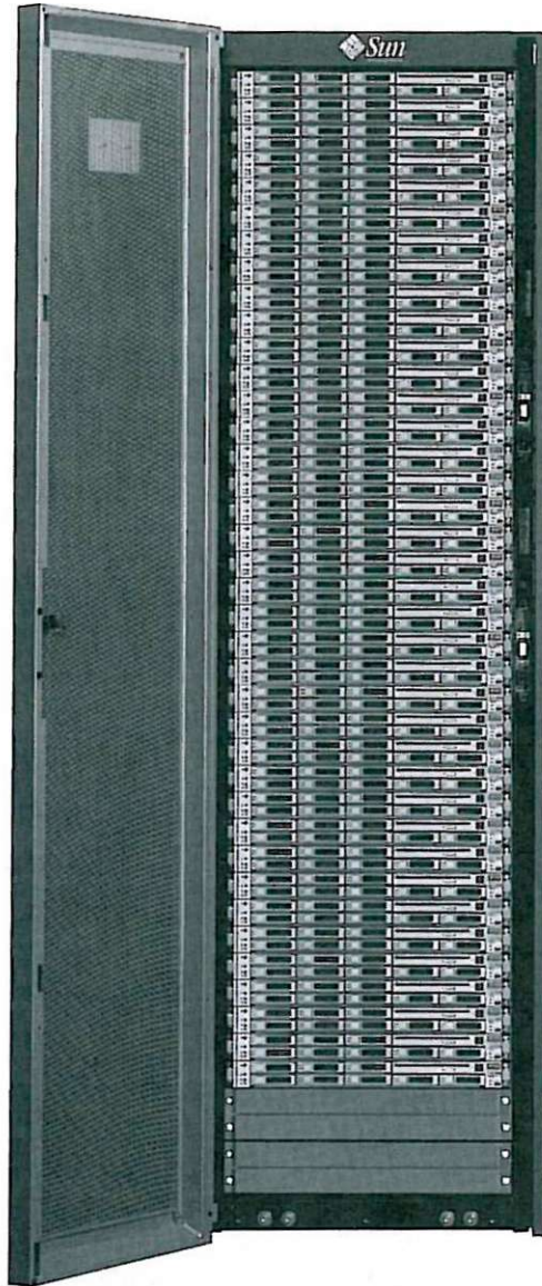
FIGURE 6.15 A standard 19-inch rack populated with 42 1U servers. This rack has 42 1U "pizza box" servers. Source: http://gchelpdesk.ualberta.ca/news/07mar06/cbhd_news_07mar06.pbp .
