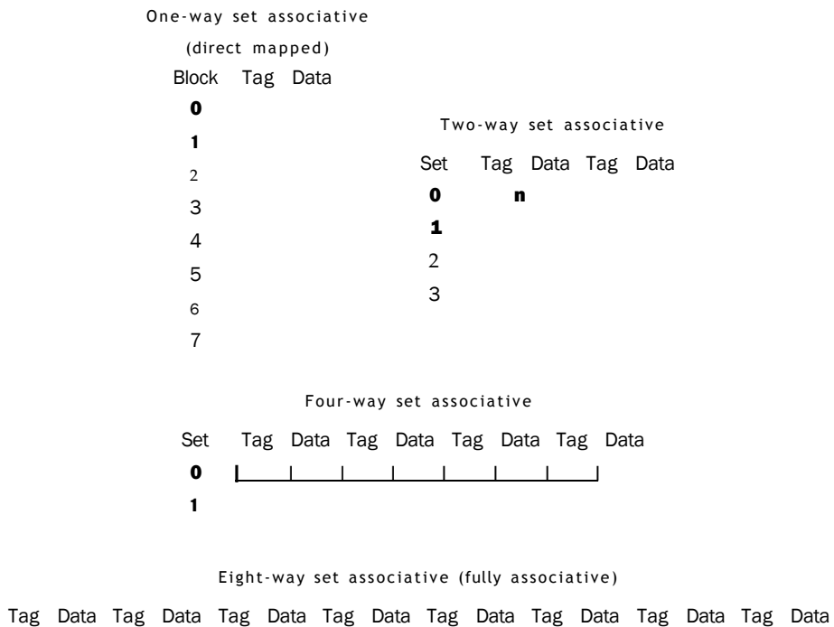
FIGURE 5.14 An eight-block cache configured as direct mapped, two-way set associative, four-way set associative, and fully associative. The total size of the cache in blocks is equal to the number of sets times the associativity. Thus, for a fixed cache size, increasing the associativity decreases the number of sets while increasing the number of elements per set. With eight blocks, an eight-way set-associative cache is the same as a fully associative cache.
