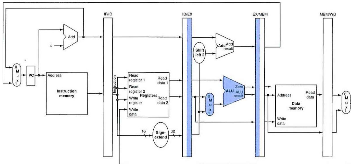
FIGURE 4.39 EX: The third pipe stage of a store instruction. Unlike the third stage of the load instruction in Figure 4.37, the second register value is loaded into the EX/MEM pipeline register to be used in the next stage. Although it wouldn't hurt to always write this second register into the EX/MEM pipeline register, we write the second register only on a store instruction to make the pipeline easier to understand.
