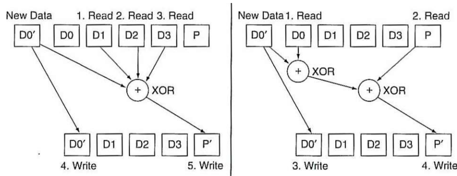
FIGURE 6.13 Small write update on RAID 3 versus RAID 4. This optimization for small writes reduces the number of disk accesses as well as the number of disks occupied. This figure assumes we have four blocks of data and one block of parity. The straightforward RAID 3 parity calculation in the left of the figure reads blocks D1, D2, and D3 before adding block D0' to calculate the new parity P'. (In case you were wondering, the new data D0' comes directly from the CPU, so disks are not involved in reading it.) The RAID 4 shortcut on the right reads the old value D0 and compares it to the new value D0' to see which bits will change. You then read the old parity P and then change the corresponding bits to form P'. The logical function exclusive OR does exactly what we want. This example replaces three disk reads (D1, D2, D3) and two disk writes (D0', P') involving all the disks for two disk reads (D0, P) and two disk writes (D0', P'), which involve just two disks. Increasing the size of the parity group increases the savings of the shortcut. RAID 5 uses the same shortcut.
