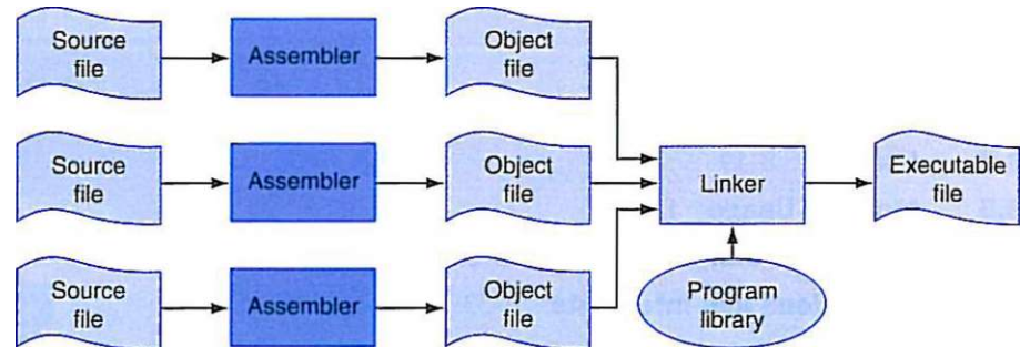
FIGURE B.1.1 The process that produces an executable file. An assembler translates a (file of assembly language into an object file, which is linked with other files and libraries into an executable file.
