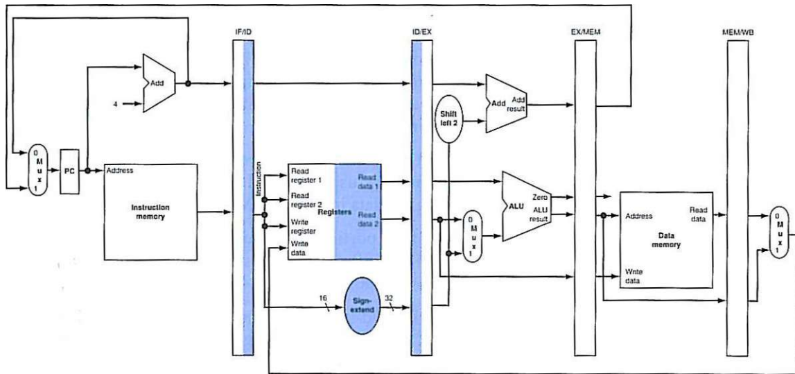
FIGURE 4.36 IF and ID: First and second pipe stages of an instruction, with the active portions of the datapath in Figure 4.35 highlighted. The highlighting convention is the same as that used in Figure 4.28. As in Section 4.2, there is no confusion when reading and writing registers, because the contents change only on the clock edge. Although the load needs only the top register in stage 2, the processor doesn't know what instruction is being decoded, so it sign-extends the 16-bit constant and reads both registers into the ID/EX pipeline register. We don't need all three operands, but it simplifies control to keep all three.
