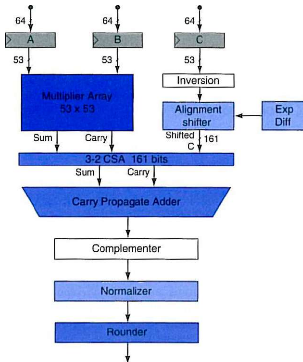
FIGURE A.6.2 Double precision fused-multiply-add (FMA) unit. Hardware To implement floating-point A \times B + C for double precision.
