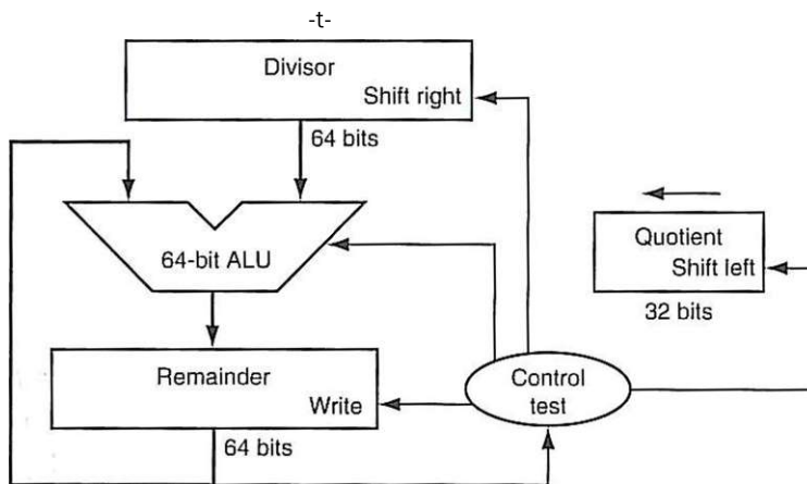
FIGURE 3.9 First version of the division hardware. The Divisor register, ALU, and Remainder register are all 64 bits wide, with only the Quotient register being 32 bits. The 32-bit divisor starts in the left half of the Divisor register and is shifted right 1 bit each iteration. The remainder is initialized with the dividend. Control decides when to shift the Divisor and Quotient registers and when to write the new value into the Remainder register.
