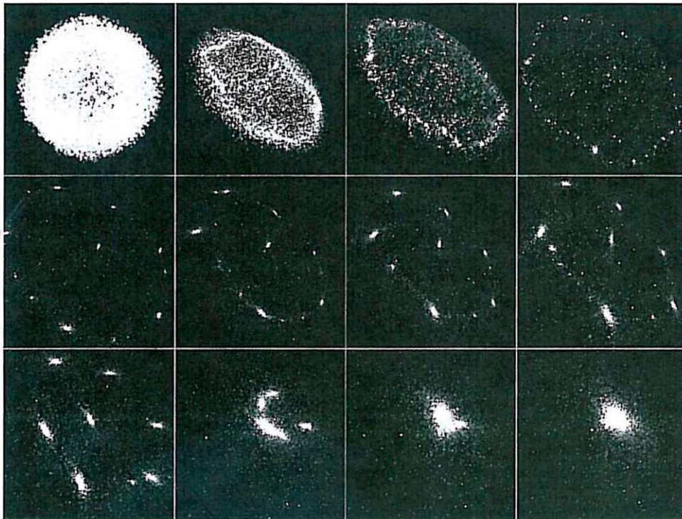
FIGURE A.8.17 12 images captured during the evolution of an N-body system with 16,384 bodies.
