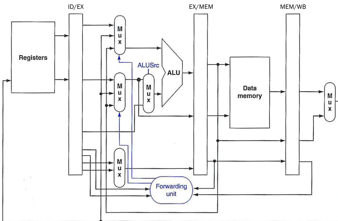
FIGURE 4.57 A close-up of the datapath in Figure 4.54 shows a 2:1 multiplexor, which has been added to select the signed immediate as an ALU input.
