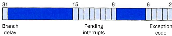
FIGURE B.7.2 The Cause register.
