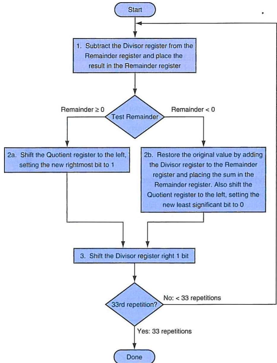
FIGURE 3.10 A division algorithm, using the hardware in Figure 3.9. If the remainder is positive, the divisor did go into the dividend, so step 2a generates a 1 in the quotient. A negative remainder after step 1 means that the divisor did not go into the dividend, so step 2b generates a 0 in the quotient and adds the divisor to the remainder, thereby reversing the subtraction of step 1. The final shift, in step 3, aligns the divisor properly, relative to the dividend for the next iteration. These steps are repeated 33 times.
