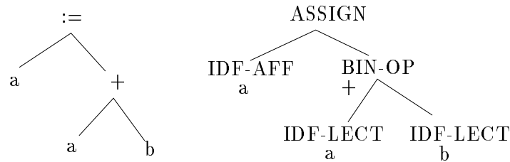
Figure 4.7: Parse tree of instruction "a:=a+b". On the left side: the parse tree is labeled with words of the Pascal program. On the right, the labels are made of two parts: the first part specifies the kind of the node, the second part is an attribute that stores the function of the node. For example, IDF-AFF indicates that the node contains the name of a variable that is modified, IDF-LECT: the name of a variable which is read, BIN-OP the name of a binary operator like the addition, ASSIGN indicates that we are doing an assignment, the left sub tree must contain the name of a variable to modify, the right sub tree contains the expression of the new value. For nodes IDF-AFF and IDF-LECT, the attribute contains the name of the variable to modify or to read. For BIN-OP, the attribute contains the name of the particular binary operator. The ASSIGN node does not have particular attributes.
