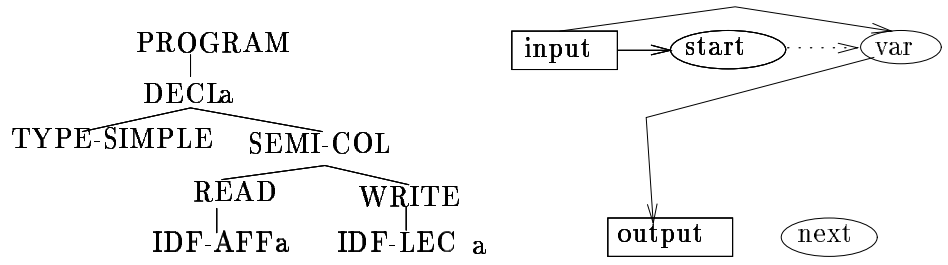
Figure C.10: The "next" cell unblocks, and disappears. Its deletion leads to the suppression of neuron 2. The final neural net encompass two input neurons: the start cell and the input variable "a"; and one output neuron: the variable "a". This neural net reads "a" and write "a". It translates what is specified by the Pascal program.
