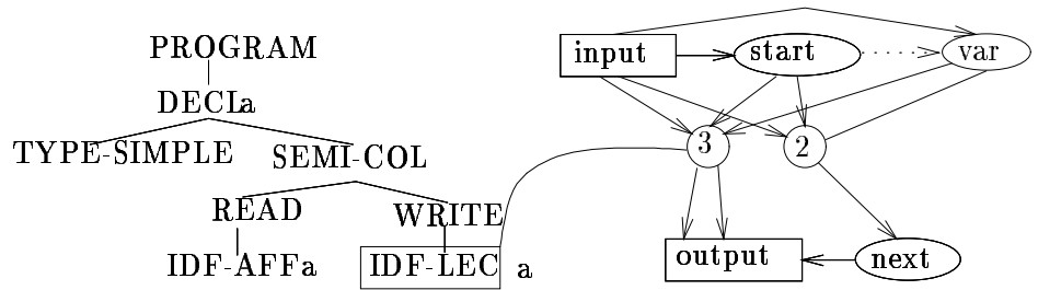
Figure C.8: Execution at step 8 of the macro program symbol WRITE. Cell 2 gives birth to another cell 3, connected to the output pointer cell. This cell 3 possesses all the input connections of cell 2. Cell 2 becomes a neuron.
