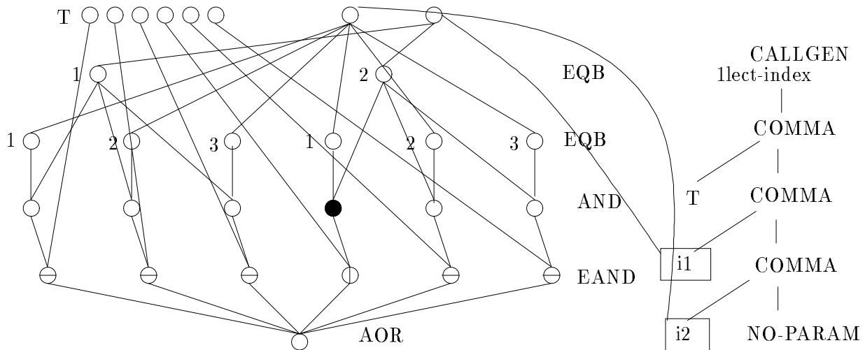
Figure C.29: Reading of a 2D array. The index i_1 is 2, the index i_2 is 1. The two first layers of EQBs have a sigmoid that test the equality to zero. They output 1 if the net input is 0, otherwise they output -1. These EQB neurons have different thresholds that are indicated. The third layer of neurons computes the logical ANDs. In this layer, a single neuron outputs 1, the one that corresponds to the element that must be read. All the other neurons of this layer output -1. The fourth layer of neurons is a layer of EAND neurons. only one of these neuron is activated. It propagates the element of the array that is read. Last, a neuron AOR gathers all the output lines and retrieves the element that is read. The instruction CALLGEN is almost like CALL-F, except that all the links to the global variables are deleted. CALLGEN will be described at the end of this section
