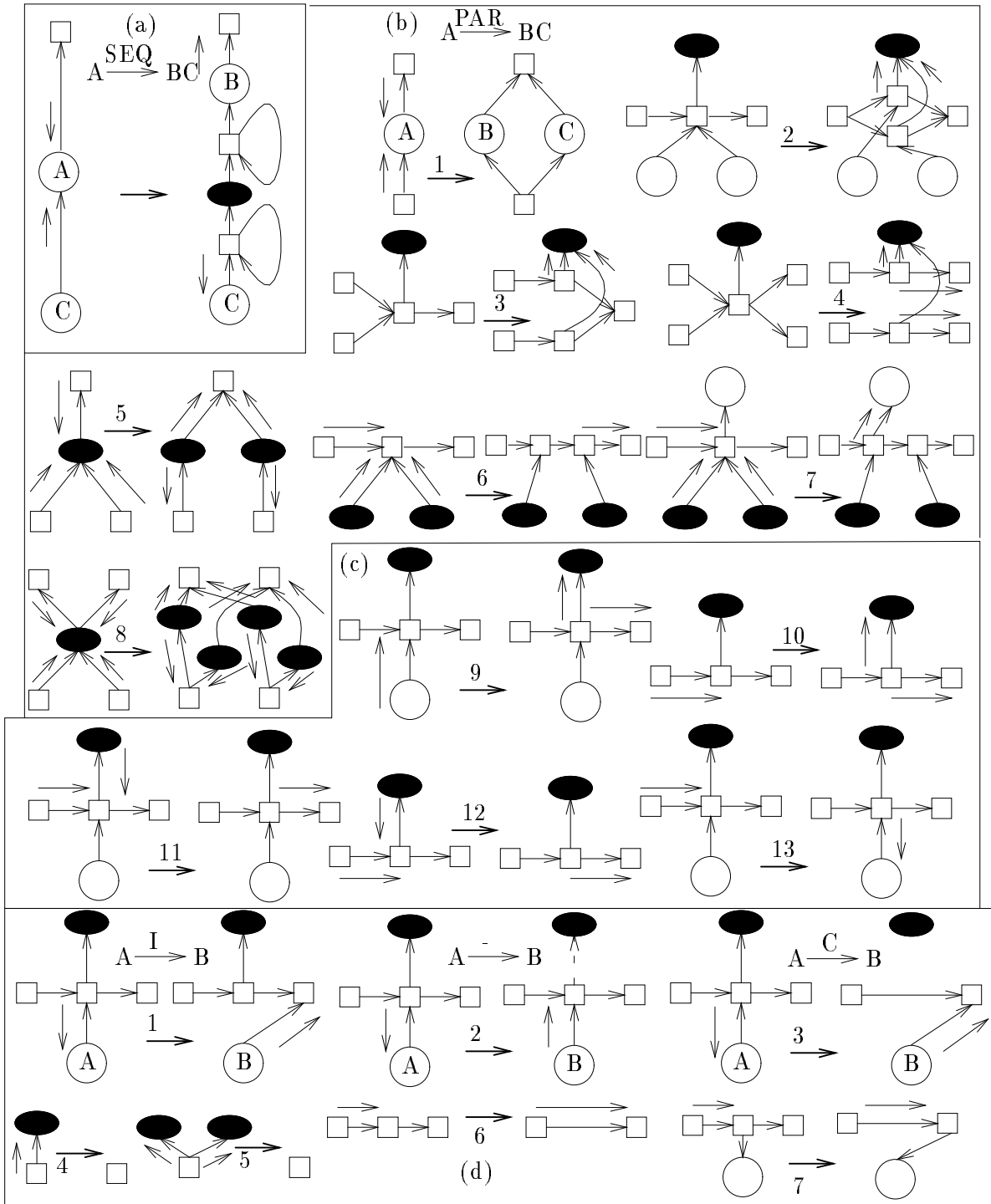
Figure B.4: Translation of the rule for cell division. (a) The sequential division (b) The parallel division (c) Managing the edge labels (arrows).
