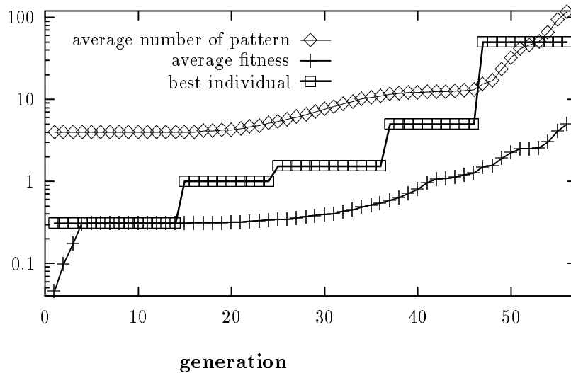
Figure 5.3: Plot of the average number of patterns used to evaluate the fitnesses, the average and best fitness in the current population.
