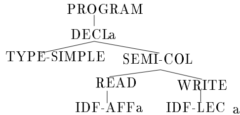
Figure 4.13: The parse tree of the Pascal Program: "program p; var a : integer; begin read(a); write (a); end." This parse tree does not have the usual form. It contains nodes for the declaration of variables, and the labels are not organized in a standard way. This particular form helps the implementation of the neural compiler. The appendix contains a BNF grammar that describes the form of these parse trees.
