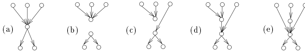
Figure 4.3: Microcoding of the program-symbol ADL 2. (Add on Link), 2 is an argument. This program symbol adds a cell on the link number 2. The microcode is \text{DIVm}\langle\text{sm}\rangle 2 (a) before the division ADL, (b) division in two children. (c) the segment "m" is analysed, (d) the segment "s" is analysed (e) the segment "m<" is analysed.
