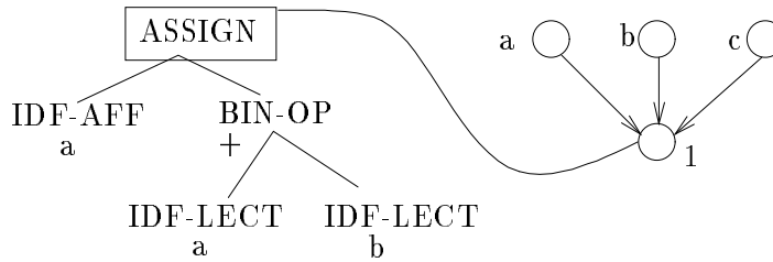
Figure 4.8: Development of the neural network corresponding to the Pascal instruction "a:=a+b", on the right side of this figure. The development begins with an ancestor cell labeled "1" connected to three neurons labeled "a", "b" and "c". On the left side, we represent the parse tree of the Pascal instruction. The arrow between the ancestor cell and the symbol ASSIGN of the parse tree represents the reading head of the ancestor cell. The input and output connections are ordered. It is the position of the arrow on the circle of the cell that codes the connection number. For example, the link to "b" has number 2.
