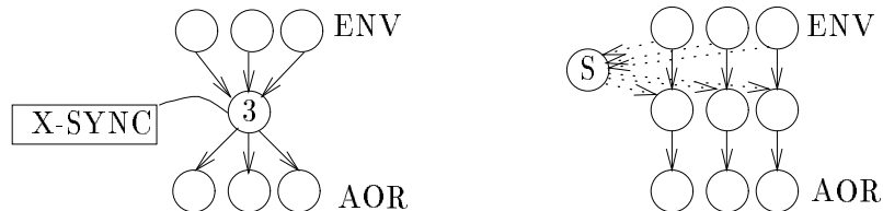
Figure C.16: Execution of the cellular code X-SYNC by cell 3 of the preceding figure. Cell 3 gives birth to a layer l of three neurons plus one neuron "S" whose dynamic is the normal dynamic. This layer is inserted between the layer of neuron that stores the output environment of the body of the WHILE , and the buffer layer of AOR at the beginning of the loop. The neuron "S" is connected from its input site, to all the neurons that contains the values of the environment. The neuron "S" is active only when all the environment is available. The neuron "S" is linked to the three neurons of layer l from its output site, with 0 weights. These connections are used to block the neurons while "S" is not active. So the three neurons of layer l are unblocked at the same time, and the flow of values is synchronized.
