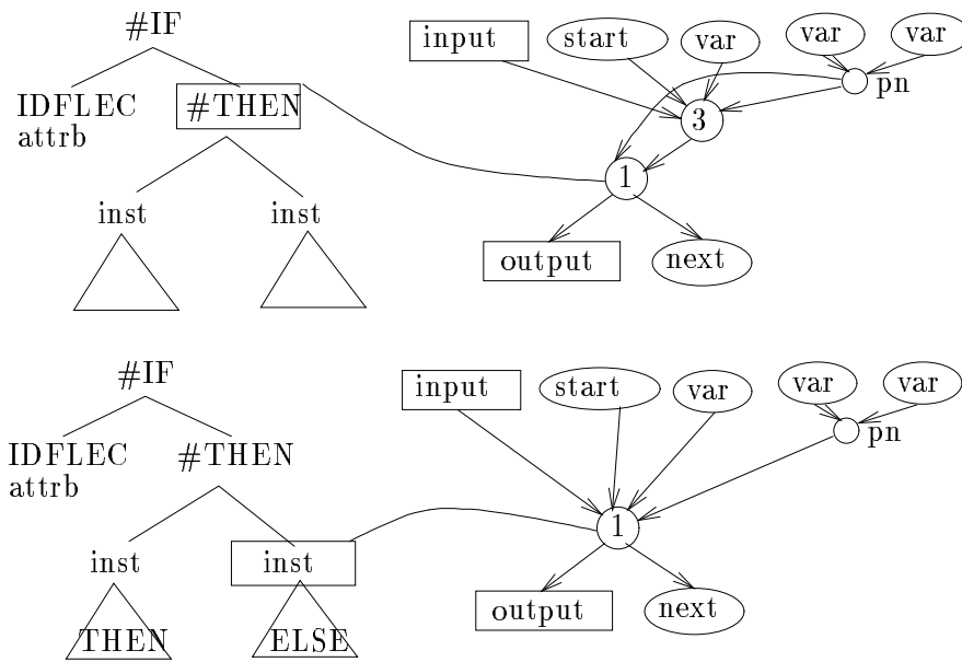
Figure C.33: Execution of the macro operator #THEN by cell number 1 of the preceding figure. After the execution of the macro program symbol IDF-LEC, cell 1 is unblocked and merges the links of its first input neighbor. The situation is described on top of the figure. The macro program symbol tests the number of input links of its first neighbor. Here this number is 2 because the array has two elements. If this number is greater than one, cell 1 places its reading head on the right subtree, as it is the case here. Otherwise it goes to read the left subtree. The left sub-tree contains the body of the #THEN, the right sub-tree contains the body of the #ELSE.
