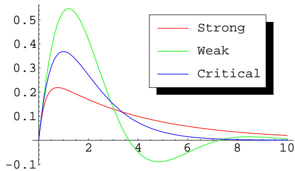
Figure 17.4: Strongly, weakly and critically damped solutions.
