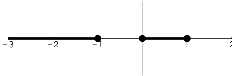
Figure 7.44: Branch cuts for \log\left(\frac{z(z+1)}{z-1}\right)
