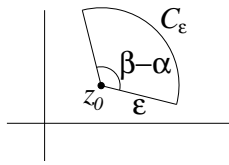
Figure 13.4: The C_\epsilon Contour
