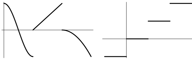
Figure 3.4: Piecewise Continuous Functions
