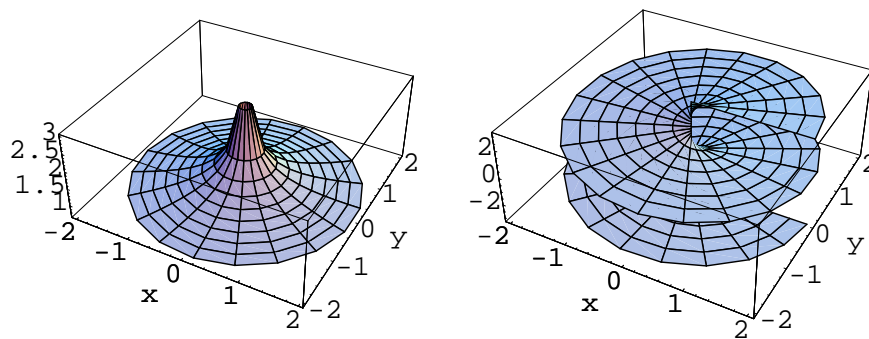
Figure 7.26: Plots of |\zeta^{-1/2}| and \text{Arg}(\zeta^{-1/2}) .
