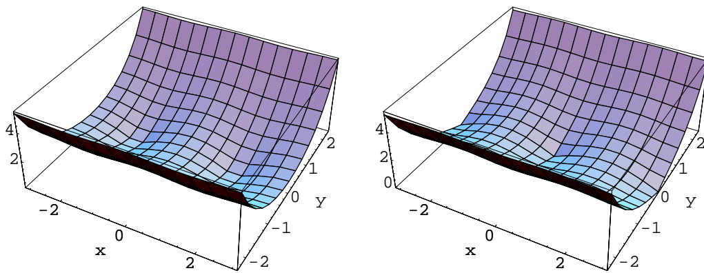
Figure 7.18: Plots of |\cos(z)| and |\sin(z)|
