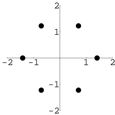
Figure 6.16: 8^{1/6}
