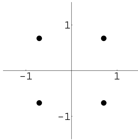
Figure 6.15: (-1)^{-3/4}
