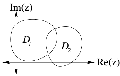
Figure 9.1: Overlapping Domains
