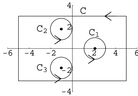
Figure 11.4: The contours for \frac{z}{z^3-9} .
