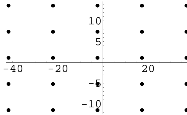
Figure 7.42: \log((1+i)^{z\pi})
