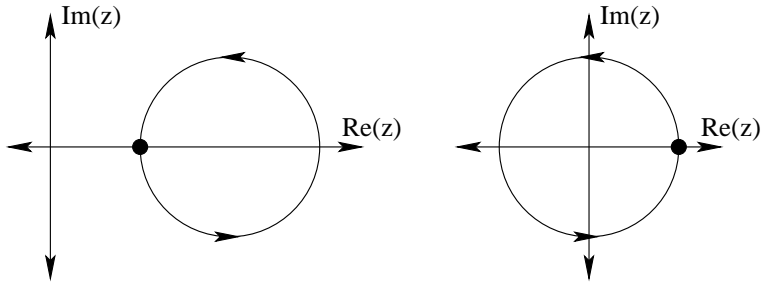
Figure 7.24: A path that does not encircle the origin and a path around the origin
