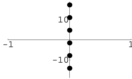
Figure 7.34: \log(-i)
