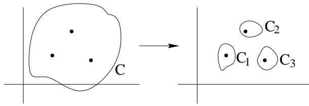
Figure 13.2: Deform the contour n contours which enclose the n singularities.
