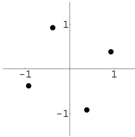
Figure 6.10: i^{1/4}
