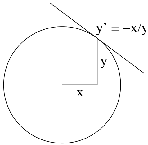
Figure 14.3: A circle and its tangent.
