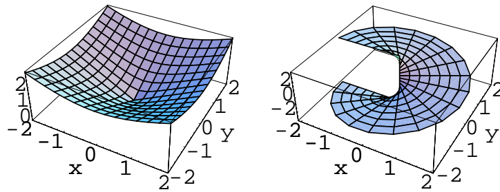
Figure 7.9: Plots of |z| and \text{Arg}(z)
