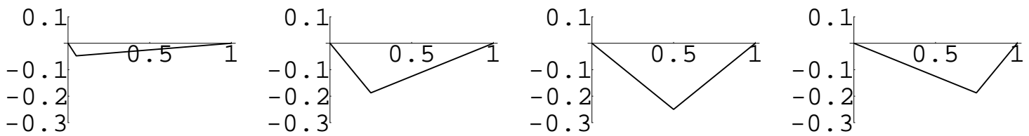
Figure 21.3: Plot of G(x|0.05), G(x|0.25), G(x|0.5) and G(x|0.75) .
