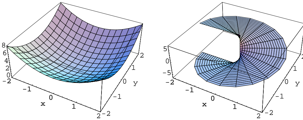
Figure 7.11: Plots of |z^2| and a branch of \arg(z^2)
