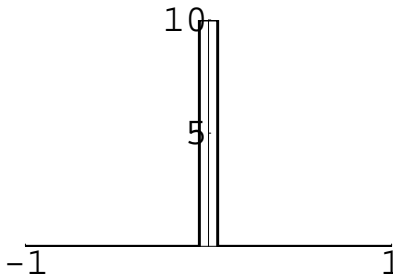
Figure 20.2: Graph of b(x, 1/10) .
