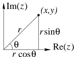
Figure 6.5: Polar Form
