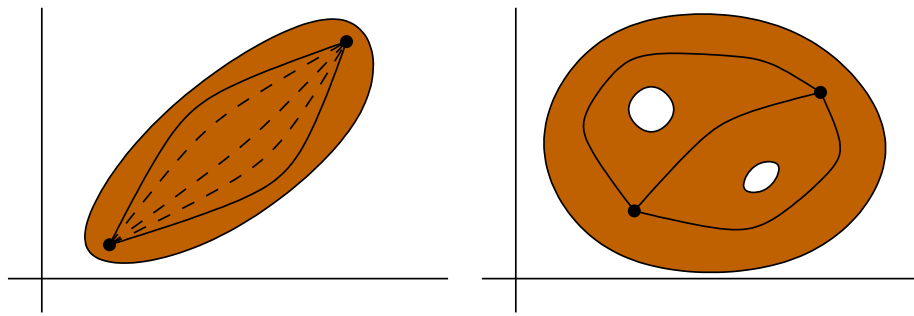
Figure 7.2: Simply-connected and multiply-connected regions.
