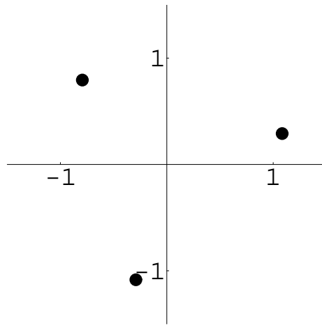
Figure 6.9: (1 + i)^{1/3}
