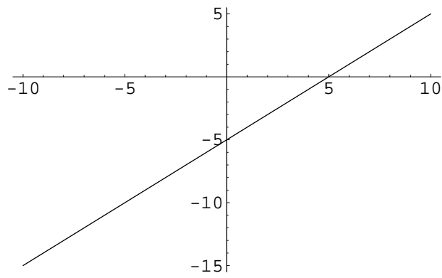
Figure 6.23: \Re(z) - \Im(z) = 5
