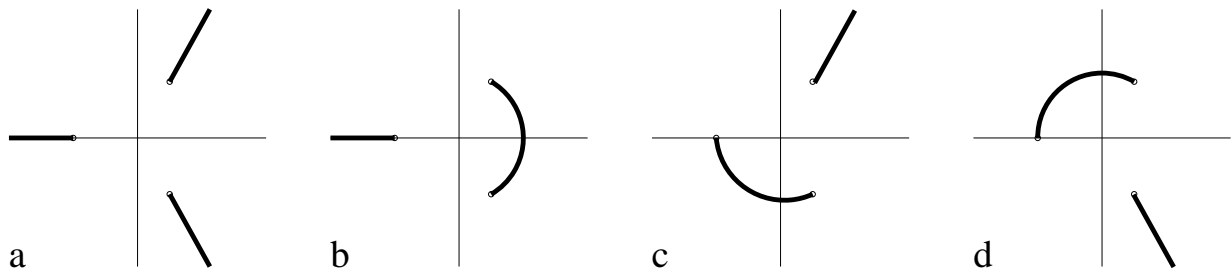
Figure 7.51: (z^3 + 8)^{1/2}
