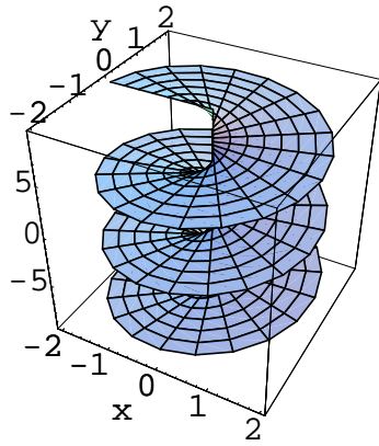
Figure 7.8: A Few Branches of \arg(z)
