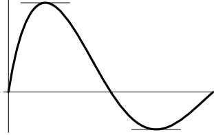
Figure 3.9: Rolle's Theorem.
