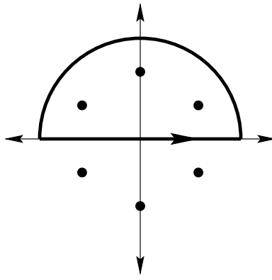
Figure 13.14: The semi-circle contour.
