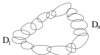
Figure 9.2: Two Paths of Analytic Continuation
