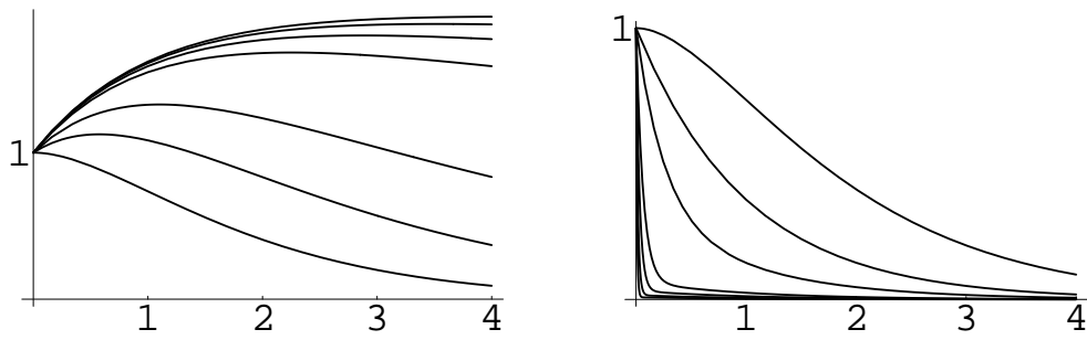
Figure 14.10: The Solution as \alpha \rightarrow 0 and \alpha \rightarrow \infty
