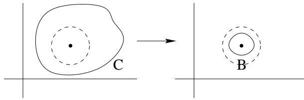
Figure 13.1: Deform the contour to lie in the deleted disk.
