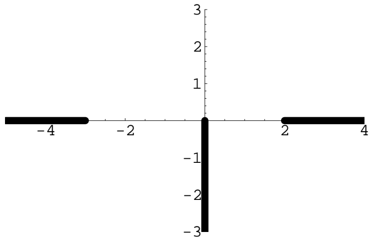
Figure 7.45: Branch Cuts for (z^3 + z^2 - 6z)^{1/2}
