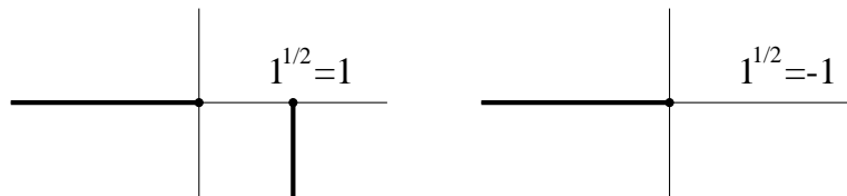
Figure 7.56: Branch Cuts for (z^{1/2} - 1)^{1/2}
