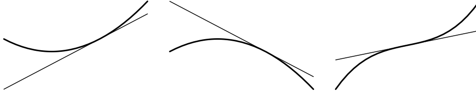
Figure 3.8: Concave Upward, Concave Downward and an Inflection Point.
