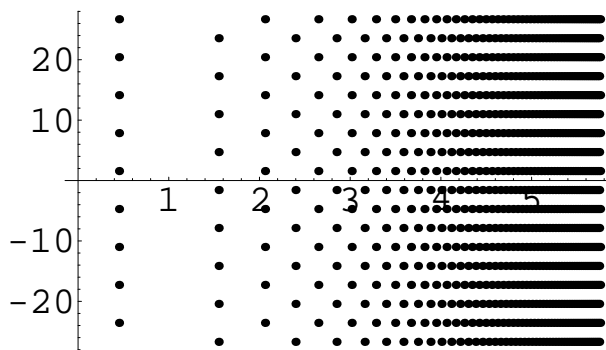
Figure 7.37: \log(\log(i))
