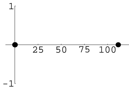
Figure 7.41: i^z
