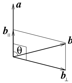
Figure 2.14: The vector \mathbf{b} written as a sum of components orthogonal and parallel to \mathbf{a} .
