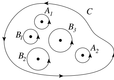
Figure 11.1: Deforming the contour C .
