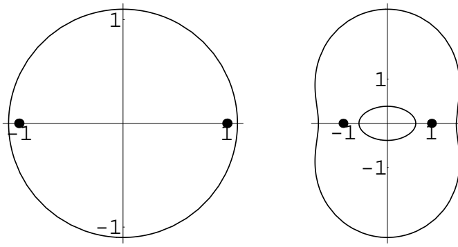
Figure 7.43: The mapping of a circle under w = z + (z^2 - 1)^{1/2} .
