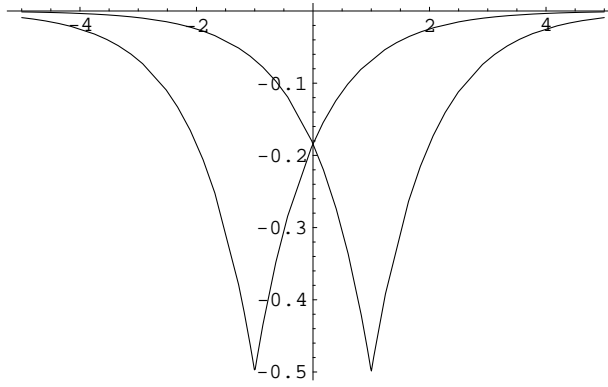
Figure 21.7: G(x; 1) and G(x; -1)
