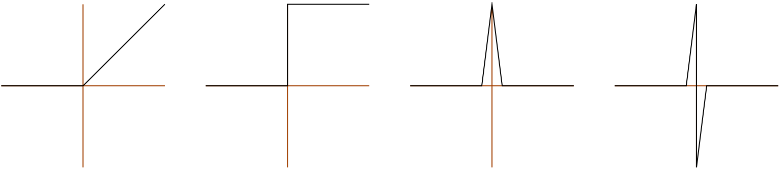
Figure 21.2: r(x) , H(x) , \delta(x) and \frac{d}{dx}\delta(x)
