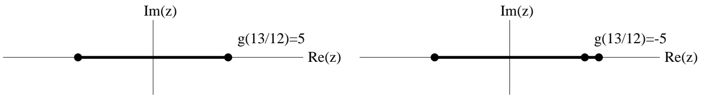
Figure 7.52: The branch cuts for f(z) = \log\left(5 + \left(\frac{z+1}{z-1}\right)^{1/2}\right) .
