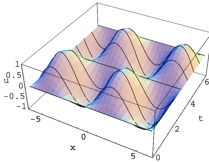
Figure 41.4: Solution of the wave equation.
