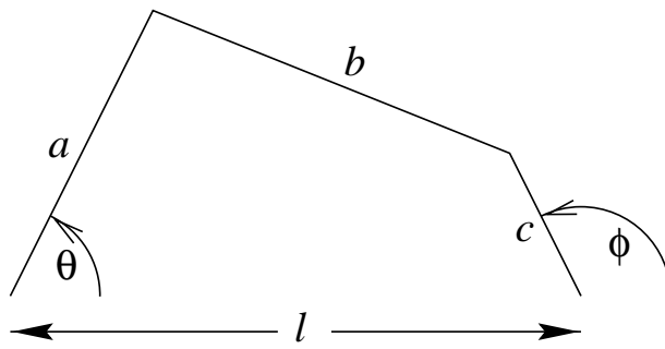
Figure 7.32: A linkage
