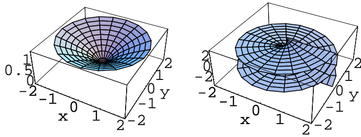
Figure 7.23: Plots of |z^{1/2}| and \text{Arg}(z^{1/2}) .
