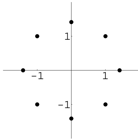
Figure 6.18: 16^{-1/8}
