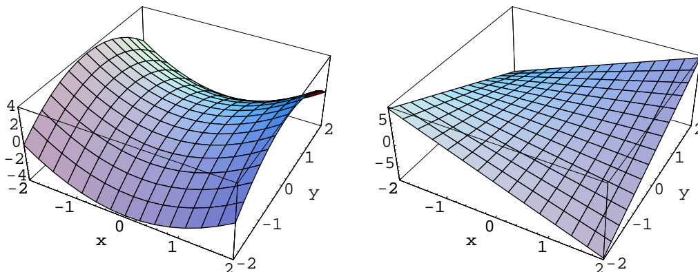
Figure 7.10: Plots of \Re(z^2) and \Im(z^2)
