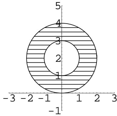
Figure 6.18: 16^{-1/8}
