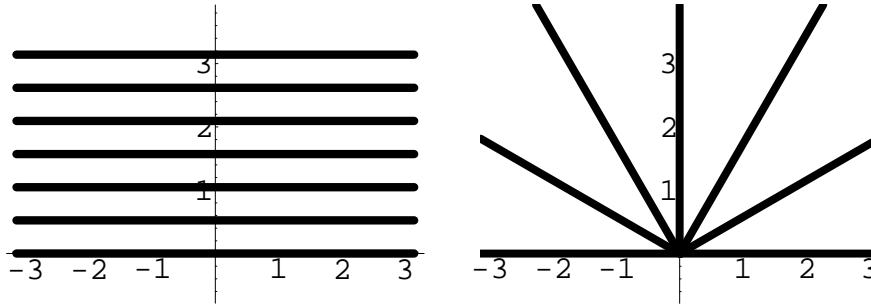
Figure 7.14: e^z maps horizontal lines to rays.
