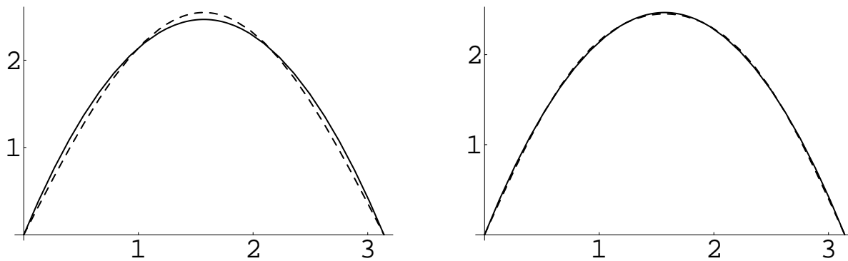
Figure 25.2: Series Expansions of x(\pi - x) .
