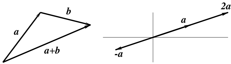
Figure 2.2: Vector arithmetic.
