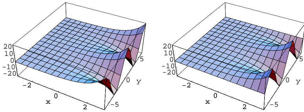
Figure 7.12: Plots of \Re(e^z) and \Im(e^z)
