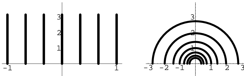
Figure 7.15: e^z maps vertical lines to circular arcs.
