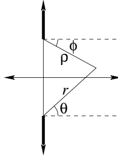
Figure 7.28: Branch Cuts for f(z) = (z^2 + 1)^{1/3}
