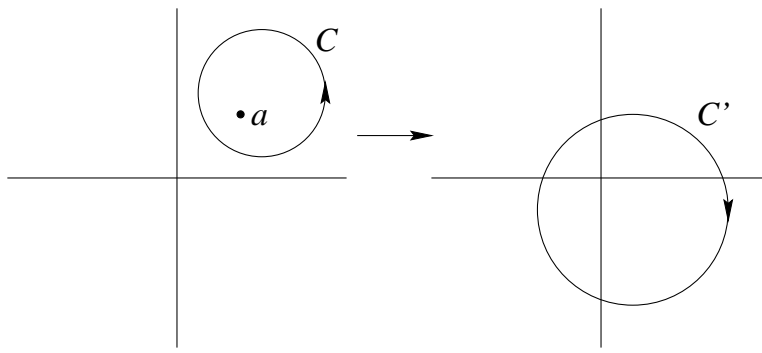
Figure 13.3: The change of variables \zeta = 1/(z - a) .
