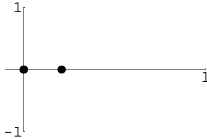
Figure 7.35: (-i)^{-i}
