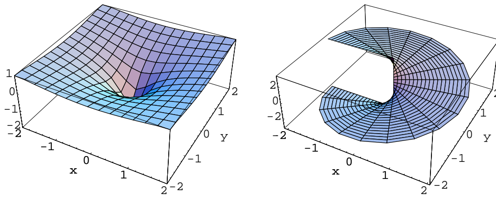
Figure 7.19: Plots of \Re(\text{Log } z) and \Im(\text{Log } z) .
