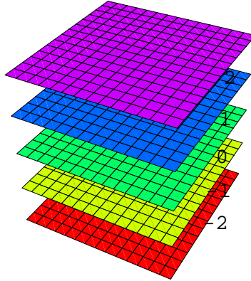
Figure 7.20: The z -plane decomposed into flat sheets.
