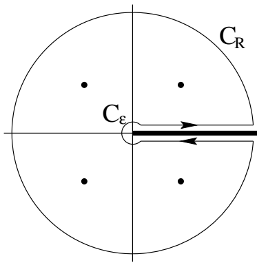
Figure 13.12: Possible path of integration for f(z) = \frac{z^a}{1+z^4}
