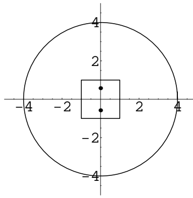
Figure 11.2: The contours and the singularities of \frac{1}{3z^2+1} .
