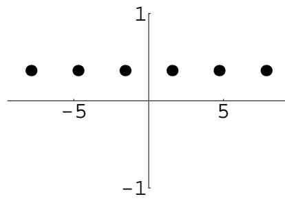
Figure 7.40: The values of \arctan(i3) .
