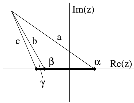
Figure 7.53: A branch of ((z^2 - 2)(z + 2))^{1/3} .
