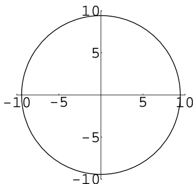
Figure 7.36: 3^\pi
