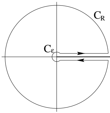
Figure 13.10: The path of integration.
