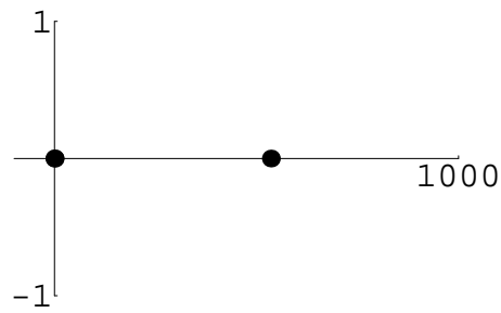
Figure 7.38: The values of (\cosh(i\pi))^{i^2} .
