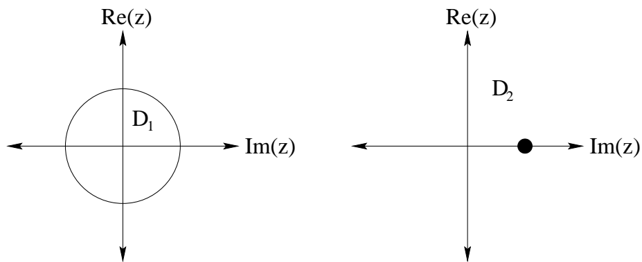
Figure 9.5: Domain of Convergence for \sum_{n=0}^{\infty} z^n .
