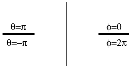
Figure 7.55: Branch Cuts and Angles for (z^2 - 1)^{1/2}
