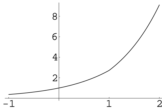
Figure 14.5: Solution to y' - y = H(x - 1) .
