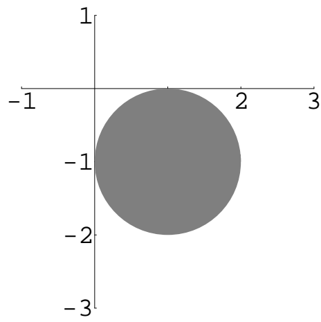
Figure 6.22: |z - 1 + i| < 1
