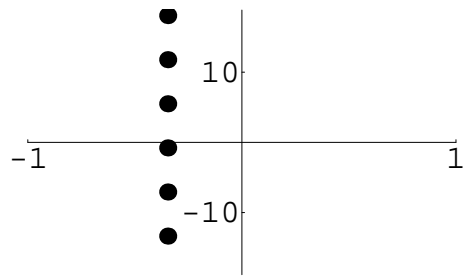
Figure 7.39: The values of \log\left(\frac{1}{1+i}\right) .
