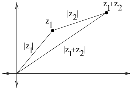
Figure 6.14: Triangle Inequality
