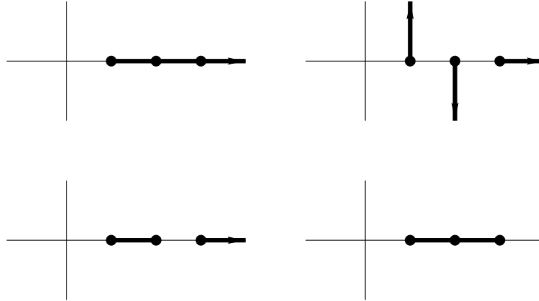
Figure 7.31: Four Candidate Sets of Branch Cuts for ((z - 1)(z - 2)(z - 3))^{1/2}
