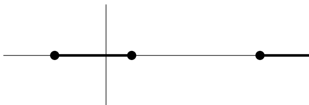
Figure 7.50: Branch Cuts for ((z + 2)(z - 1)(z - 6))^{1/2}
