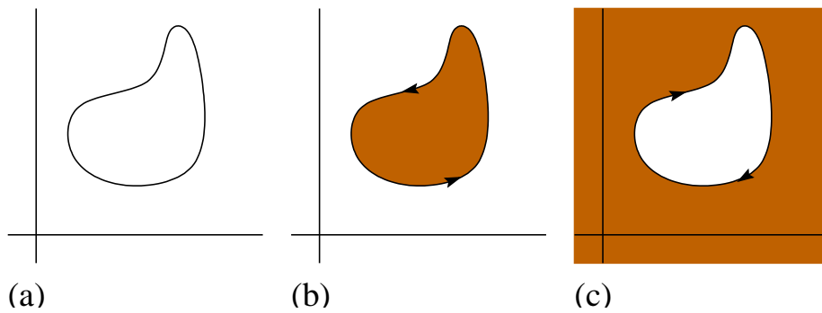
Figure 7.4: Two interpretations of a curve.
