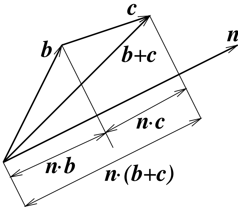
Figure 2.12: The distributive law for the dot product.
