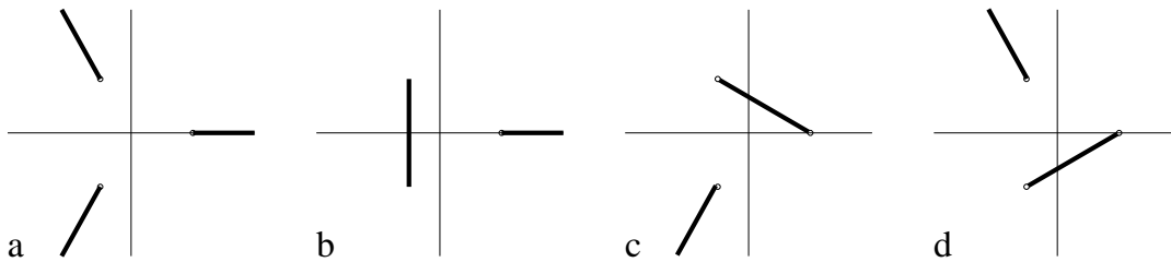
Figure 7.49: (z^3 - 1)^{1/2}
