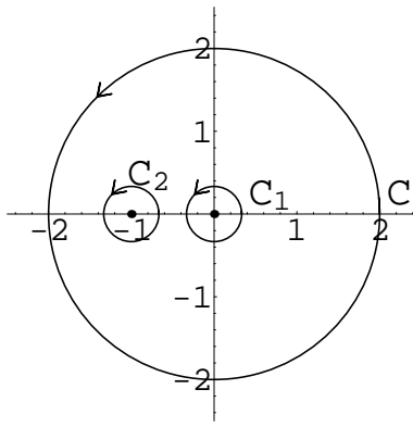
Figure 11.6: The contours for \frac{e^{zt}}{z^2(z+1)} .
