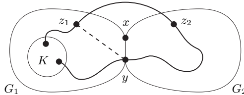
Fig. 4.4.4. A TK^5 or TK_{3,3} in G + z_1z_2
