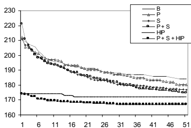
(a) best individual
