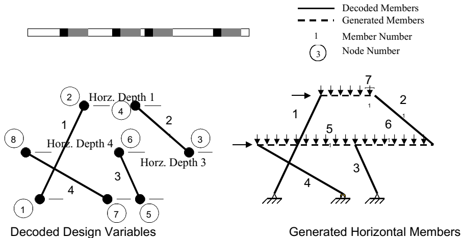
Figure 9.10 Assembly of complete structure from design variables
