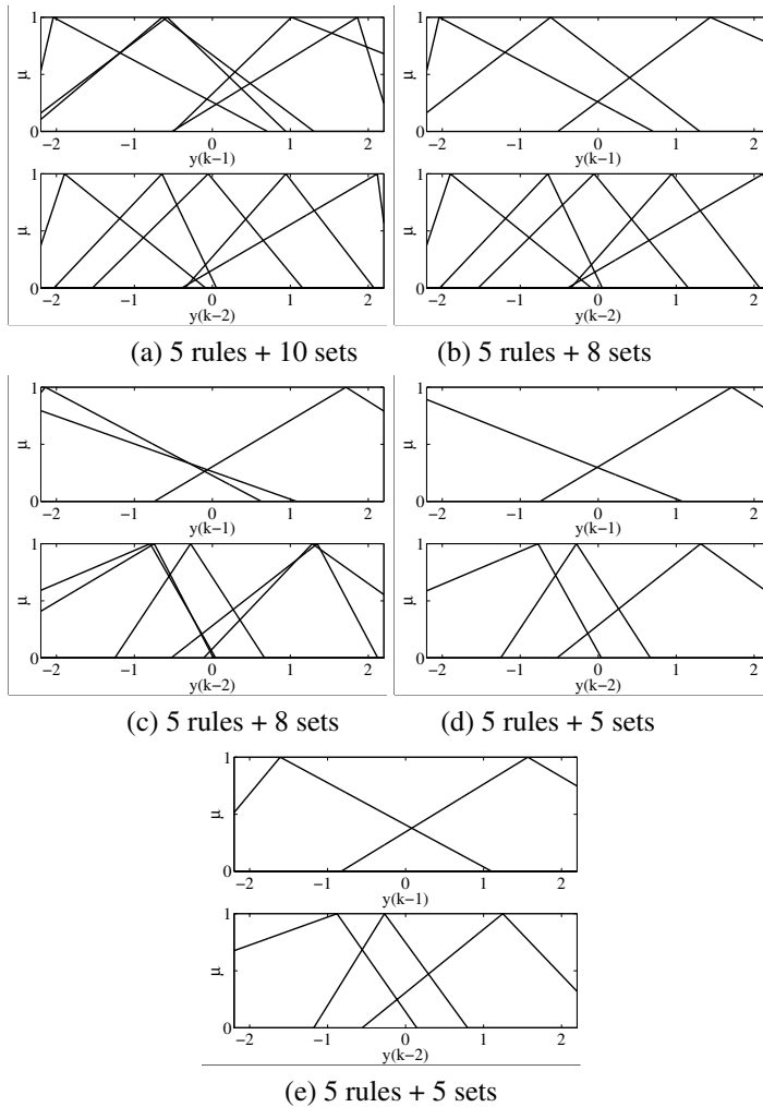
Figure 1.10 Local linear TS-model derived in five steps: (a) initial model with ten clusters, (b) set merging, (c) GA-optimization, (d) set-merging, (e) final GA optimization
