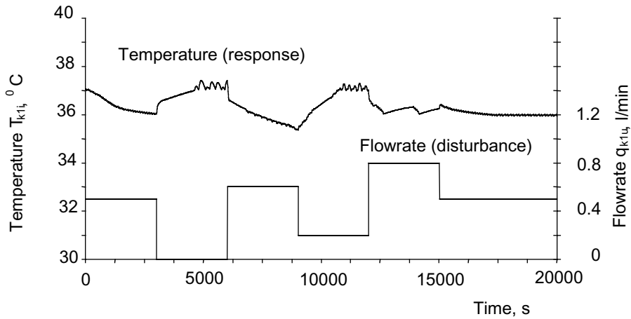
Figure 12.16 Response of the first stage of a plant controlled by fuzzy controllers (decision tables are GA-tuned) for set point T_r = 37^\circ\text{C}
