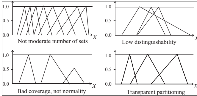
Figure 1.3 Transparency of the fuzzy rule base premise
