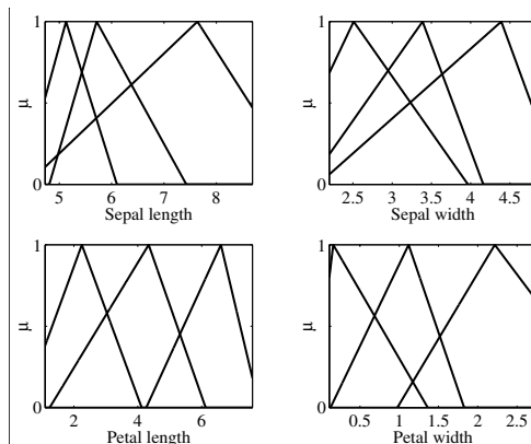
Figure 1.15 Optimized fuzzy rule-based model with three rules and three misclassifications (Table 1.3-B)
