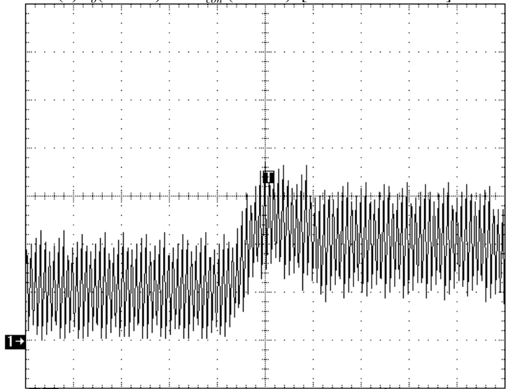
(b) i_L (0.5A/div). [Timebase: 2ms/div]
