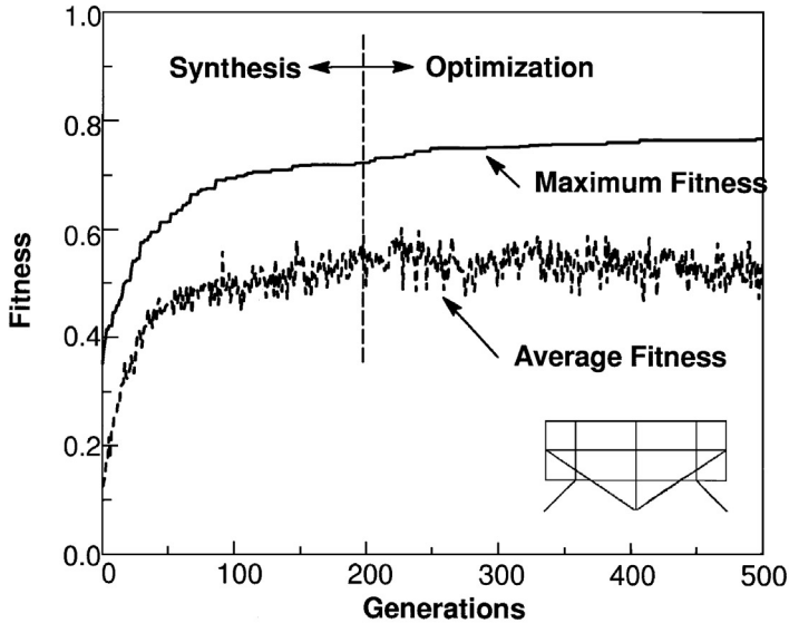
Figure 9.34 Maximum fitness and average fitness of the IRR GA population over 500 generations for a single trial.
