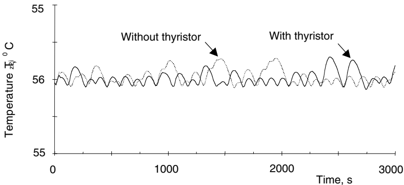
Figure 12.21 Second stage response with nonlinear characteristic of thyristor converter
