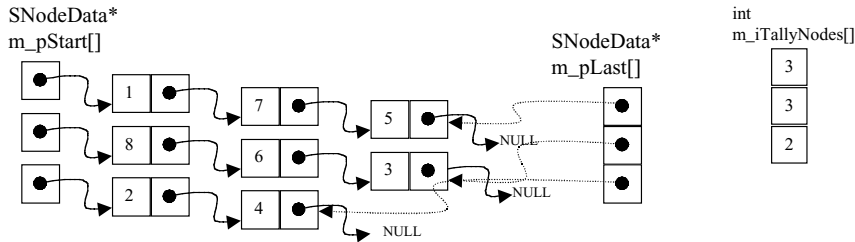
Figure 9.11 Linked lists of SNodeData structures for frame structure defined in Figure 9.10
