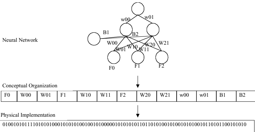
Figure 5.3 Organization of a chromosome coding for a simple three-layer neural network
