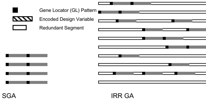
Figure 9.4 Dynamic redundancy provided by the IRR GA compared to the SGA
