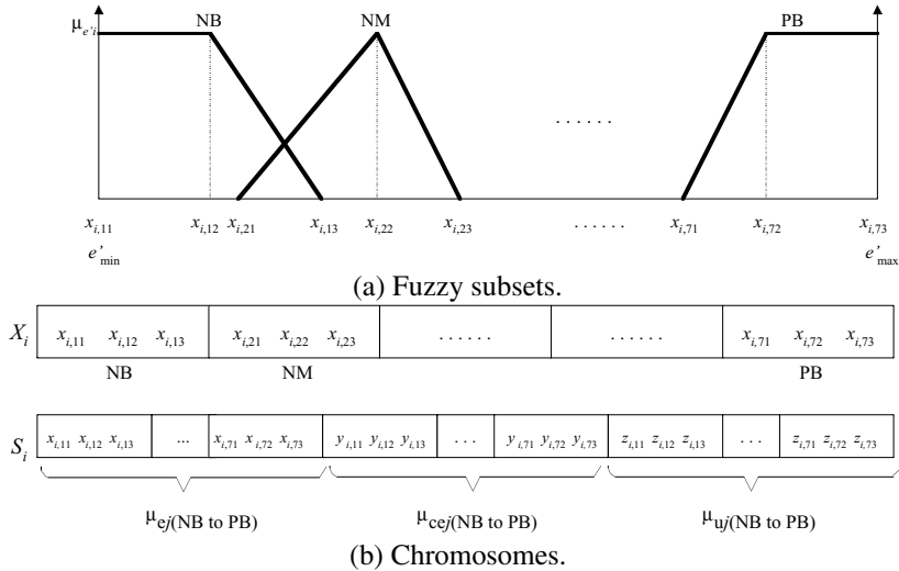
Figure 11.3 Structure of the fuzzy subsets and chromosomes
