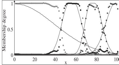
Figure 1.2 Fuzzy sets are defined by fitting parametric functions (solid lines) to the projections (dots) of the point-wise defined fuzzy sets in the fuzzy partition matrix U
