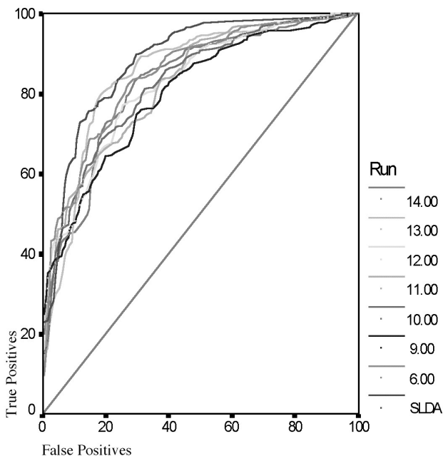
Figure 5.13 ROC curves for test on train results
