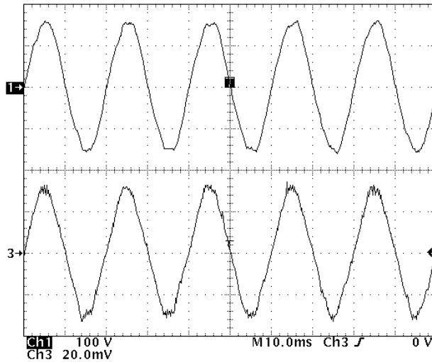
(a) Input voltage and input current waveforms.
