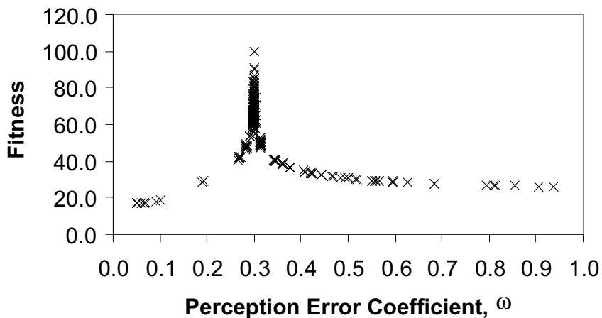
Figure 7.16 Fitness vs perception error coefficient in the TFS calibration
