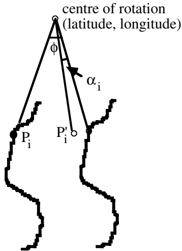
Figure 0.3 Fitting contours on the opposite sides of an ocean
