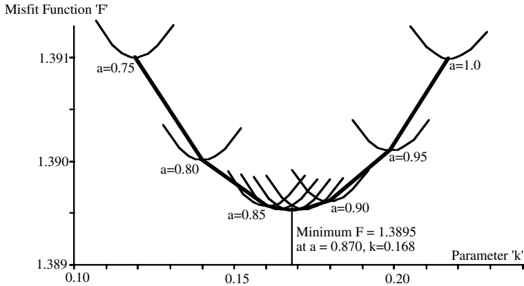
Figure 0.13 Fitting model 2: \rho(r) = a \cdot \exp(-kr)
