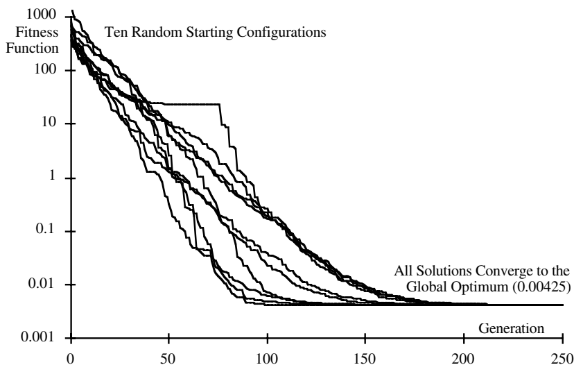
Figure 6.6 Genetic algorithm using the same ten random starting configurations
