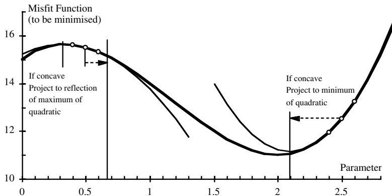
Figure 6.3 Projected mutation
