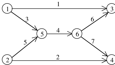
Figure 7.3 Example network 2
