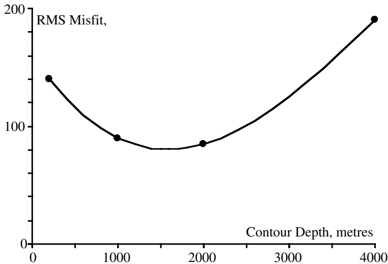
Figure 0.4 Least misfit for contours of steepest part of continental shelf
