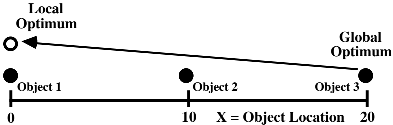
Figure 6.1 Global and local optima for the one-dimensional example
