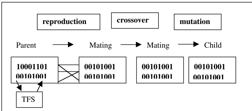
Figure 7.5 Flowchart of GAB calibration algorithm
