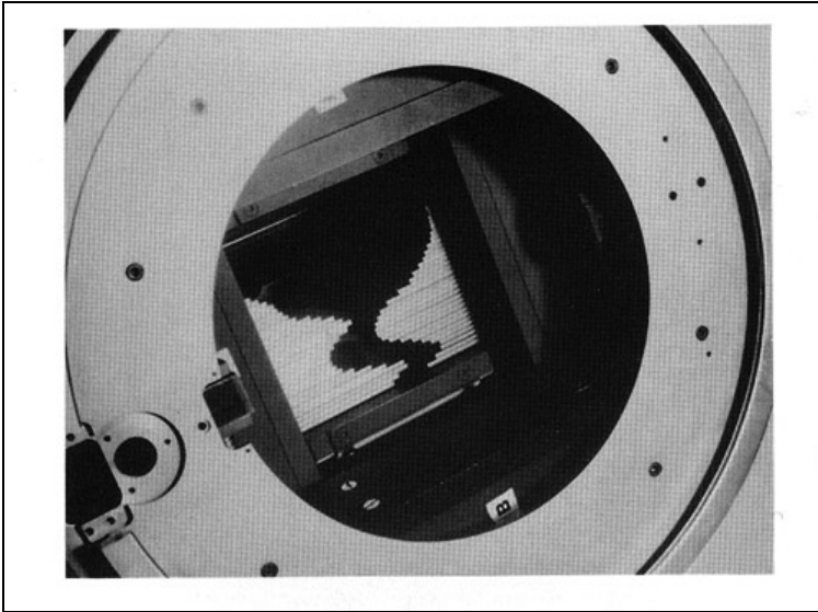
Figure 13.2 The Elekta multi-leaf collimator
