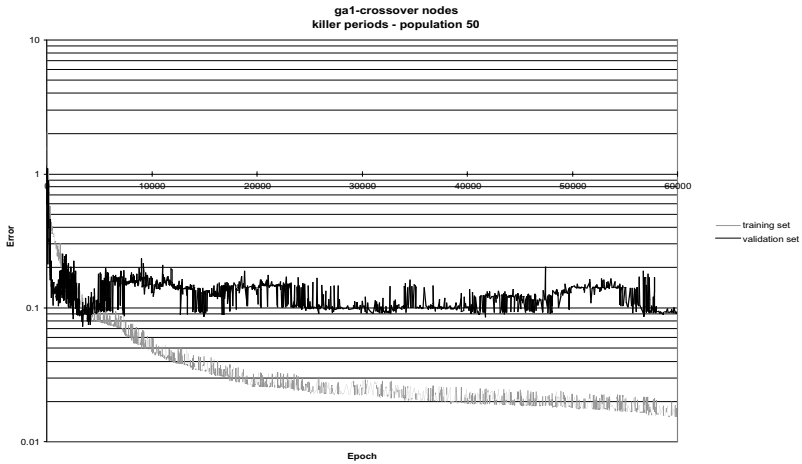
Figure 13.11 A plot of training set error and validation set error against generation for the EANN
