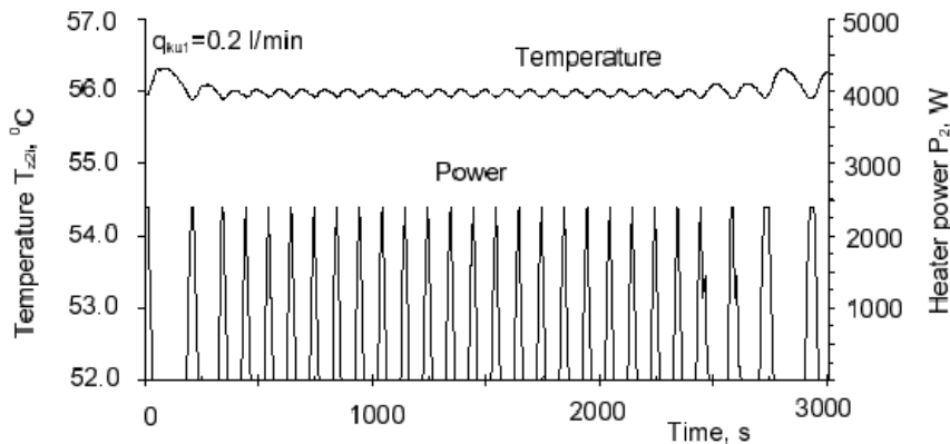
Figure 12.13 Second stage response to step disturbance q_{klu} (from q_{klu} = 0.5 l/min to q_{klu} = 0.2 l/min) controlled with genetic algorithm-tuned decision tables
