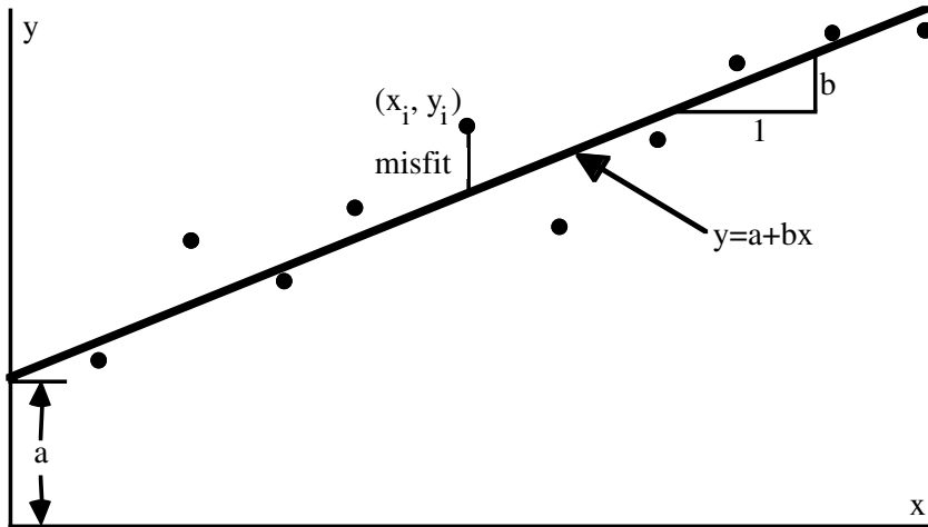
Figure 0.1 Simple linear regression
