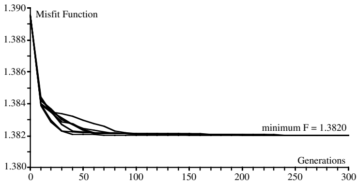
Figure 0.16 Fit of model 3 using the genetic algorithm
