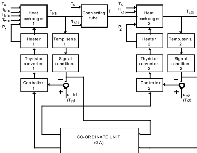
Figure 12.4 Block diagram of laboratory plant
