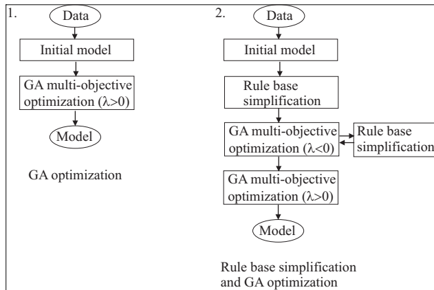
Figure 1.5 Two modeling schemes with multi-objective GA optimization
