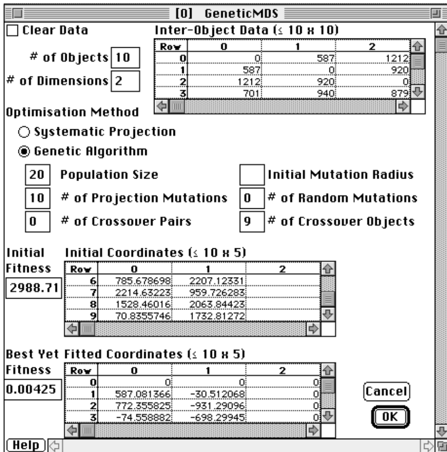
Figure 6.4 The genetic algorithm control panel
