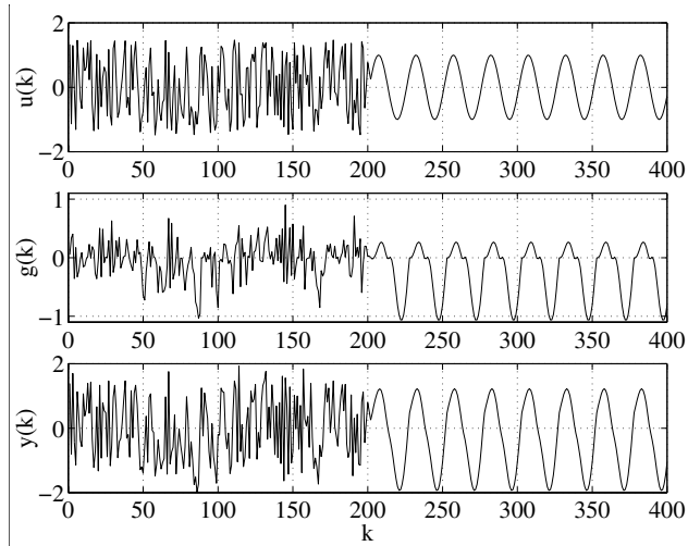
Figure 1.6 Input u(k) , unforced system g(k) , and output y(k) of the plant in (Equations 15 and 16)
