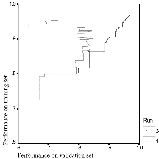
Figure 5.7 Performance of a “good” classifier (Run 1) compared with that of a “poor” classifier (Run 3) on training and validation data
