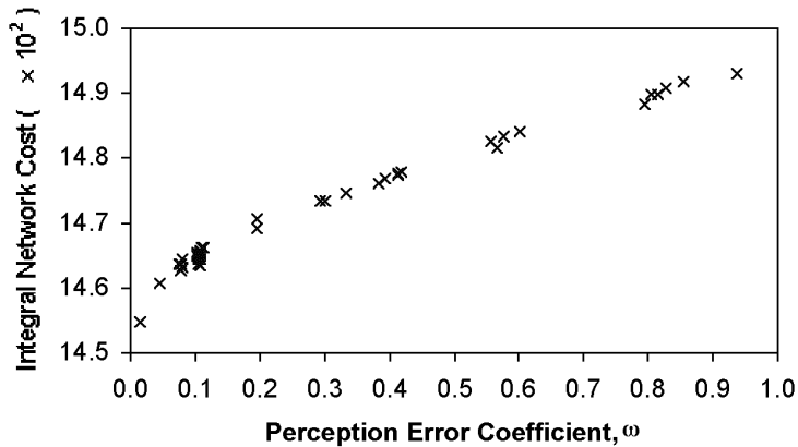
Figure 7.7 Integral network cost vs. perception error coefficient
