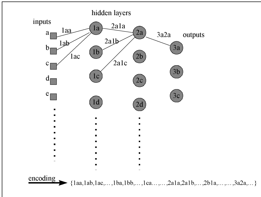
Figure 13.10 Encoding of the connection weights on a chromosome
