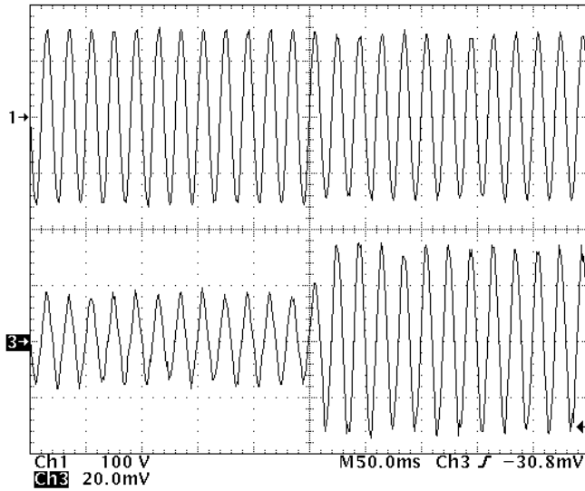
(a) Input voltage and input current waveforms.
