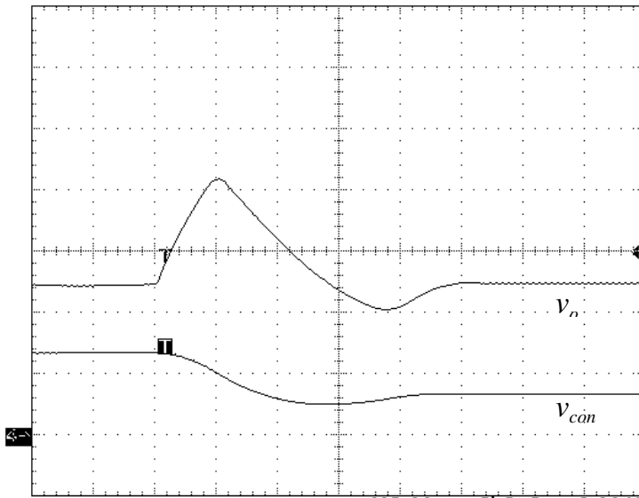
(a) v_o (2V/div) and v_{con} (2V/div) [Timebase: 2ms/div]
