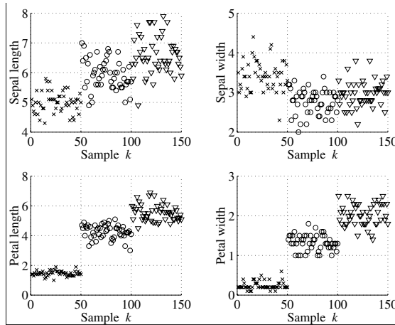
Figure 1.13 Iris data: setosa (×), versicolor (O), and virginica (∇)
