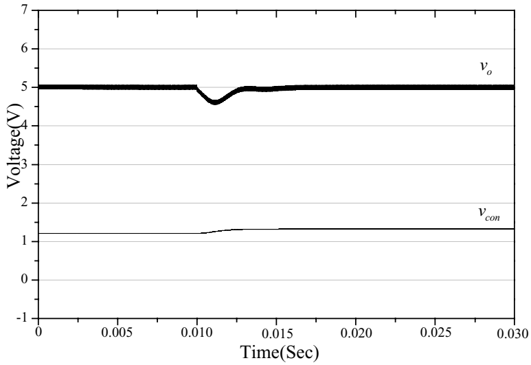
(a) v_o and v_{con}
