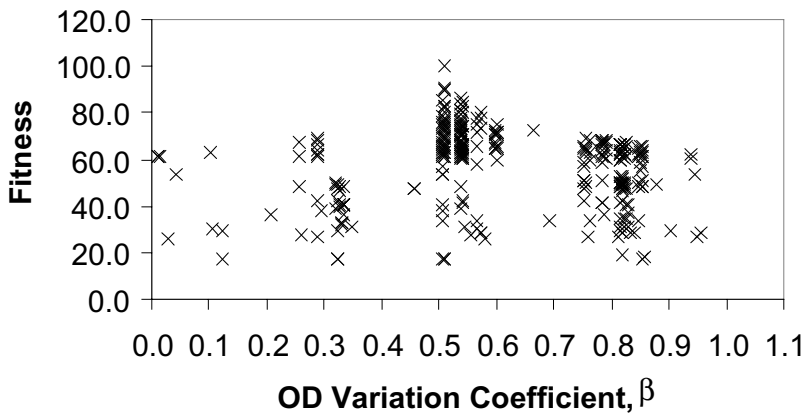
Figure 7.17 Fitness vs OD variation coefficient in the TFS calibration
