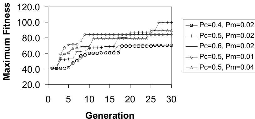
Figure 7.15 Maximum fitness vs. crossover probability and mutation probability
