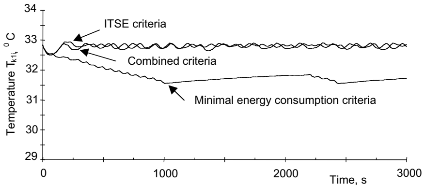
Figure 12.22 First stage process response for various optimizing criteria
