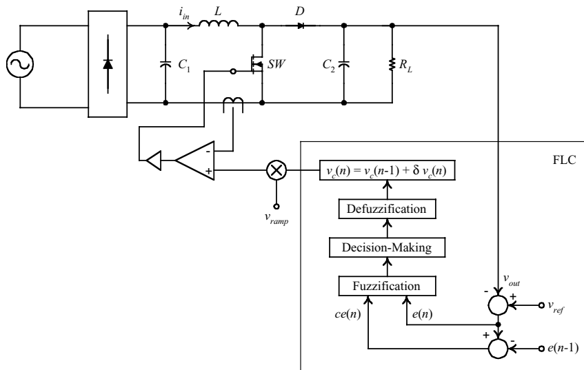
Figure 11.1 Block diagram of the boost rectifier with APFC and FLC
