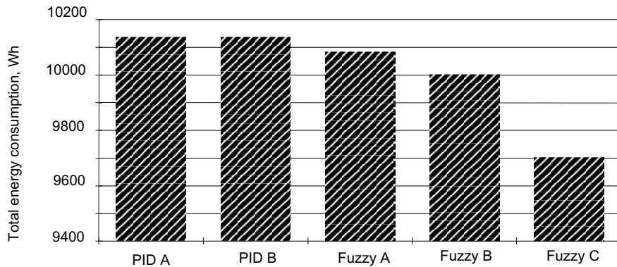
Figure 12.15 Comparison of cumulative energy consumption for both stages of the laboratory plant for total of six steps input disturbances
