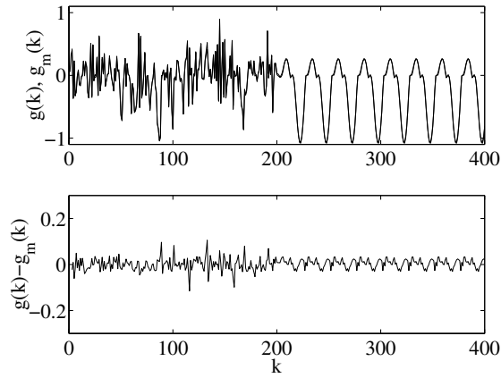
Figure 1.11 Simulation of the six-rule TS singleton model and the error in the estimated output
