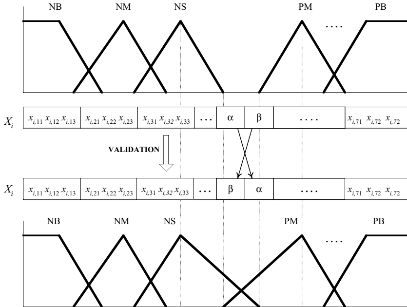
Figure 11.8 Validation of S_i
