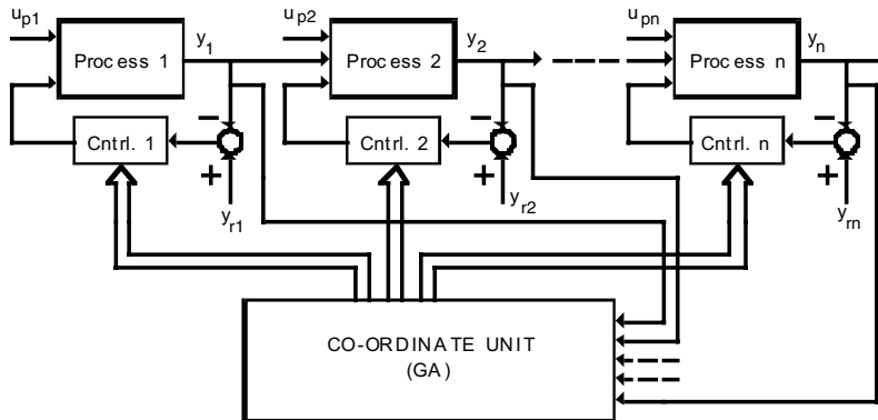
Figure 12.1 Block diagram of a coordinate control concept
