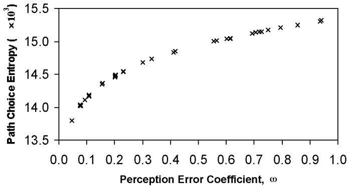
Figure 7.10 Path choice entropy vs. perception error coefficient
