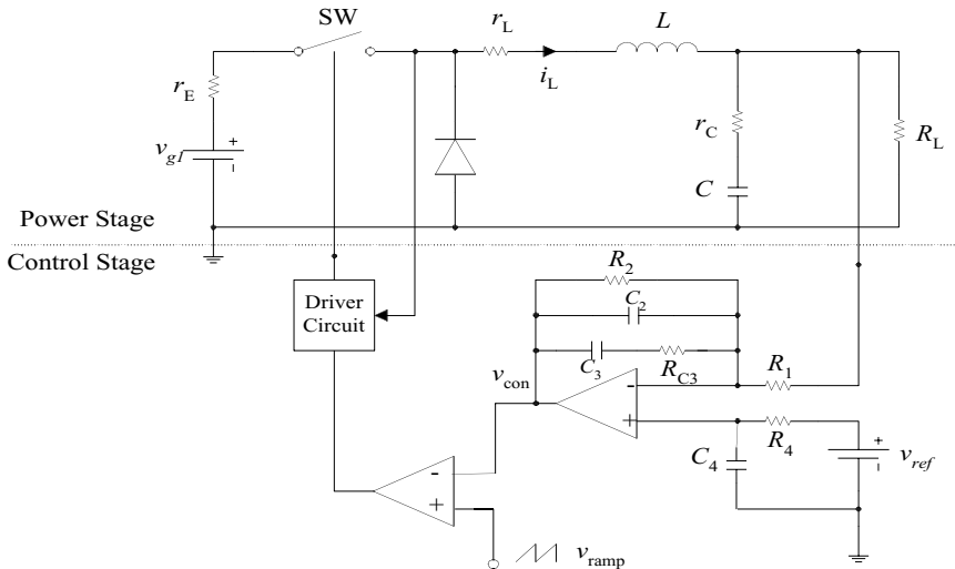
Figure 4.6 Buck regulator with overcurrent protection
