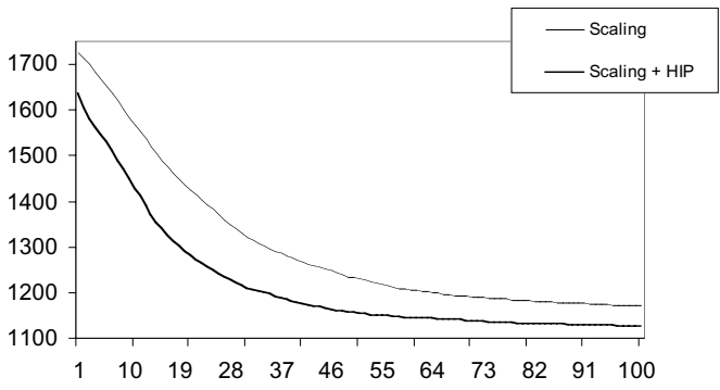
(b) Mean fitness evolution with fitness1
