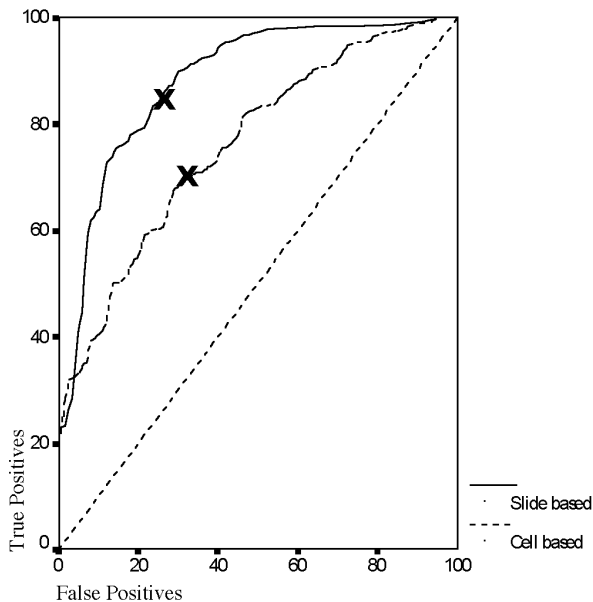
Figure 5.11 ROC curves for test on train results
