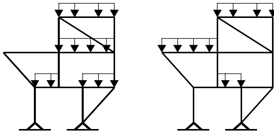
Figure 9.19 Application of alternating span live loading to an example structure
