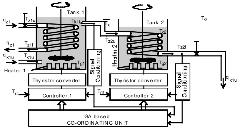
Figure 12.2 Block diagram of laboratory plant
