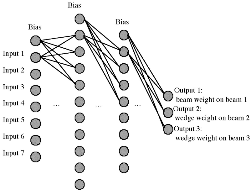
Figure 13.9 Neural network architecture showing inputs and outputs (some connection lines are not shown)
