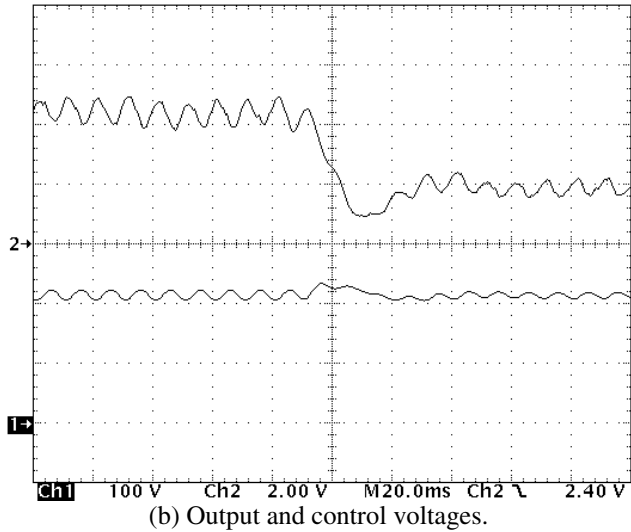
(b) Output and control voltages.
