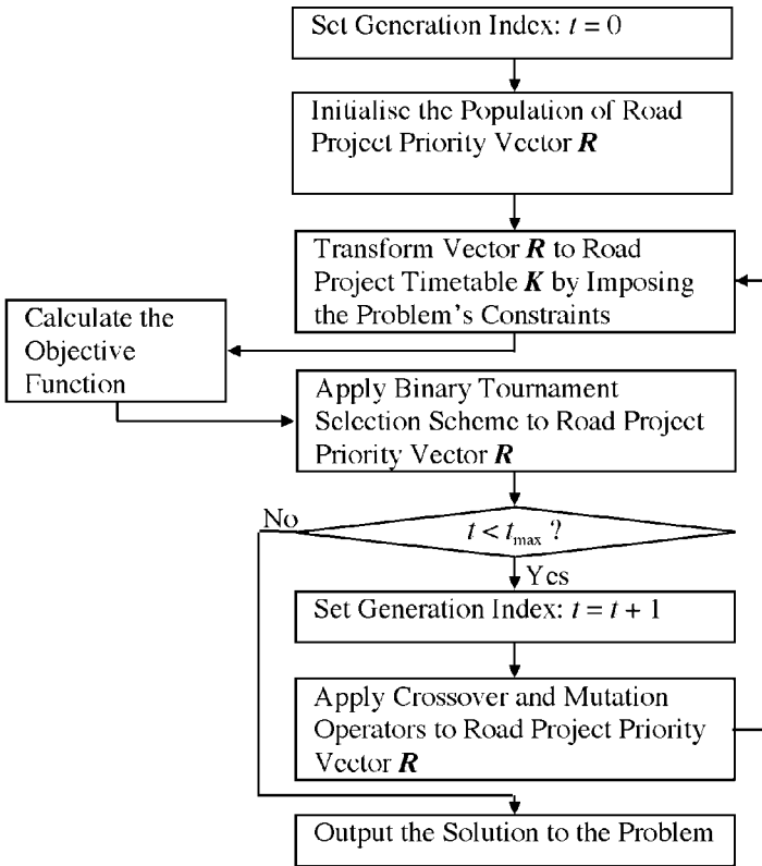
Figure 3.1 The genetic algorithm for the road project construction timetable problem
