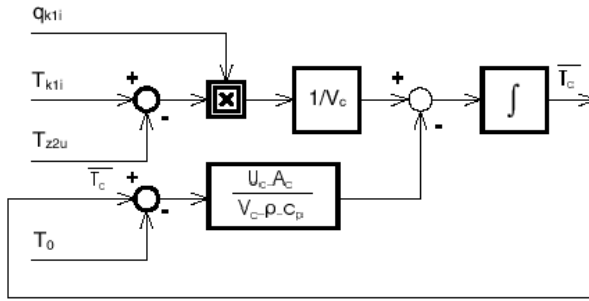
Figure 12.7 Block diagram of the connecting tube
