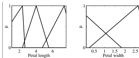
Figure 1.16 Optimized and reduced fuzzy rule-based model with three rules and four misclassifications (Table 1.3-E)
