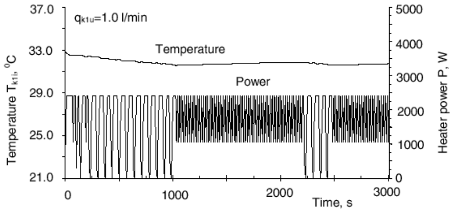
Figure 12.10 First stage response to step disturbance q_{k1u} (from q_{k1u} = 0.5 l/min to q_{k1u} = 1.0 l/min) controlled with genetic algorithm tuned decision tables
