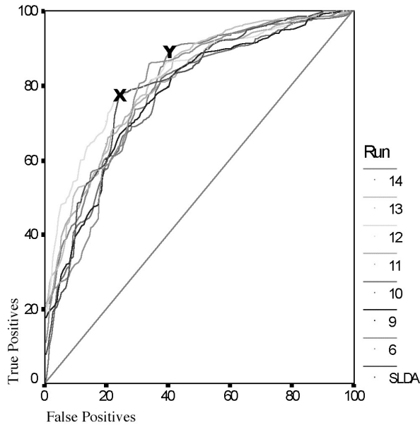
Figure 5.14 ROC curves for test on test results
