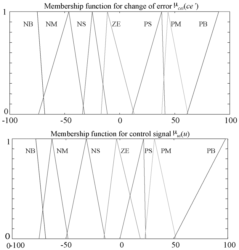
Figure 11.9 GA-trained membership functions
