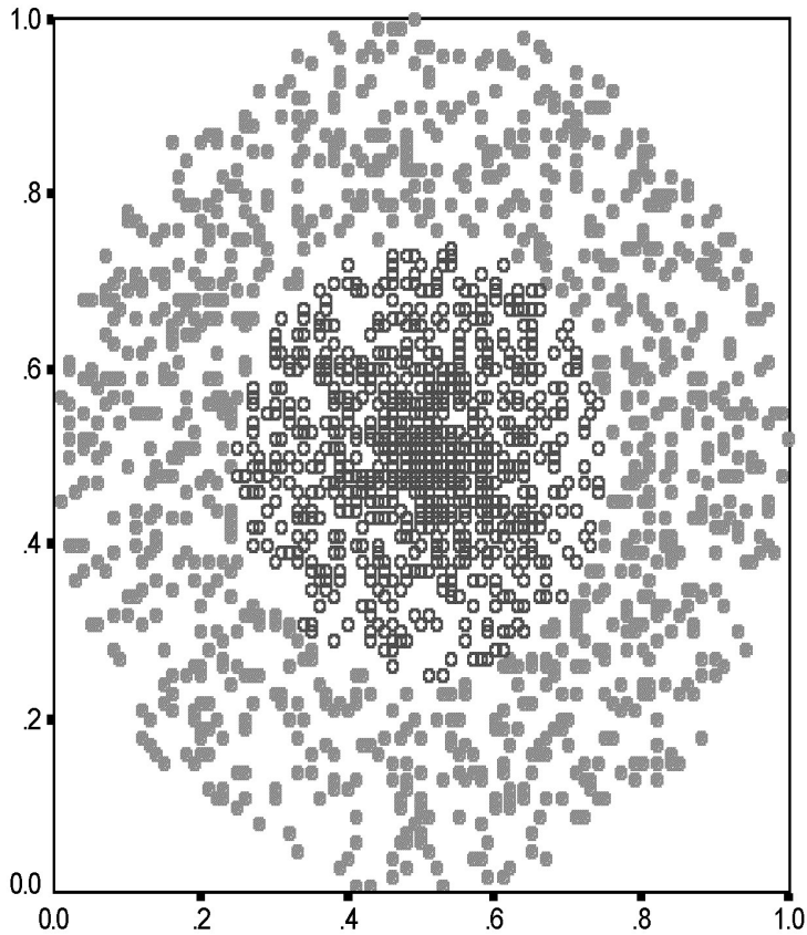
Figure 5.4 Two dimensional training data
