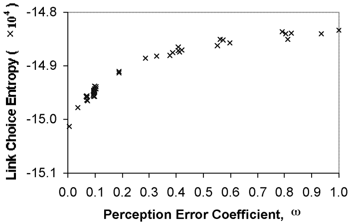
Figure 7.9 Link choice entropy vs. perception error coefficient
