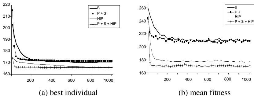
Figure 8.4 Results about convergence of four versions of the GA along 1000 generations. Mean values of 15 experiments are considered for one of the 60 problems. As before, fitness1 values are shown in every case
