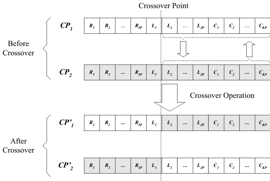
(a) Crossover operation.
