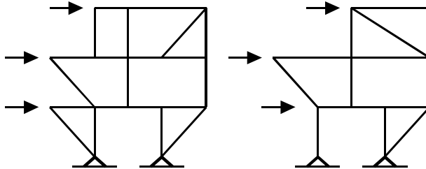
Figure 9.21 Application of wind loading to the exterior nodes of two example structures
