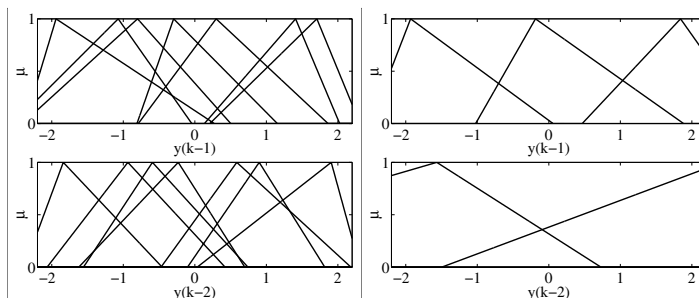
Figure 1.7 Initial fuzzy sets and fuzzy sets in the reduced model
