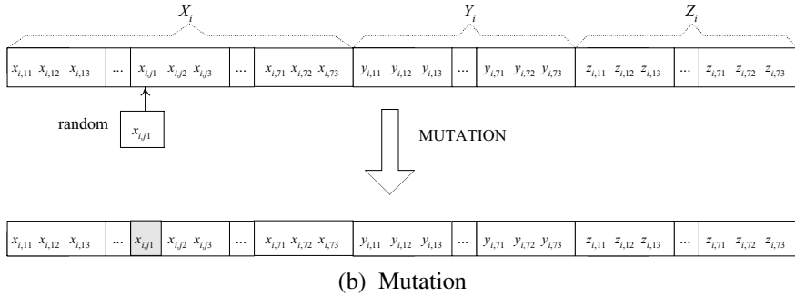
Figure 11.7 Crossover and mutation operations
