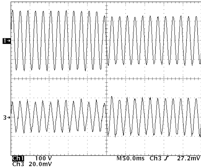
(a) Input voltage and input current waveforms.
