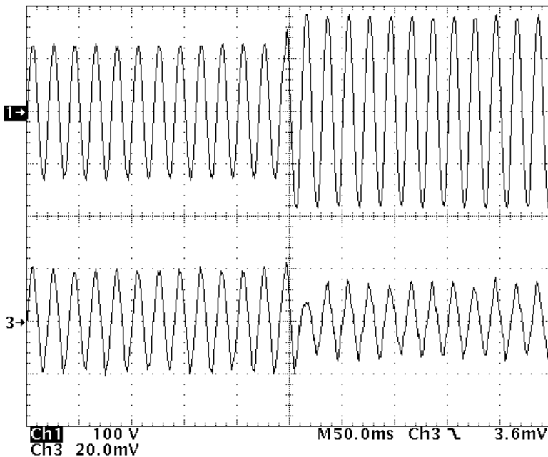
(a) Input voltage and input current waveforms.
