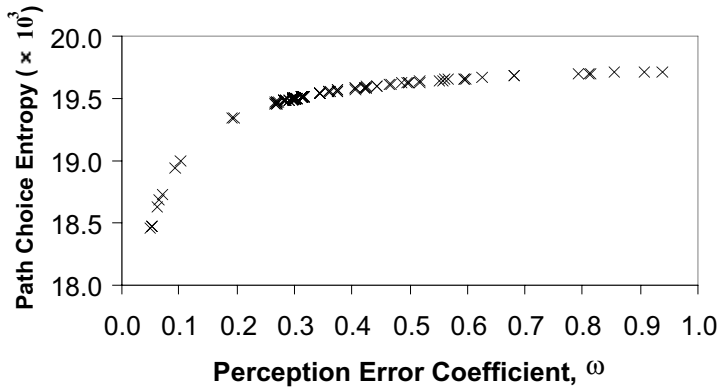
Figure 7.12 Path choice entropy vs. perception error coefficient in the pilot tests
