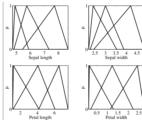
Figure 1.14 Initial fuzzy rule-based model with three rules and 33 misclassifications
