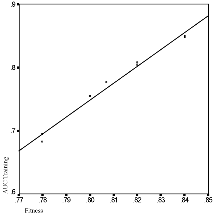
Figure 5.9 Correlation of AUC on the training data with maximum fitness for the parameterization experiments
