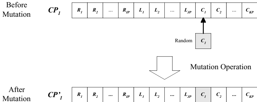
(b) Mutation operation.
