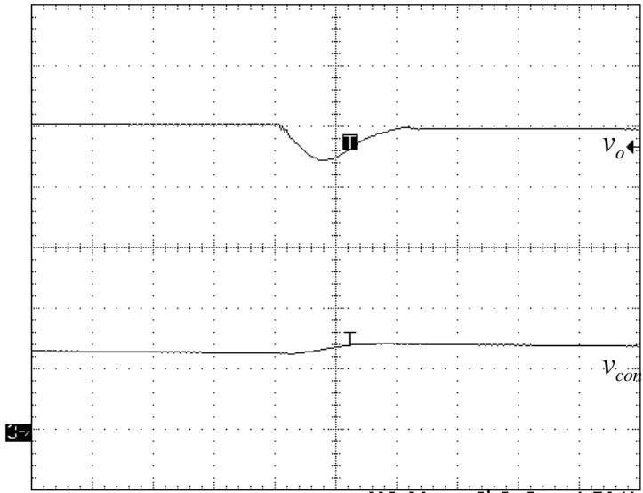
(a) v_o (1V/div) and v_{con} (1V/div). [Timebase: 2ms/div]
