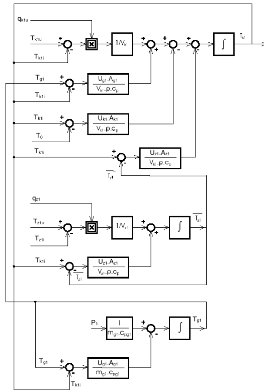
Figure 12.5 Block diagram of the first stage of plant
