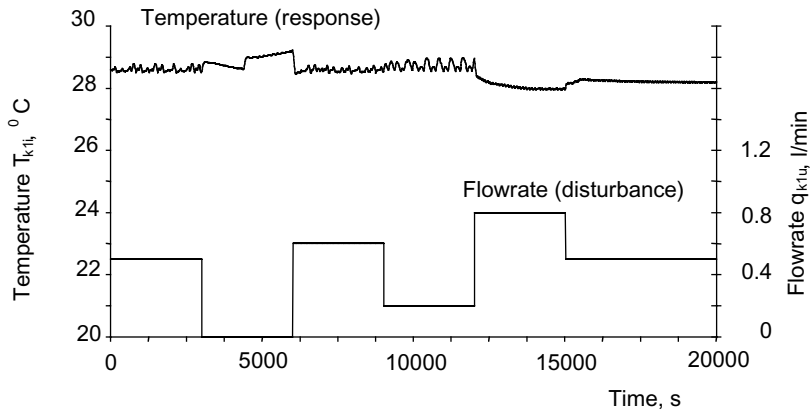
Figure 12.18 Behavior of the first stage of a plant controlled by fuzzy controllers (decision tables are GA tuned) for set point T_r = 28.6^\circ\text{C}
