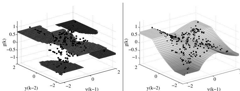
Figure 1.8 Local singleton models and the response surface
