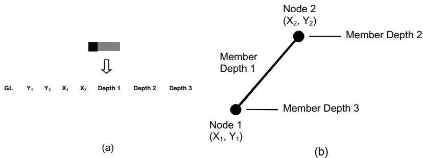
Figure 9.6 Definition of design variables encoded in the IRR GA genotype. (From Raich & Ghaboussi, in press.)
