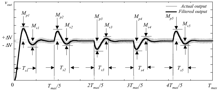
Figure 11.6 Typical output response of the boost rectifier
