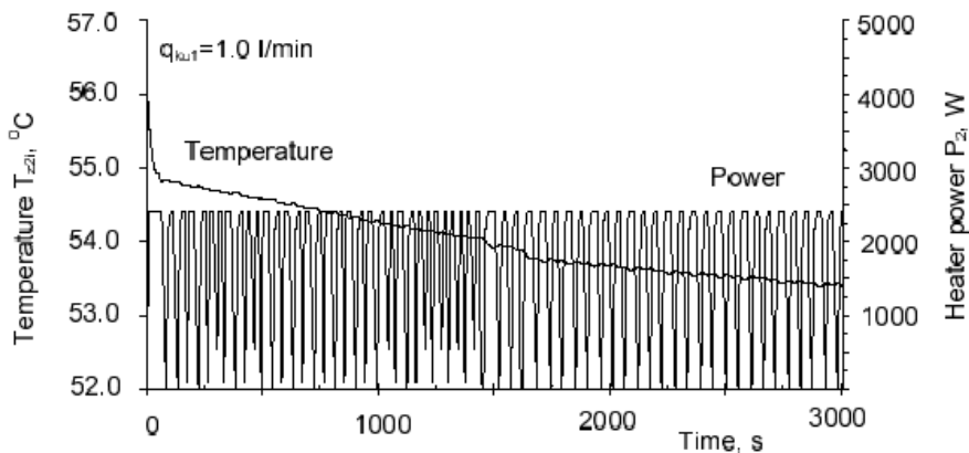
Figure 12.12 Second stage response to step disturbance q_{klu} (from q_{klu} = 0.5 l/min to q_{klu} = 1.0 l/min) controlled with genetic algorithm tuned decision tables
