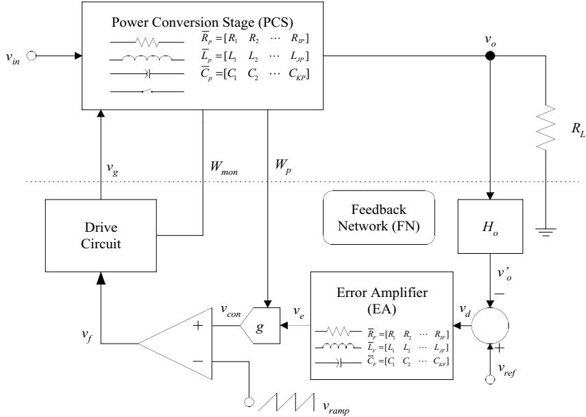
Figure 4.1 Block diagram of power electronics circuits: chromosome structures and the fitness functions
