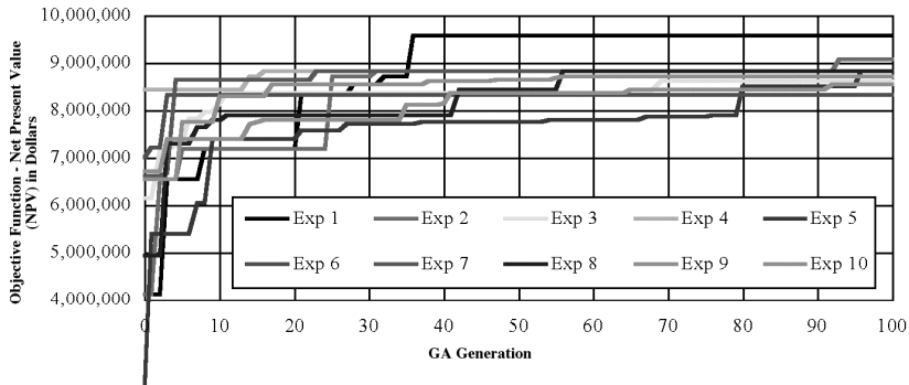
Figure 3.4: Comparison of the Steps in the Improvement of the Objective Function Values of the Best individuals over GA Generations in Ten Experiments
