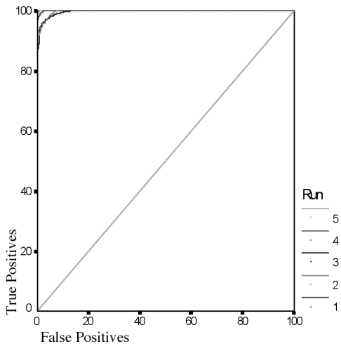
Figure 5.5 ROC curves for 2-D data: select 2 from 7 features, training set
