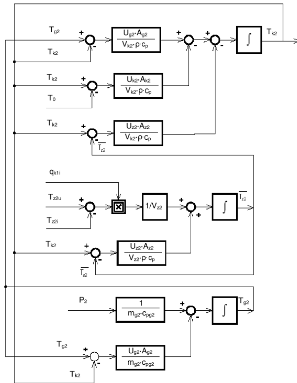
Figure 12.6 Block diagram of the second stage of plant
