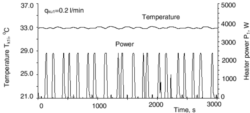
Figure 12.11 First stage response to step disturbance q_{klu} (from q_{klu} = 0.5 l/min to q_{klu} = 0.2 l/min) controlled with genetic algorithm tuned decision tables
