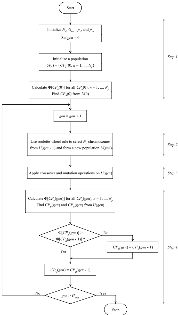
Figure 4.4 Flowchart of the optimization steps of PCS
