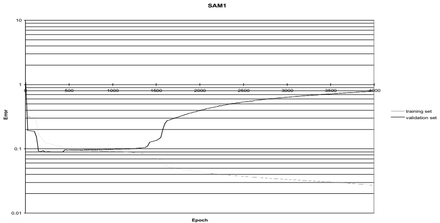
Figure 13.12 A plot of training set error and validation set error against epoch for SAM
