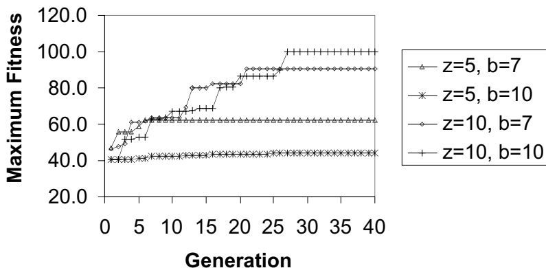
Figure 7.14 Maximum fitness vs population size, generation, length of chromosome
