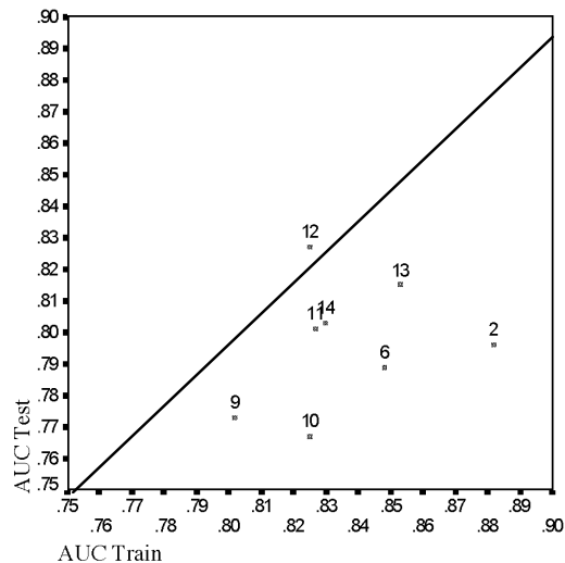
Figure 5.15 Generalizability of the MACs classifiers
