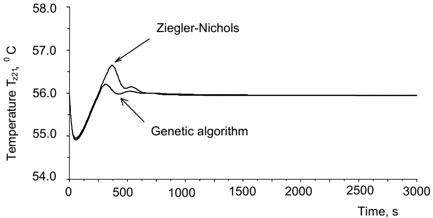
Figure 12.9 Second process stage response for Ziegler-Nichols and GA tuned PID_2 controller for step input q_{k1u} from q_{k1u} = 0.5 l/min to q_{k1u} = 1.0 l/min
