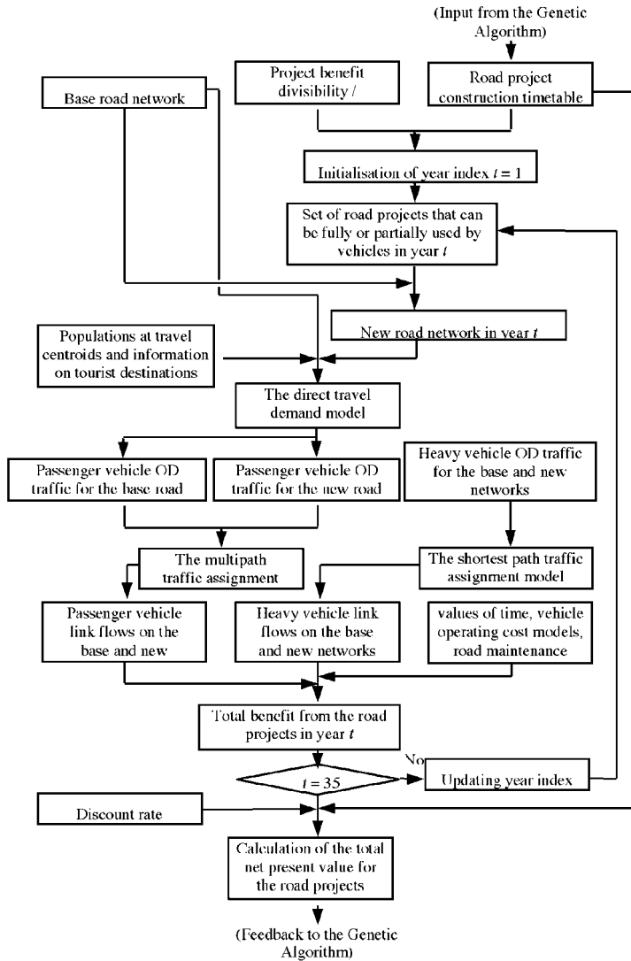
Figure 3.3 Procedure for calculation of the objective function value
