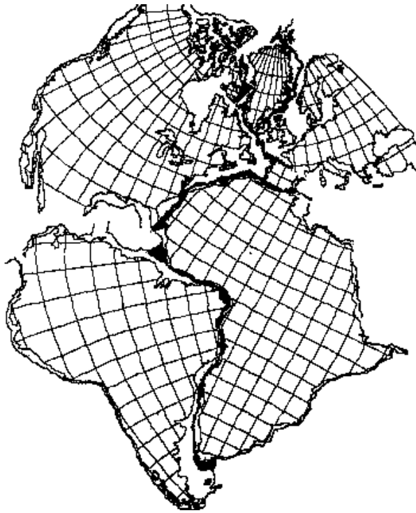
Figure 0.5 The fit of the continents around the Atlantic
