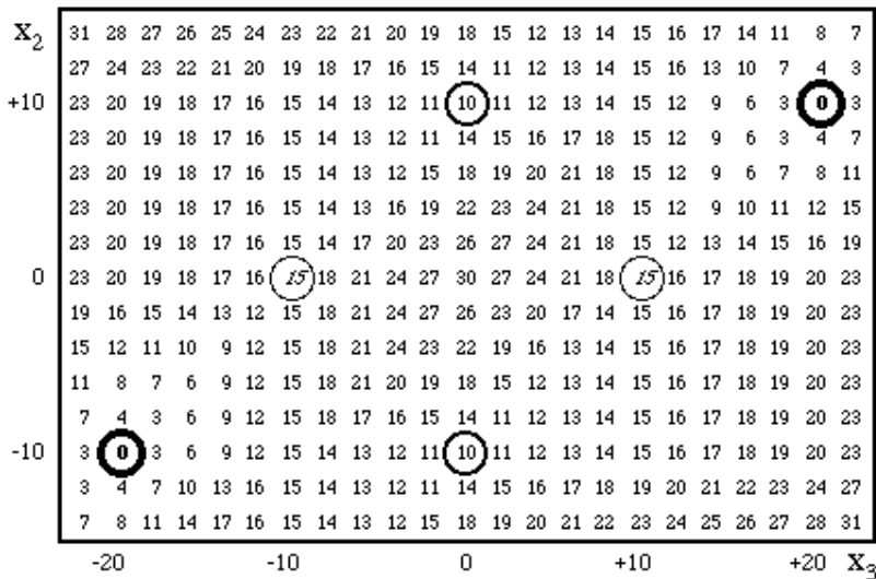
Figure 6.2 Misfit function ( Y ) for the one-dimensional example
