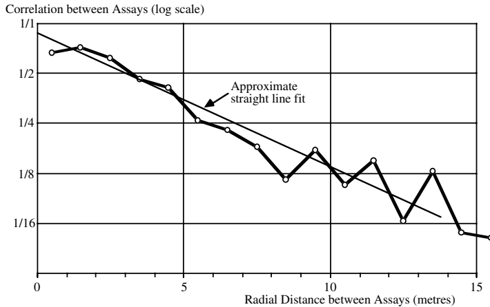
Figure 0.9 Log correlations as a function of r , the inter-assay distance
