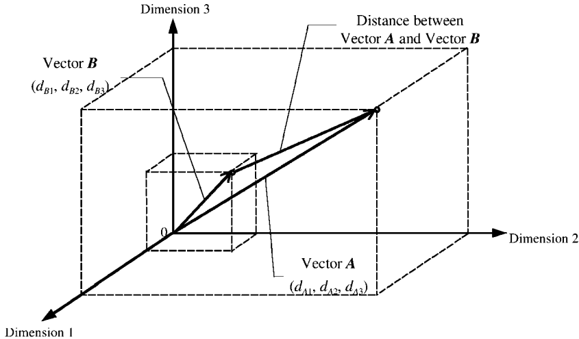
Figure 3.5 Euclidean distance between two vectors in a R^3 space
