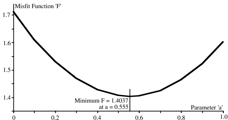
Figure 0.11 Fitting model 0: \rho(r) = a
