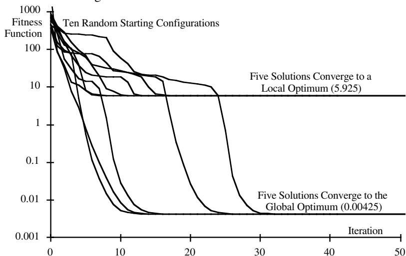
Figure 6.5 Systematic projection from ten random starting configurations
