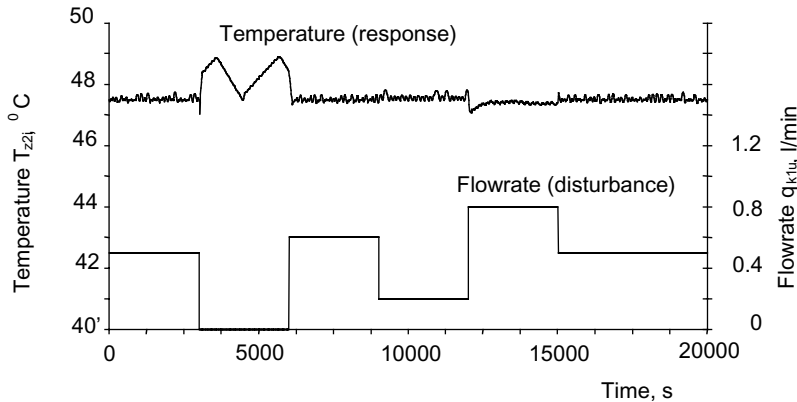
Figure 12.19 Behavior of the second stage of a plant controlled by fuzzy controllers (decision tables are GA tuned) for set point T_r = 47.5^\circ\text{C}
