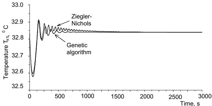
Figure 12.8 First process stage response for Zeigler-Nichols and GA tuned PID, controller for step input q_{k1u} from q_{k1u} = 0.5 l/min to q_{k1u} = 1.0 l/min
