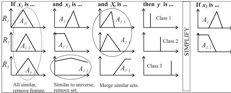
Figure 1.4 Similarity-driven simplification
