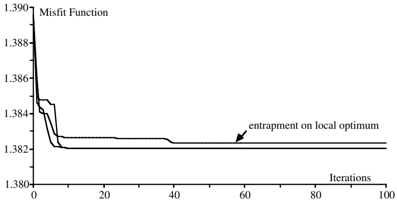
Figure 0.15 Fit of model 3 using systematic projection
