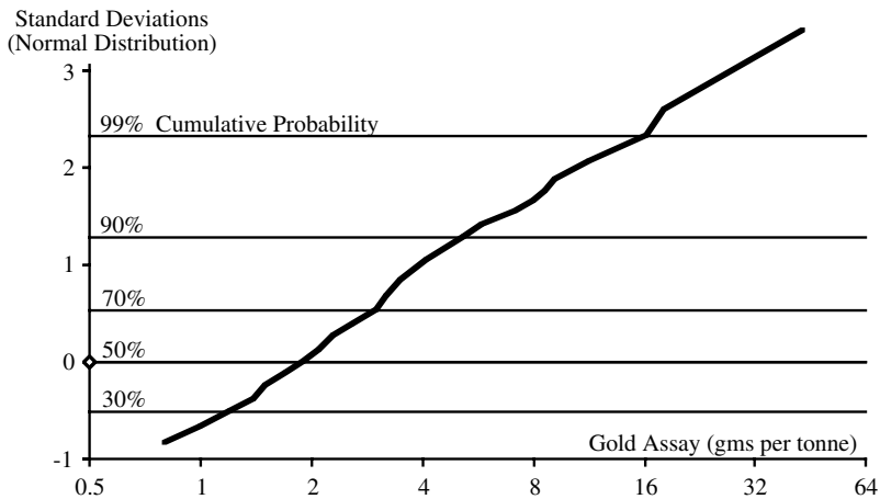
Figure 0.7 Cumulative distribution of gold assays, on log normal scale
