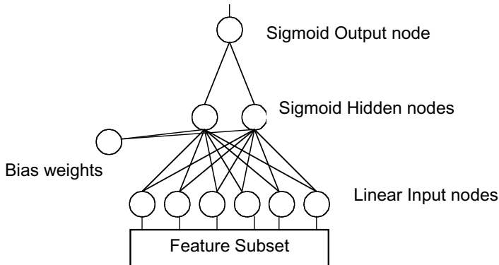
Figure 5.2 Architecture of the neural network
