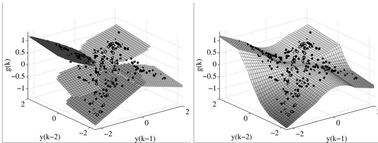
Figure 1.12 Local linear TS model and the response-surface
