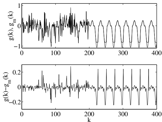
Figure 1.9 Simulation of the six-rule TS singleton model and error in the estimated output
