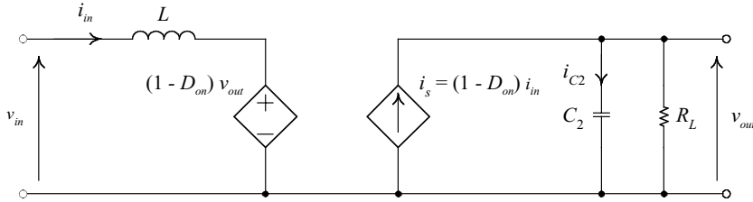
Figure 11.2 Behavioral model of the APFC
