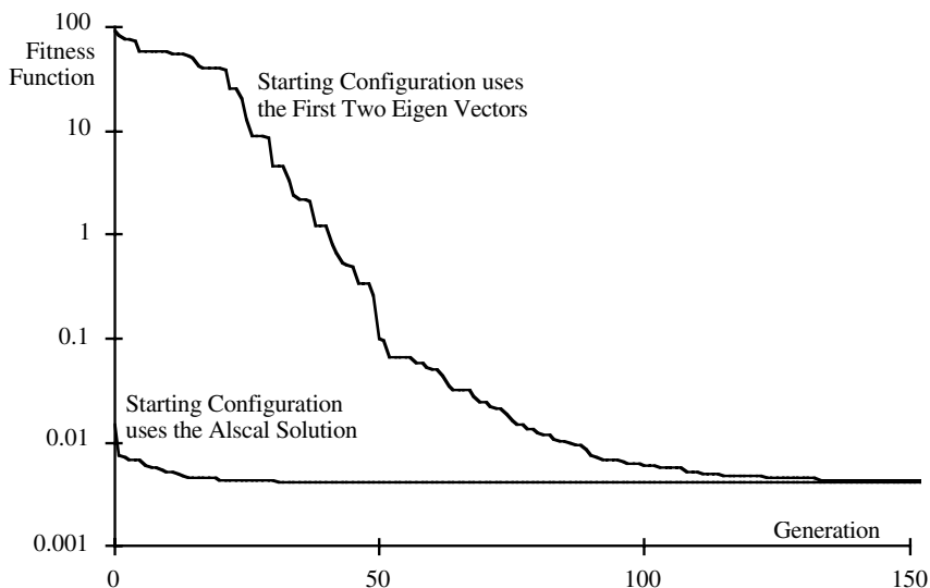
Figure 6.7 Starting from Eigen vectors and from the Alsca solution
