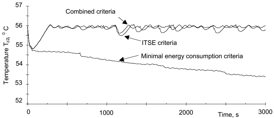
Figure 12.23 Second stage process response for various optimizing criteria
