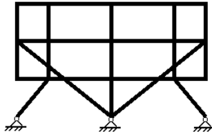
Figure 9.30 Frame design solutions for four trials represented by the fittest population individual of each IRR GA trial. (From Raich & Ghaboussi, in press.)
