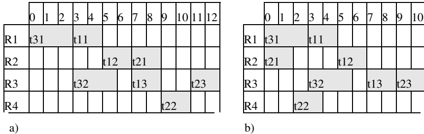
Figure 8.2 (a) Scheduling produced by the fitness1 strategy to the problem of Figure 8.1 from the individual (3 3 1 1 1 2 2 2). The fitness1 value is 13. (b) Scheduling produced from the same individual by the fitness2 strategy. The fitness2 value is 11
