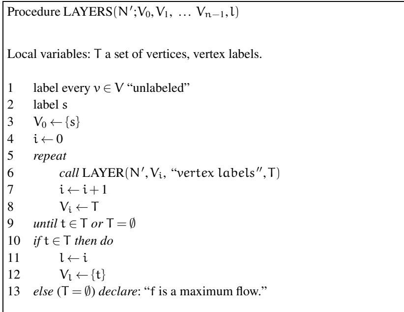
Algorithm 5.5: Finding the BFS Layers of N' .
