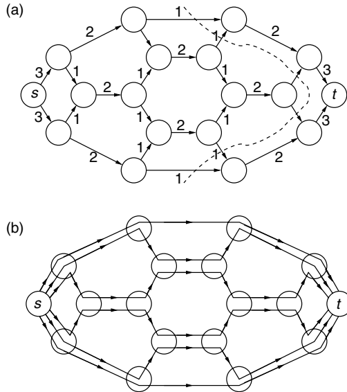
Figure 6.5: (a) The minimum flow in the PERT; (b) decompositions of the flow into the PERT into F directed paths.
