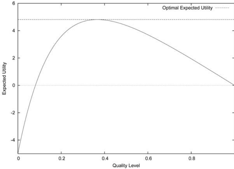
FIGURE 1. Quality level vs expected utility. V_m \sim Exp(5) , g_m(v) = -10 \cdot v + 10 , h_m(v) = -15 \cdot v + 15
