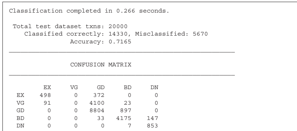
Figure 6.4 The results of credit worthiness classification for the classifier based on a neural network
