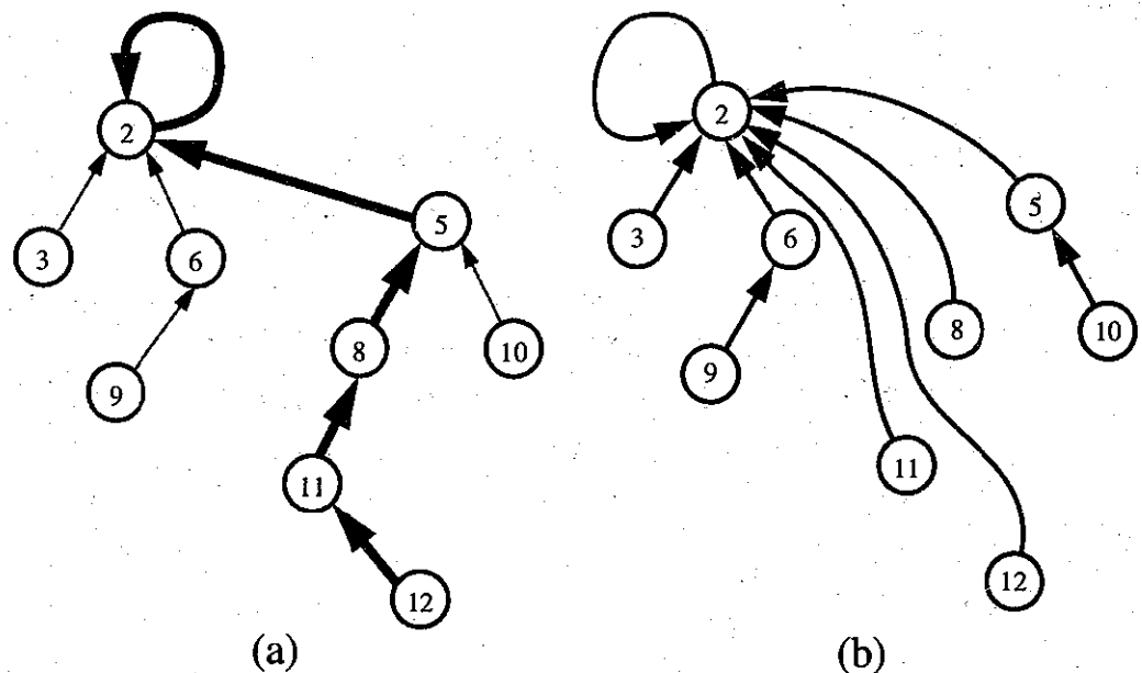
Figure 4.9: Path-compression heuristic: (a) path traversed by operation find on element 12; (b) restructured tree.
