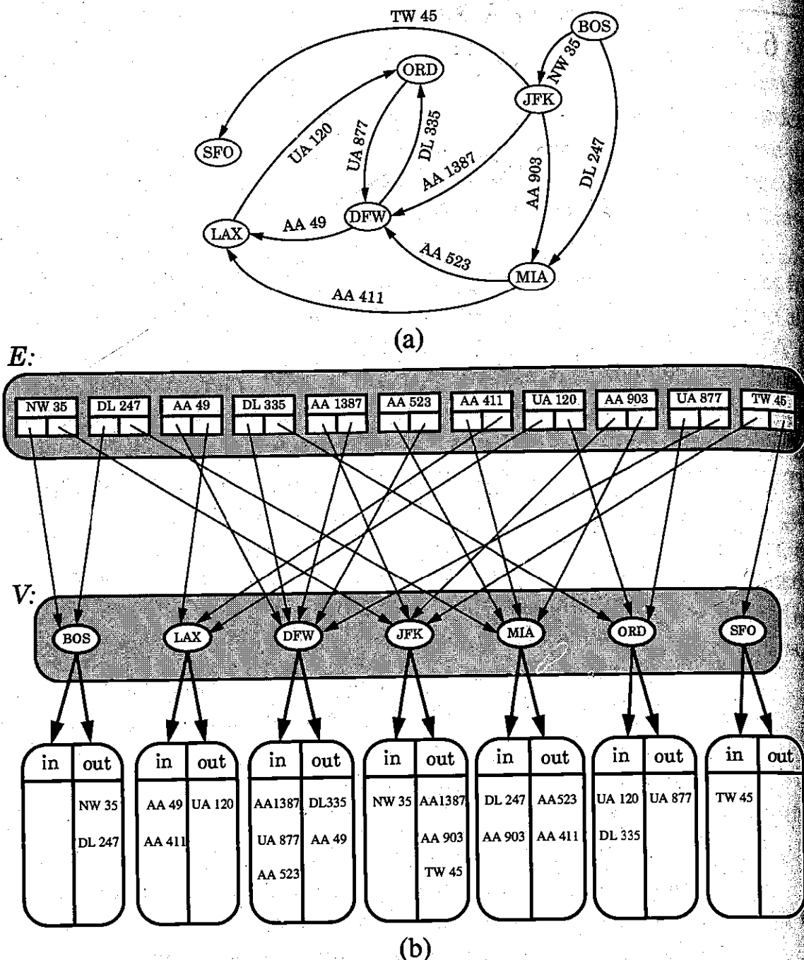
Figure 6.4: (a) A directed graph G ; (b) schematic representation of the adjacency list structure of G . As in Figure 6.3, we visualize the elements of containers with names. Also, we only show the incidence containers for directed edges, since there are no undirected edges in this graph.
