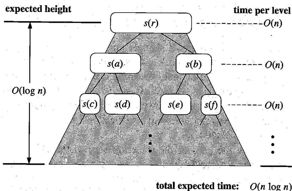
Figure 4.13: A visual time analysis of the quick-sort tree T .
