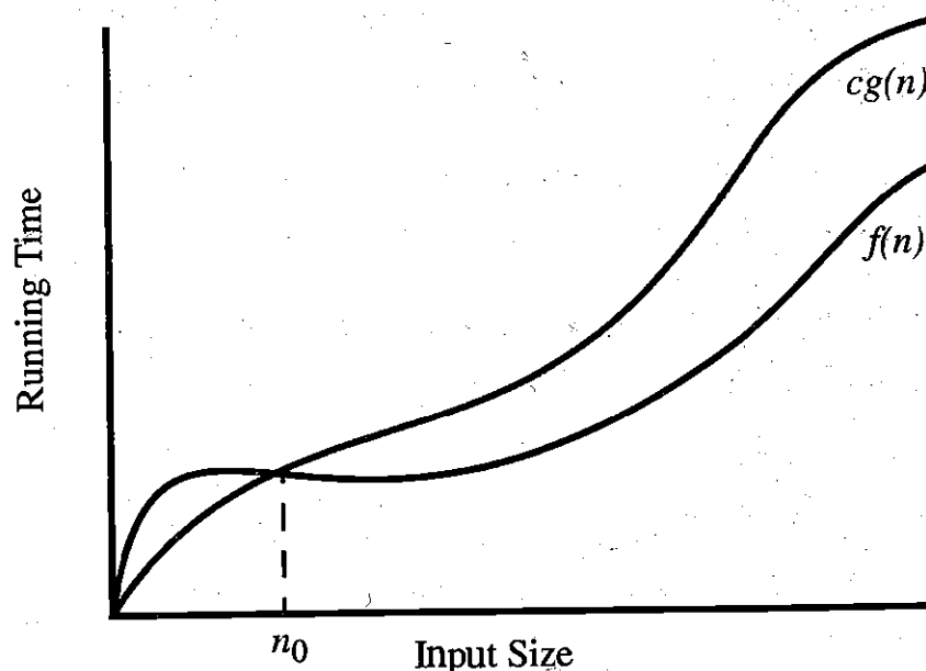
Figure 1.5: Illustrating the "big-Oh" notation. The function f(n) is O(g(n)) , for f(n) \leq c \cdot g(n) when n \geq n_0 .
