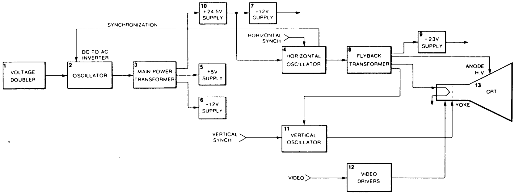
Figure 6-3 Monitor/Power Supply Block Diagram
