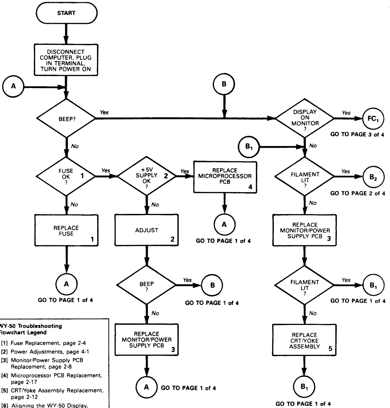
Figure 3-2 Troubleshooting Flowchart
