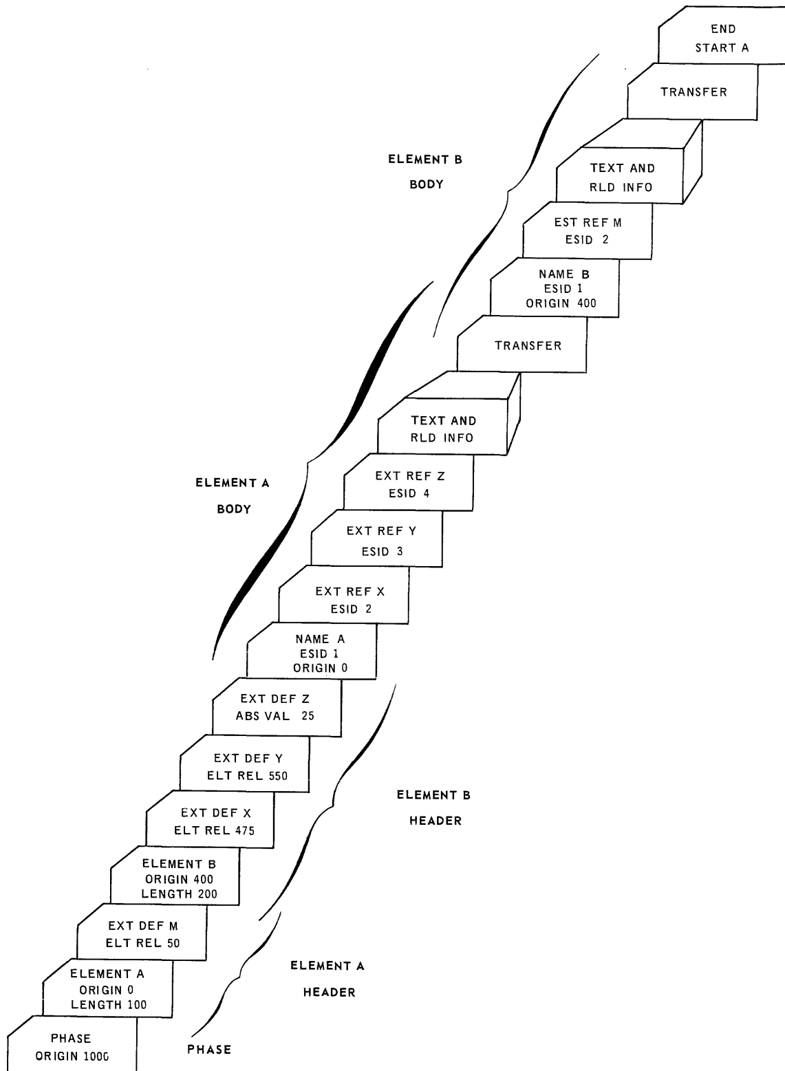
Figure 5-2. Linker Input
