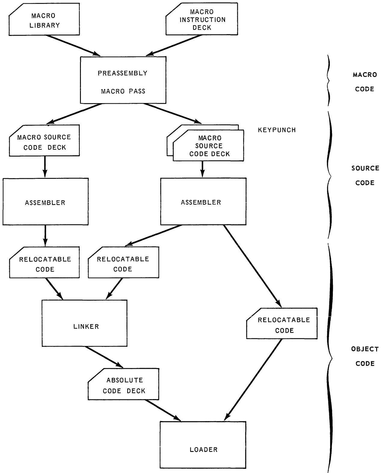
Figure 1-2. 9200/9300 Assembly System
