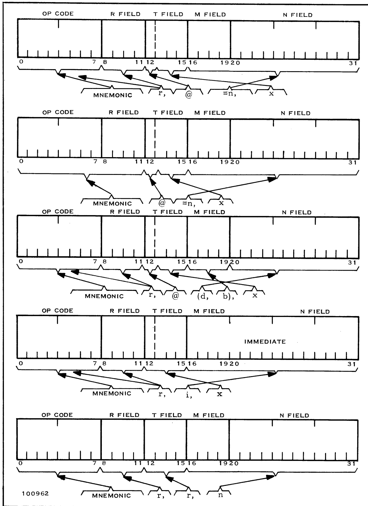
Figure 6-1. Assembler Statement Translations into Machine Code
