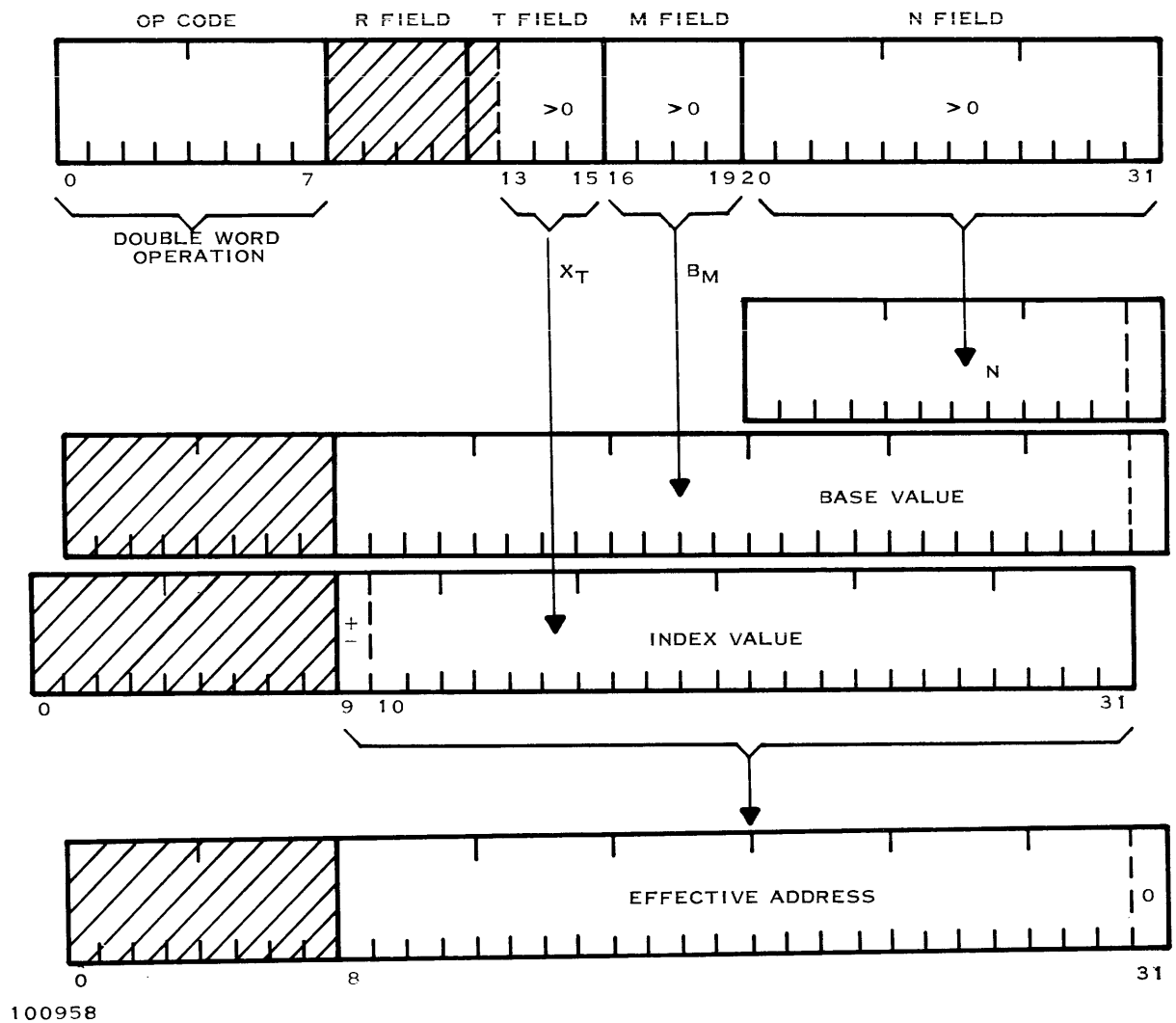
Figure 6-5. Development of Doubleword Effective Addresses
