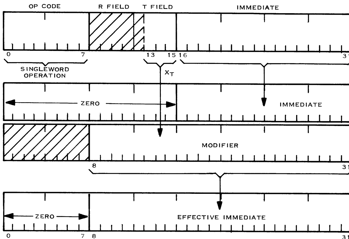
Figure 6-9. Development of Singleword Logical Immediate Operands
