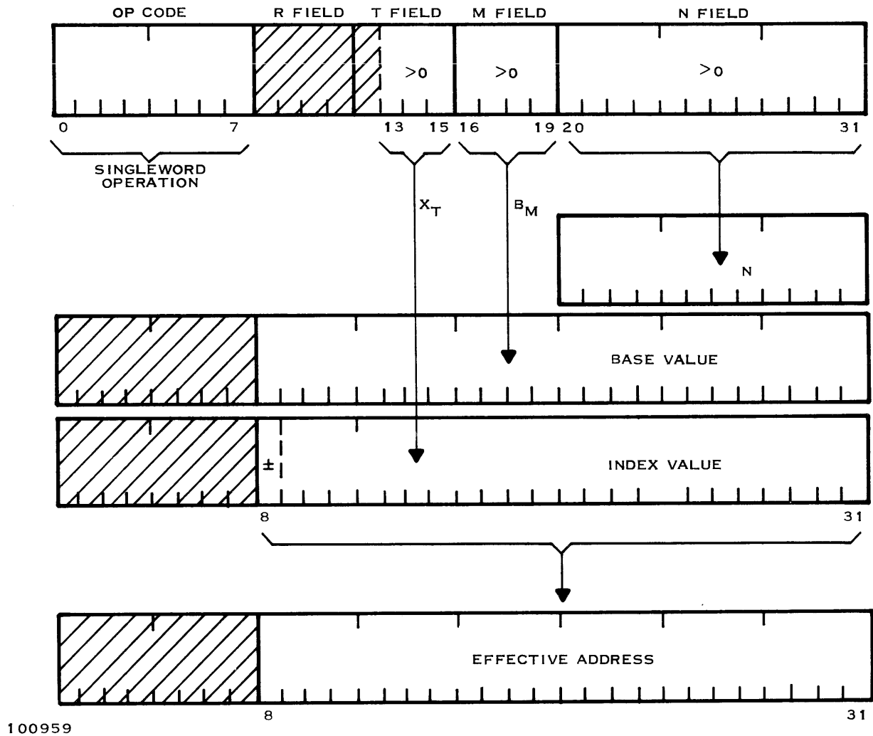
Figure 6-3. Development of Singleword Effective Addresses
