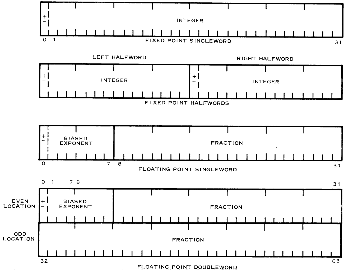
Figure 6-12. Algebraic Data Formats
