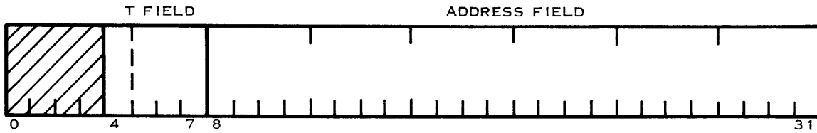
Figure 6-6. Indirect Address Cell Format
