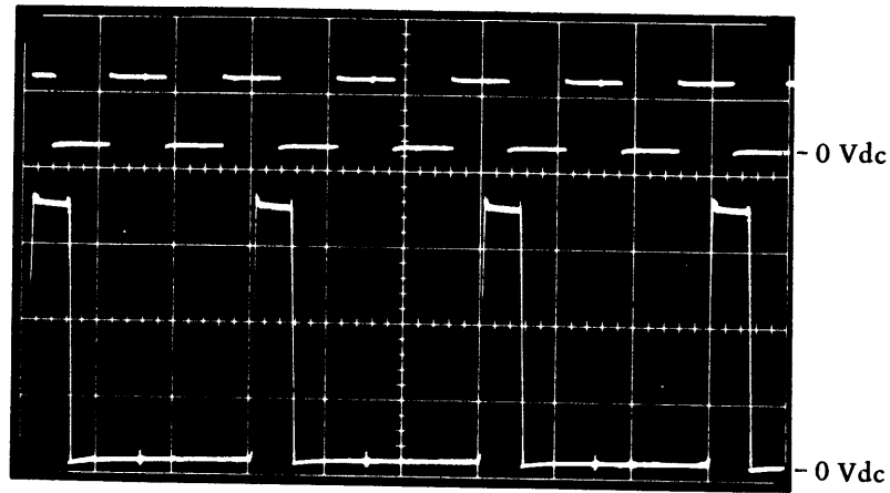
Figure 5-3. Waveform 2
