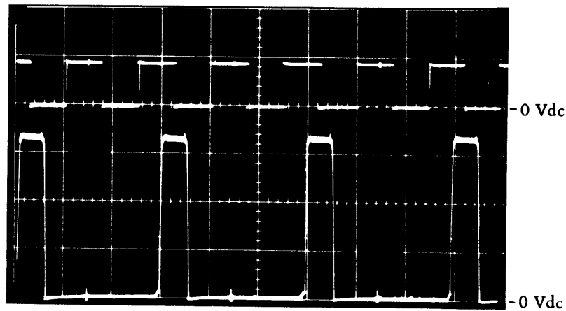
Figure 5-5. Waveform 4
