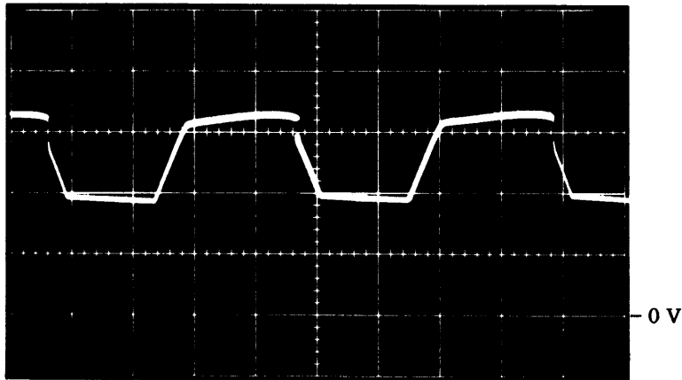
Figure 5-11. Waveform 10
