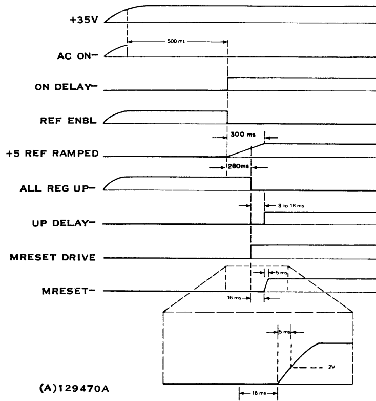
Figure 4-11. Turn-On Sequence Timing
