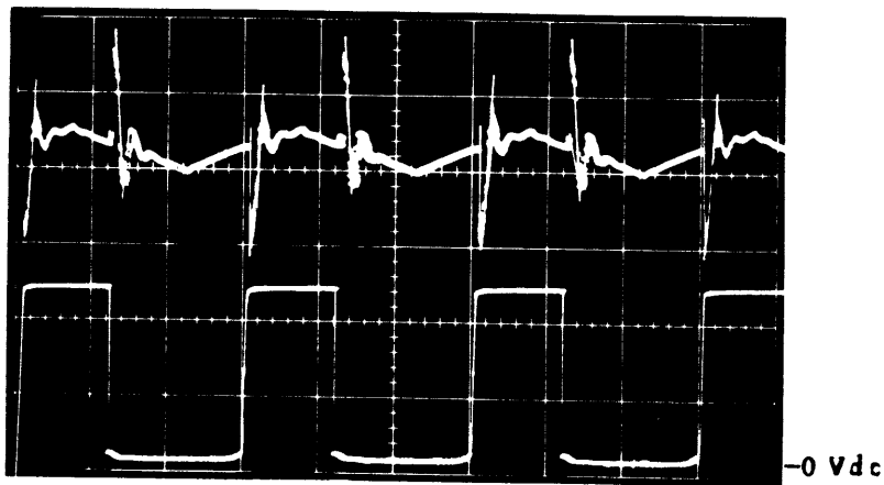
Figure 5-7. Waveform 6
