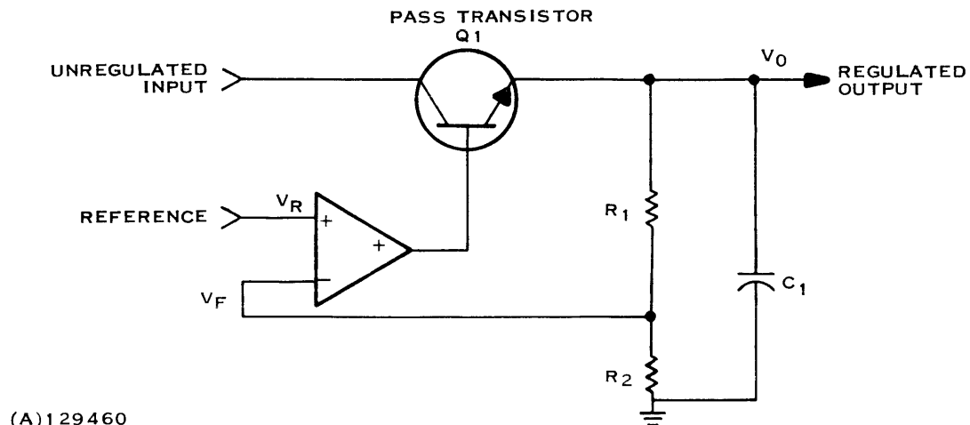
Figure 4-1. Series Regulator Circuit Diagram
