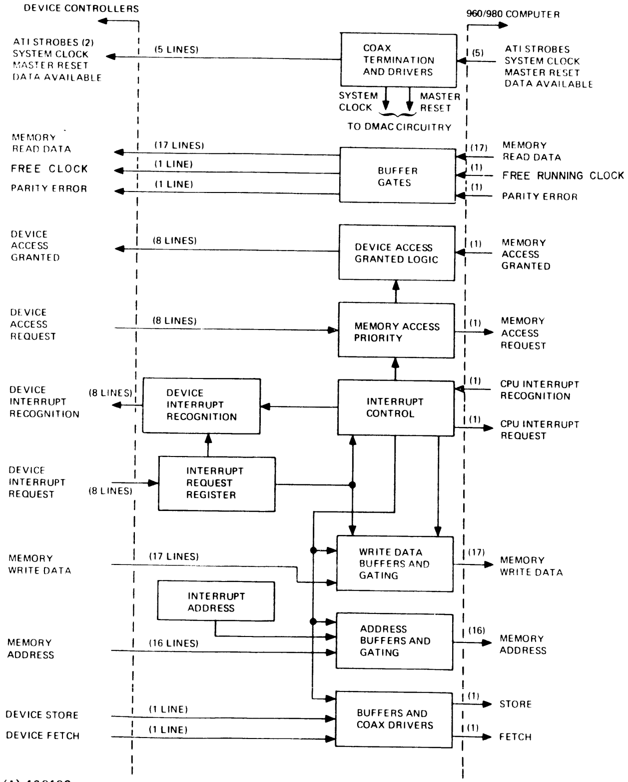
Figure 3-1. DMAP Expander Block Diagram
