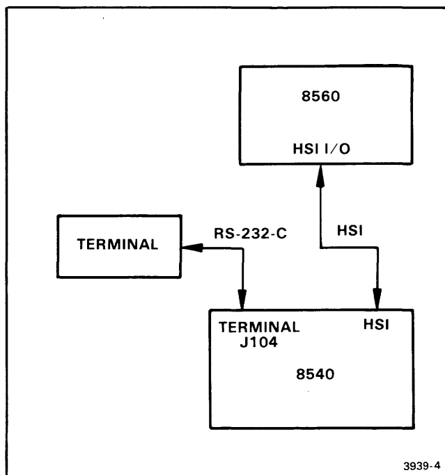
Fig. 2-1. Hardware configuration for 8540/8560 interface.
