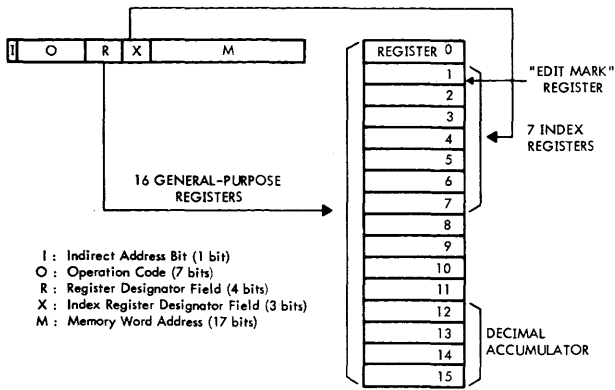
Figure 4. Register and instruction format.
