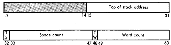
Figure 10. Stack pointer.
