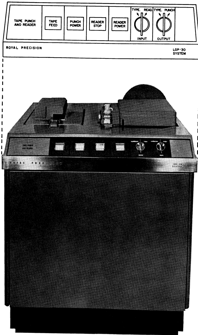
FIGURE 8. Photo-Electric Reader Model 342
