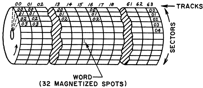
FIGURE 1. Magnetic Drum; 4096 Word Memory
