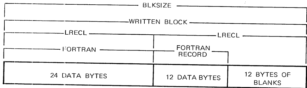
FIGURE 2-7. FIXED-LENGTH BLOCKED RECORDS WRITTEN UNDER FORMAT CONTROL
