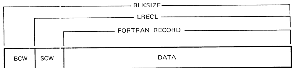
FIGURE 2-4. FORTRAN RECORD (FORMAT CONTROL) WITH VARIABLE-LENGTH SPECIFICATION
