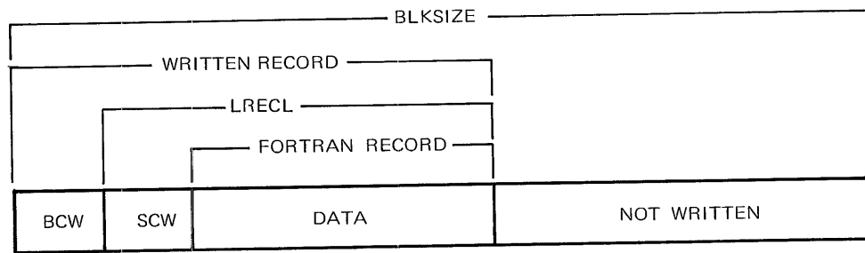
FIGURE 2-5. FORTRAN RECORD (FORMAT CONTROL) WITH VARIABLE-LENGTH SPECIFICATION
