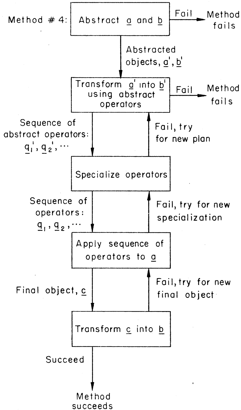
Fig. 7—Planning method
