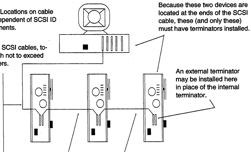
Figure 7-7 SCSI Cable Configuration B
