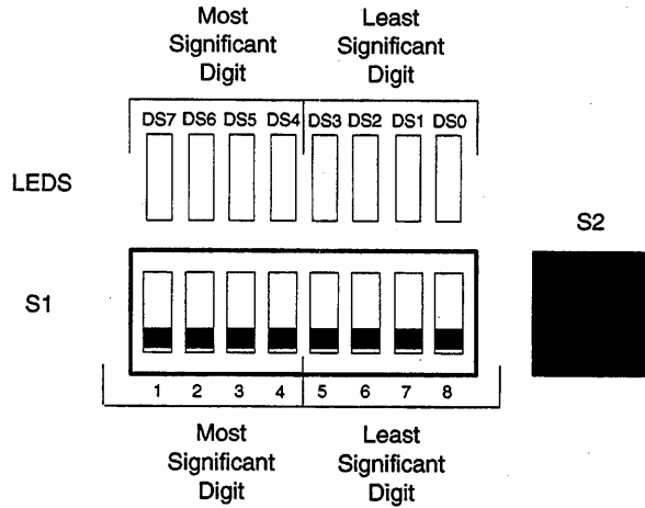
Figure 7-2 Configuration Switch S1, S2 and Display LEDs
