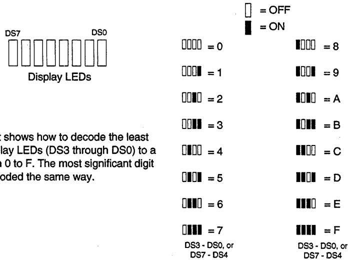
Figure 7-4 SCSI PCBA Display LEDs
