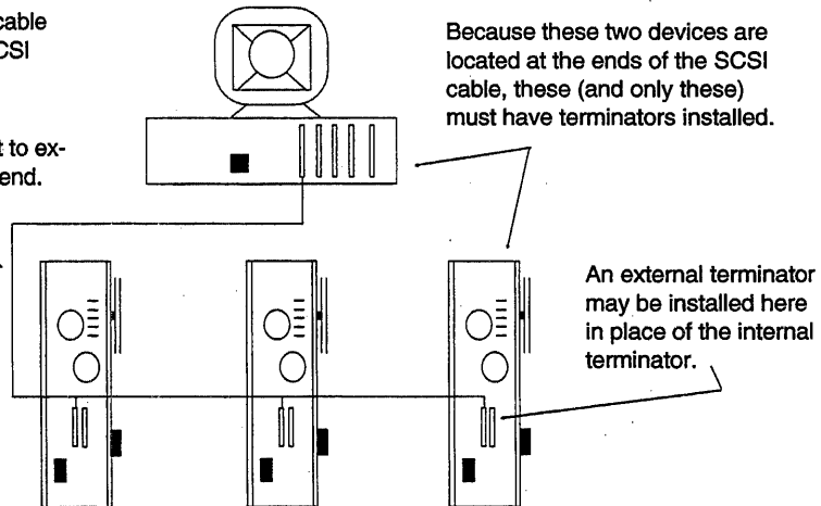
Figure 7-6 SCSI Cable Configuration A
