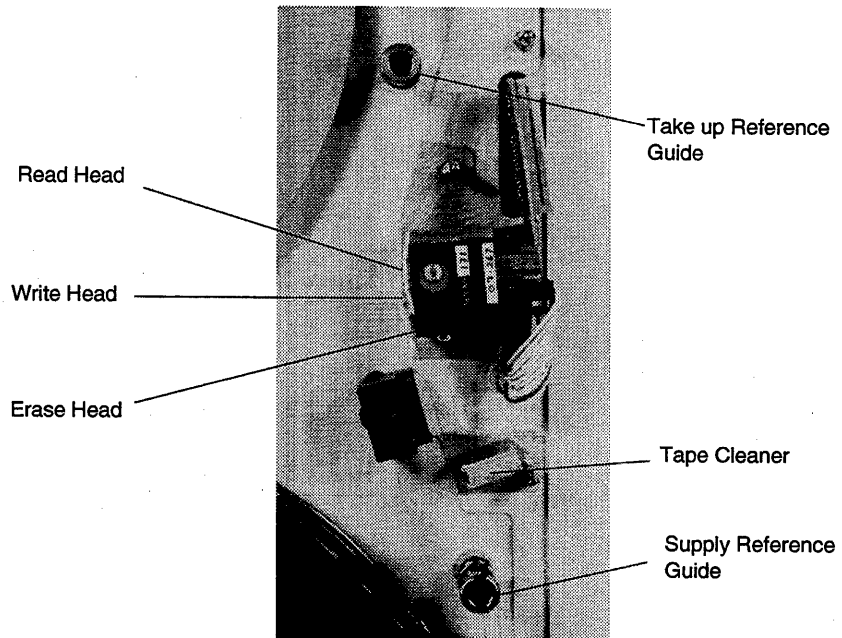
Figure 4-1 Head Area Components
