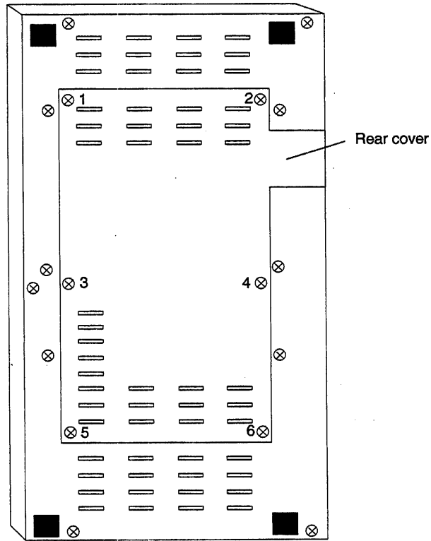
Figure 7-9 1054 Rear View
