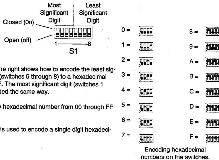
Figure 7-3 SCSI PCBA Switches
