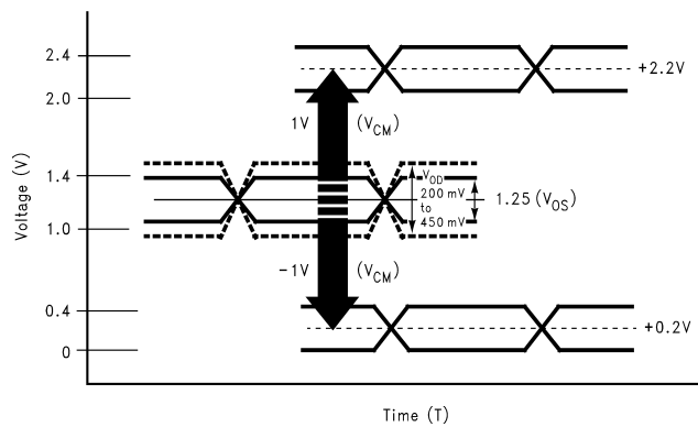
FIGURE 7. The active signal swings of LVDS and Bus LVDS are reduced even further to about 1/4 of the reduced-swing technologies illustrated in Figure 6. However, because LVDS is differential, the common-mode range should be compared to single-ended noise margins. The effective noise margin is two to four times better using LVDS.
