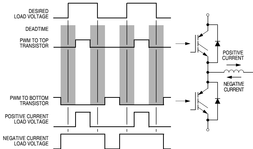
Figure 9-18. Deadtime Distortion
