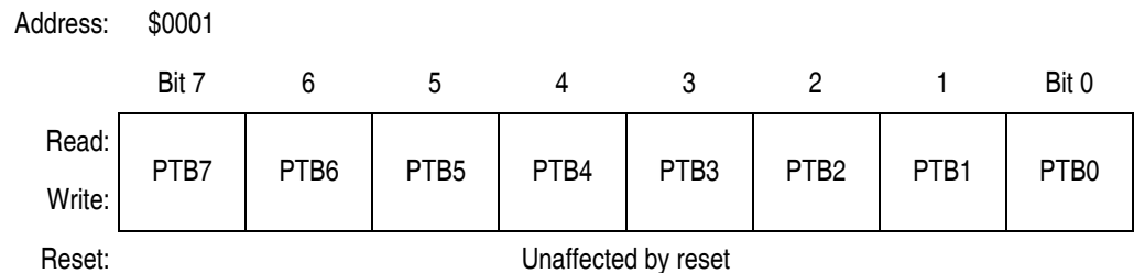
Figure 15-5. Port B Data Register (PTB)
