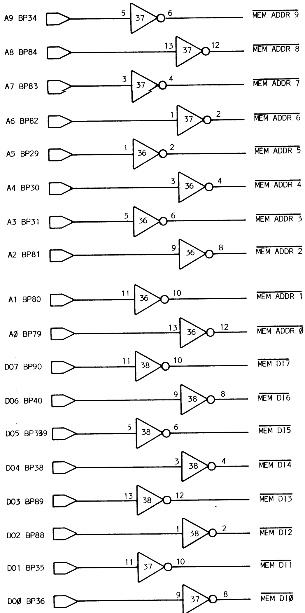
TYPICAL 74LS04
