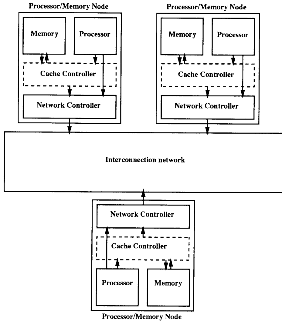
Figure 4-3: Typical network-based architecture supported by the simulator.
