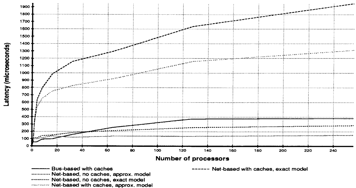
Figure 5-3: Average latency of shared memory operations for various machine configurations and sizes.
