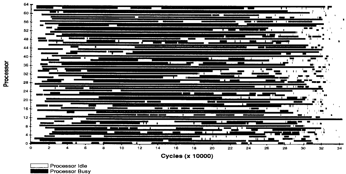
Figure 3-10: Processor lifelines for the 8-queens program with random thread placement (processors=64).
