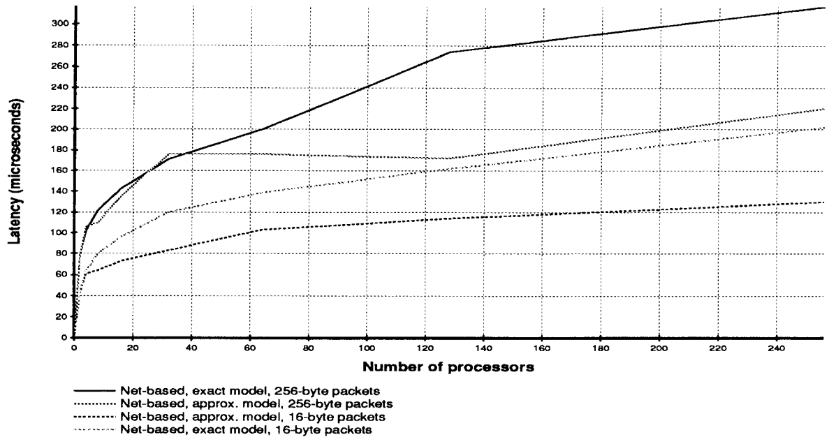
Figure 5-4: Average latency of ipi operations for various machine configurations and sizes.
