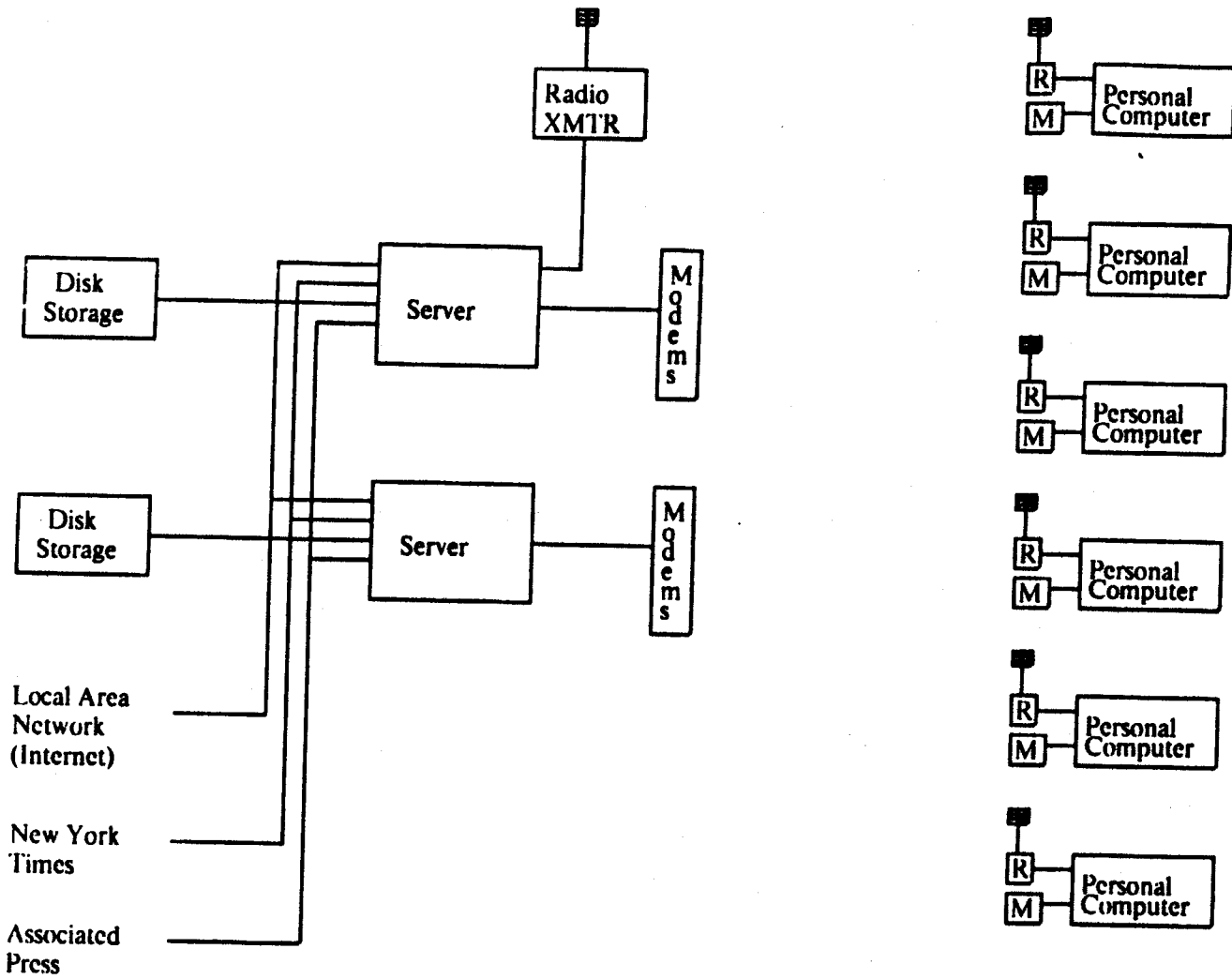
Figure 2-1: Boston CommInS System Block Diagram
