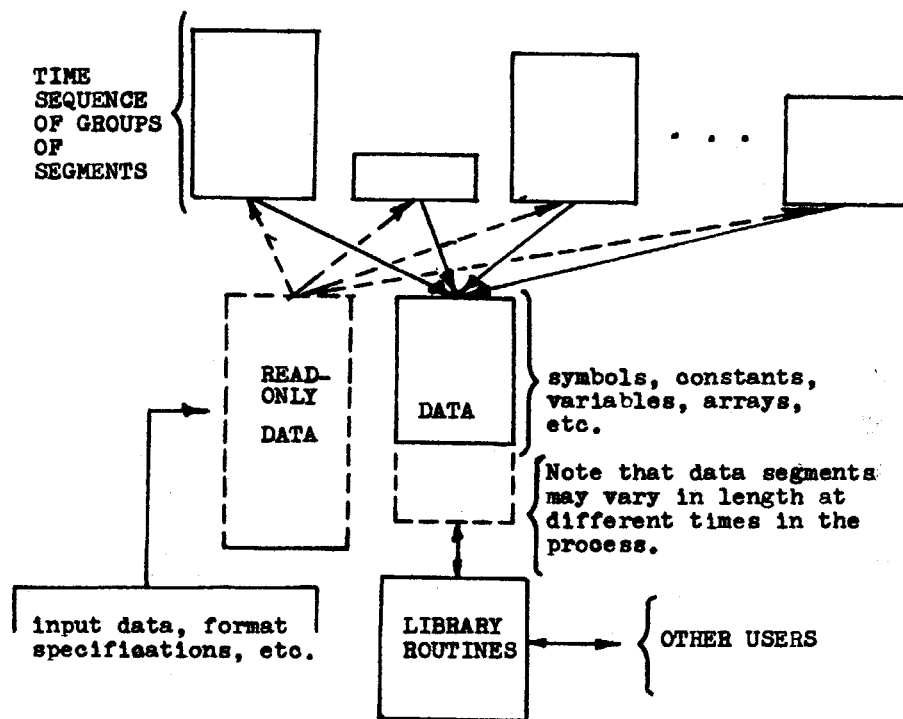
Figure 2.1. Operation of one user in a segmented system.
