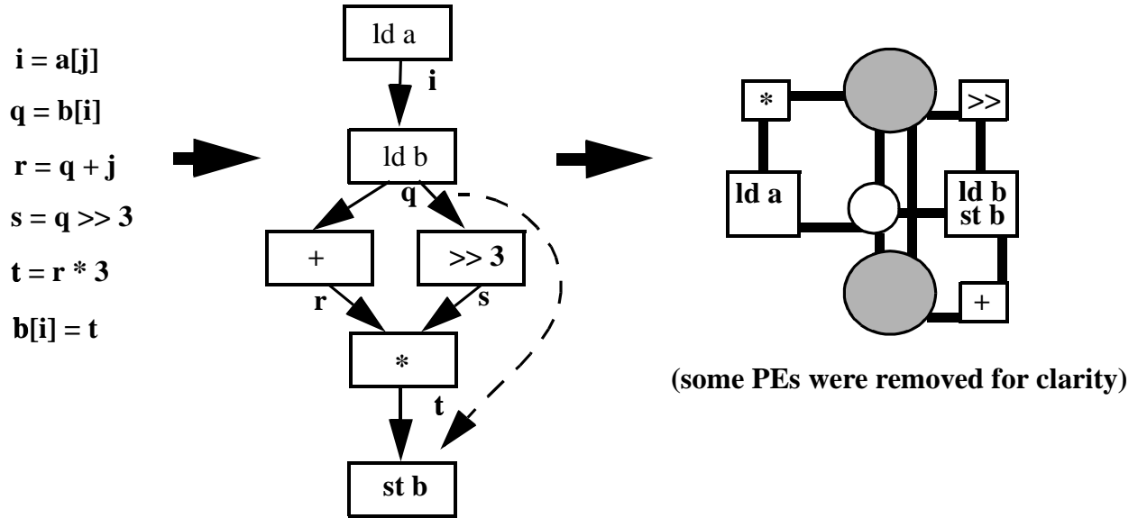
Figure 2: Dataflow Graphs and Operation Assignment
