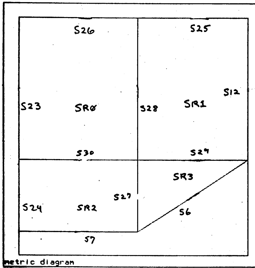
Fig. 54. Space Graph
