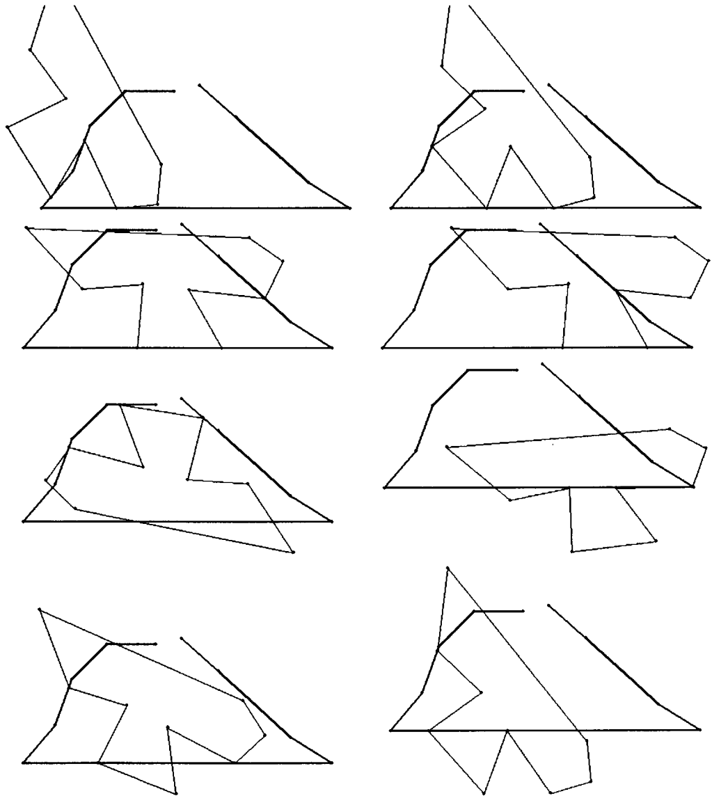
Figure 3.26: Simulation 7: generated and rejected poses. A sample of some of the rejected candidates.
