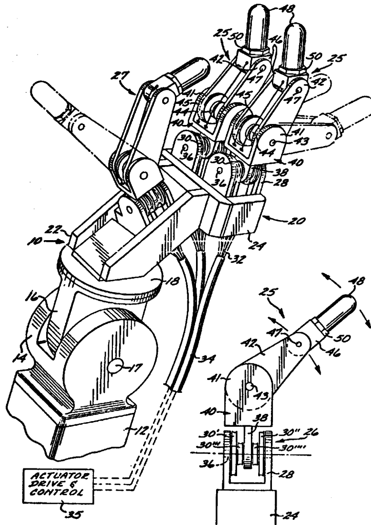
Figure 2.1: The Salisbury-JPL hand, from Salisbury [90].
