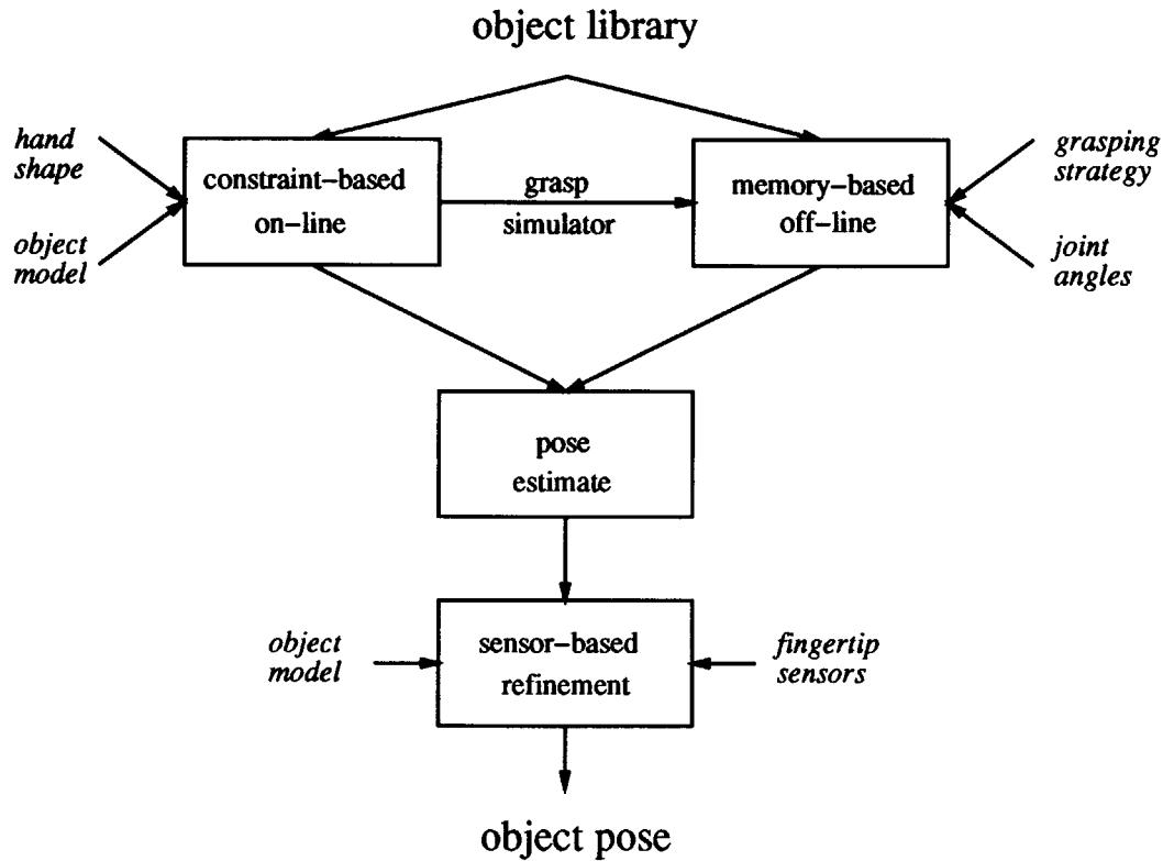
Figure 1.4: Algorithms and their relationship. The algorithms studied in this report, and their relationship, are diagrammed in this figure.
