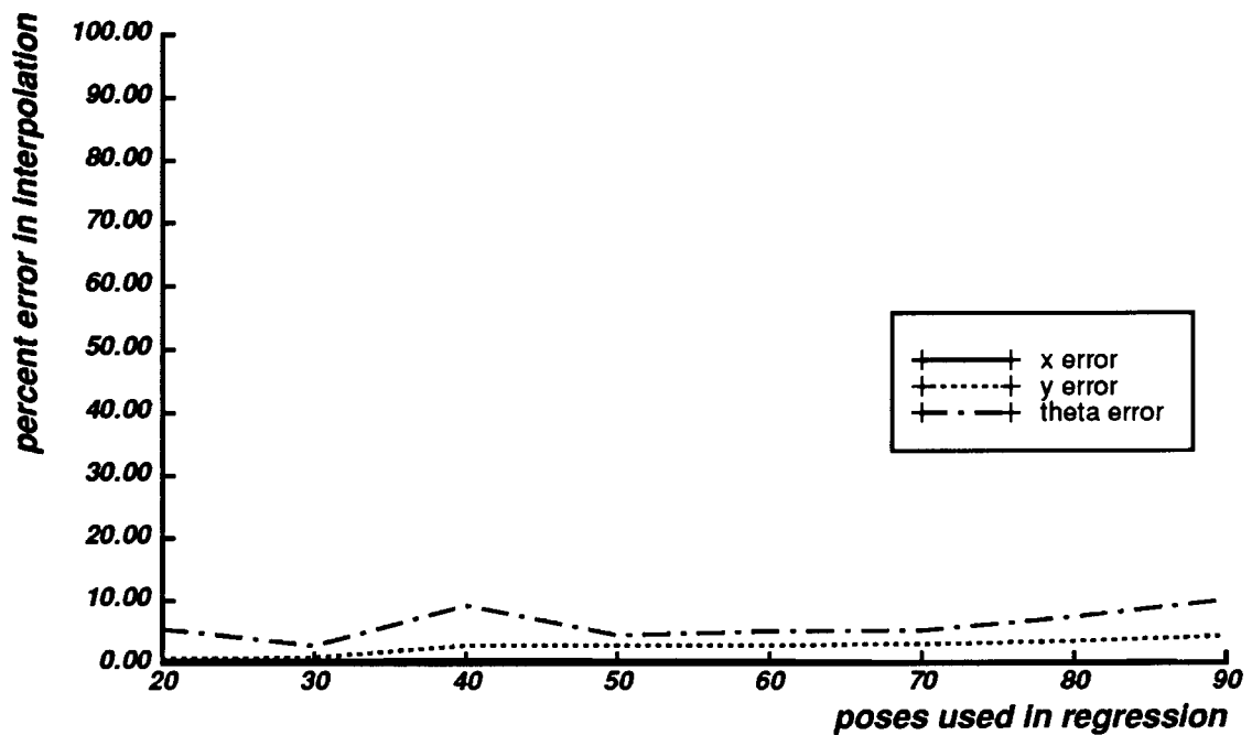
Figure 4.8: Typical interpolation error. The error in interpolation, for object x , y , and \theta , is plotted against the number of configurations used in the regression. This plot is representative of the performance of the method under most tested configurations.
