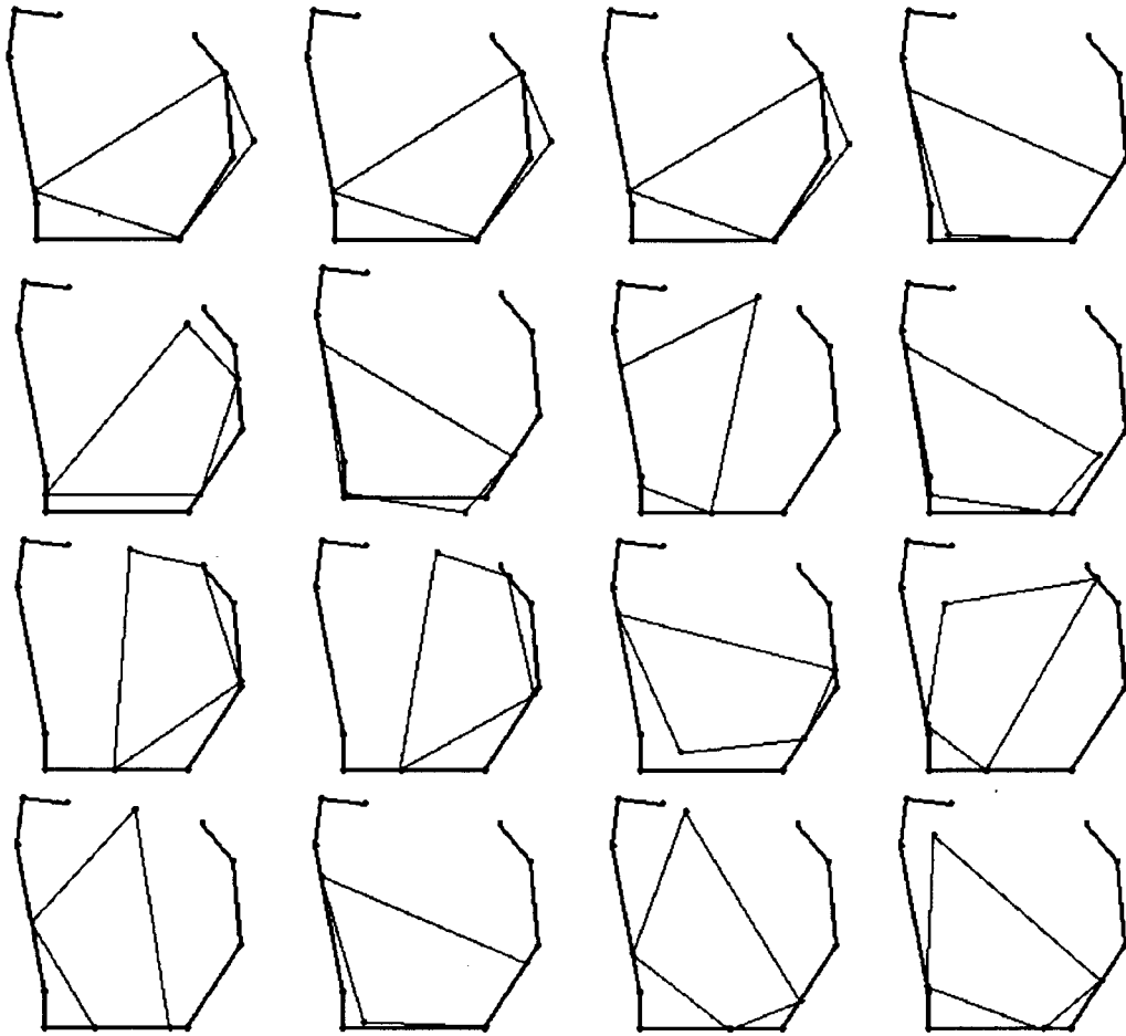
Figure 3.32: Trial 1: generated and rejected poses. These poses were found by the generator, and rejected by the verifier using either the joint torque or intersection constraints.
