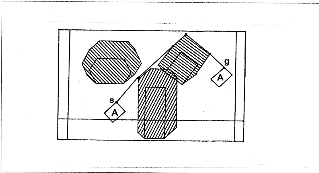
Figure 3. The Findpath problem and its formulation using the CO_A^v(B_j) . The shortest collision-free paths connect the origin and the destination via the vertices of the CO polygons.
