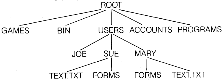
Figure 3-3: A sample hierarchical directory structure
