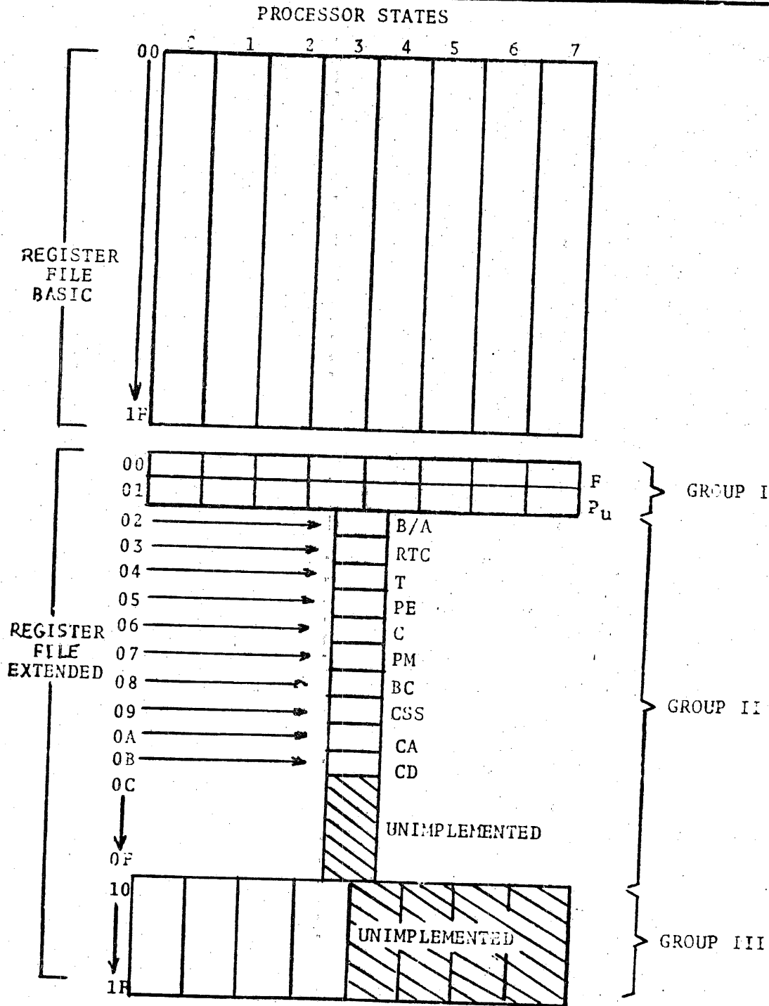
FIGURE 3: REGISTER FILE ORGANIZATION (HEXADECIMAL NOTATION)
