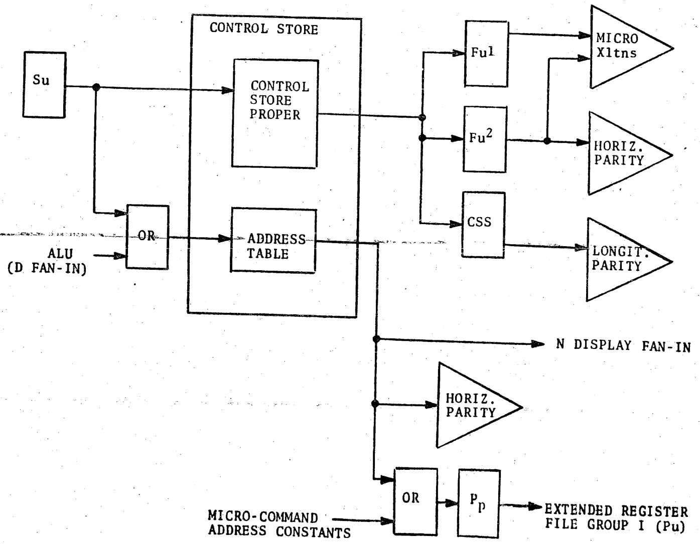
FIGURE 6 - CONTROL STORE AND PERIPHERY
