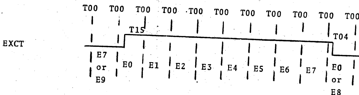
FIGURE 7: EXTENDED REGISTER FILE, GROUP III SIGNAL TIMING
