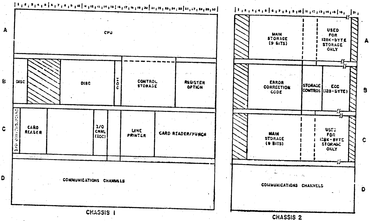
FIGURE 2 PROCESSOR ELEMENTS WITHIN THE 7100 PROCESSOR SYSTEM
