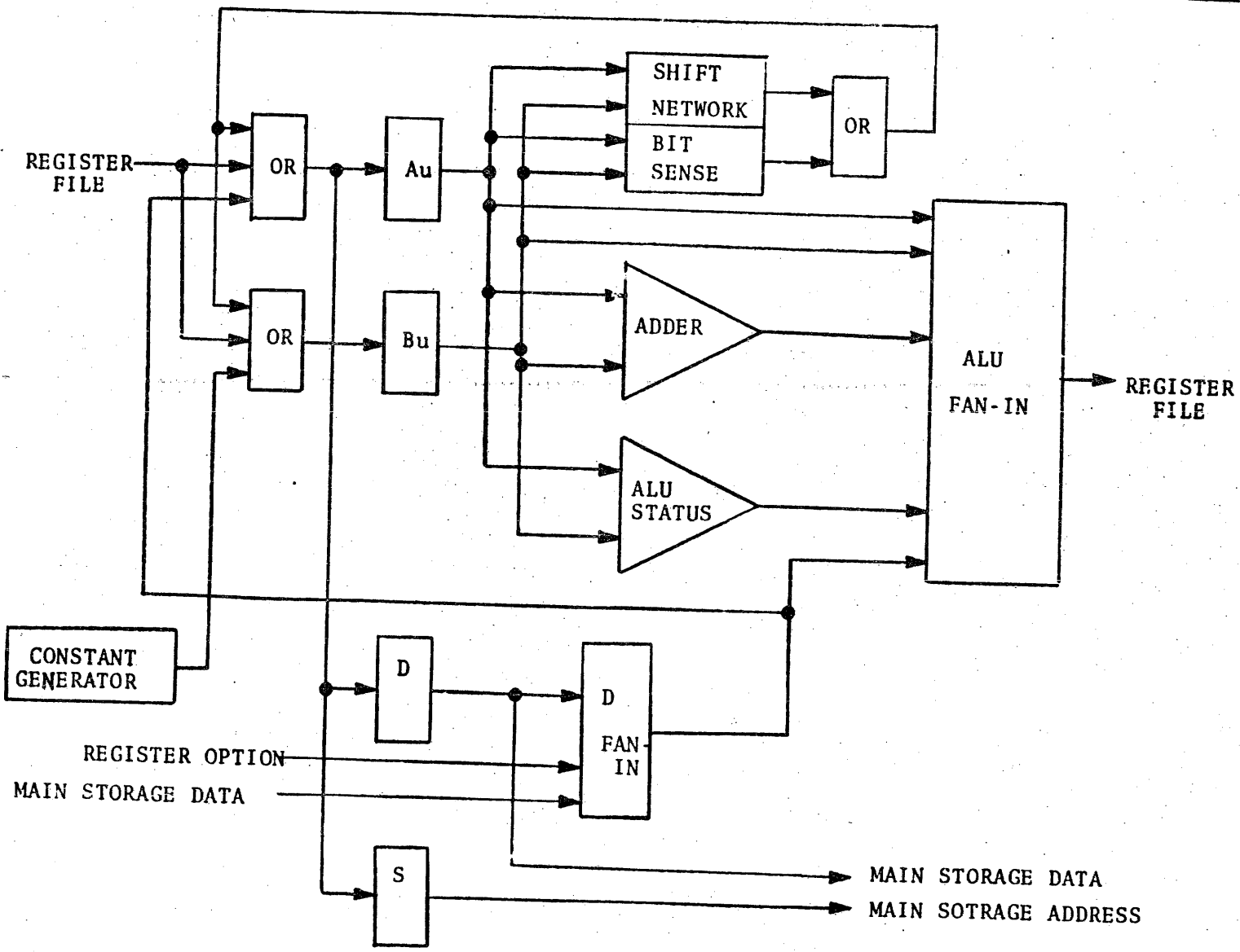
FIGURE 5 - ALU BLOCK DIAGRAM
