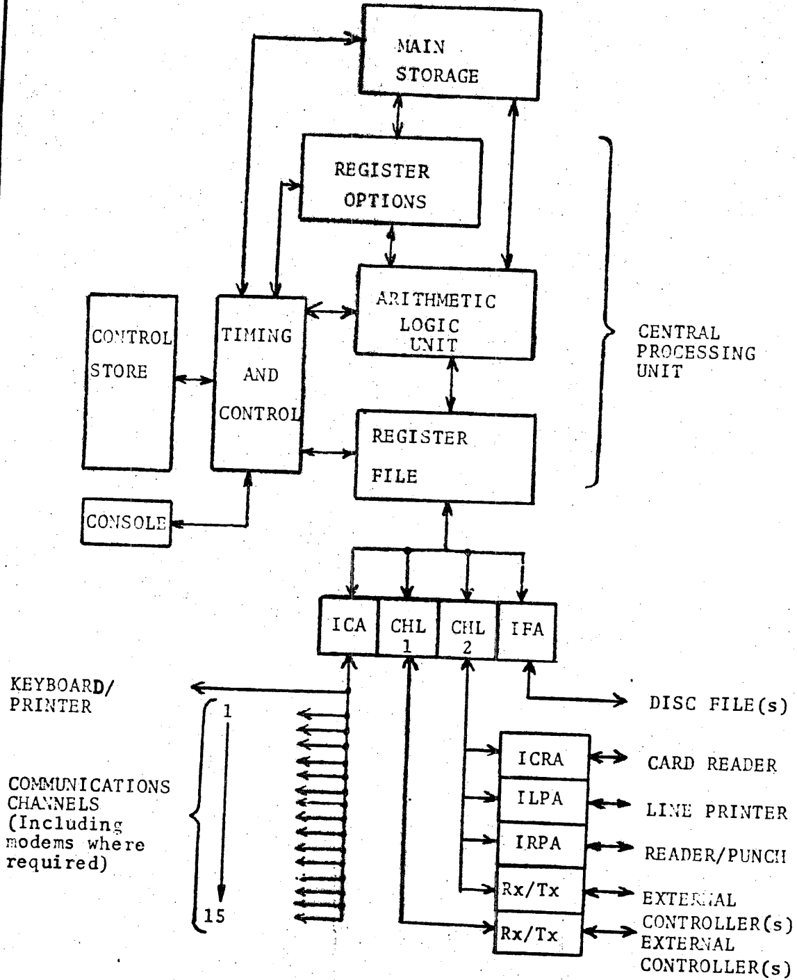
FIGURE 1: 7300 PROCESSOR BLOCK DIAGRAM
