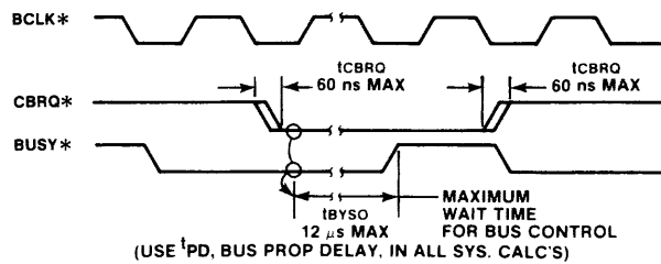
Fig. 23 Common Bus Request AC Timing
