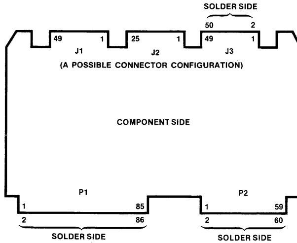
Fig. 32 Connector and Pin Numbering
