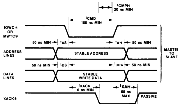
Fig. 19 Write AC Timing
