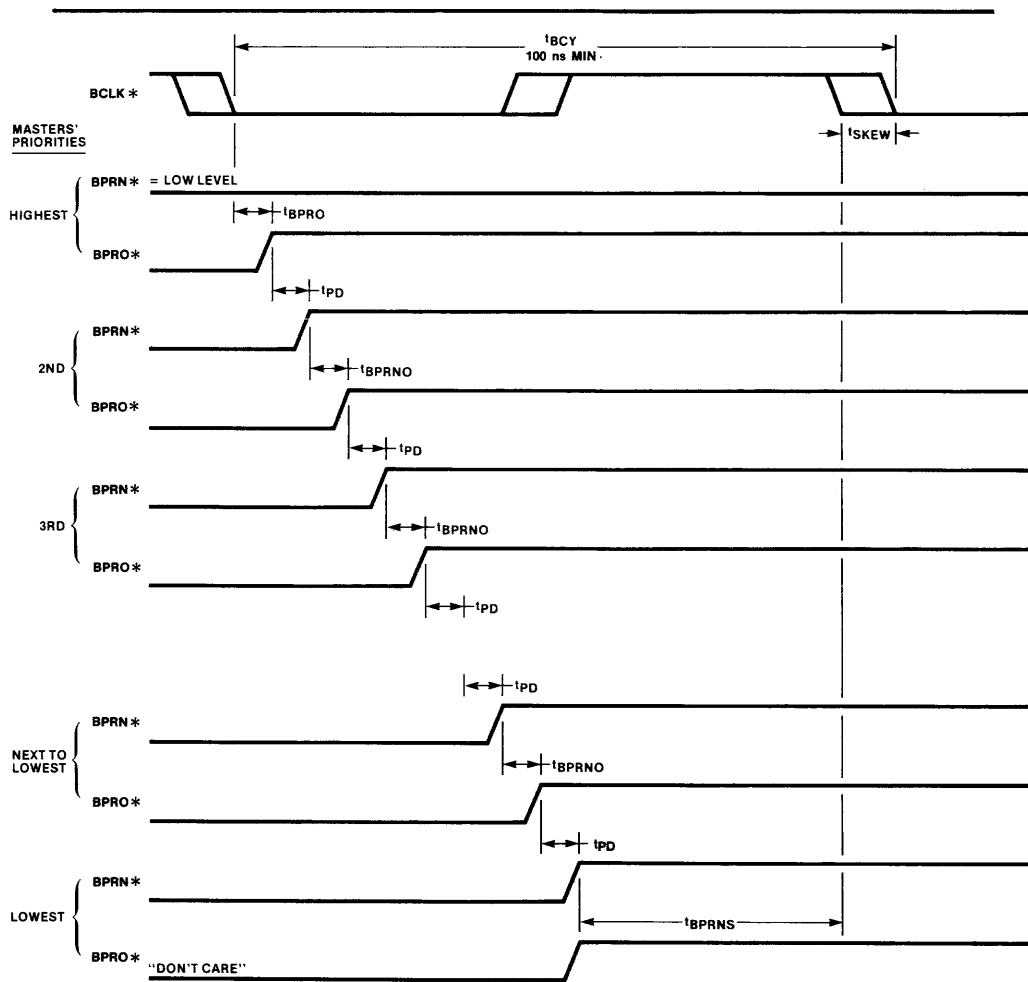
Fig. 24 Serial Priority AC Timing
