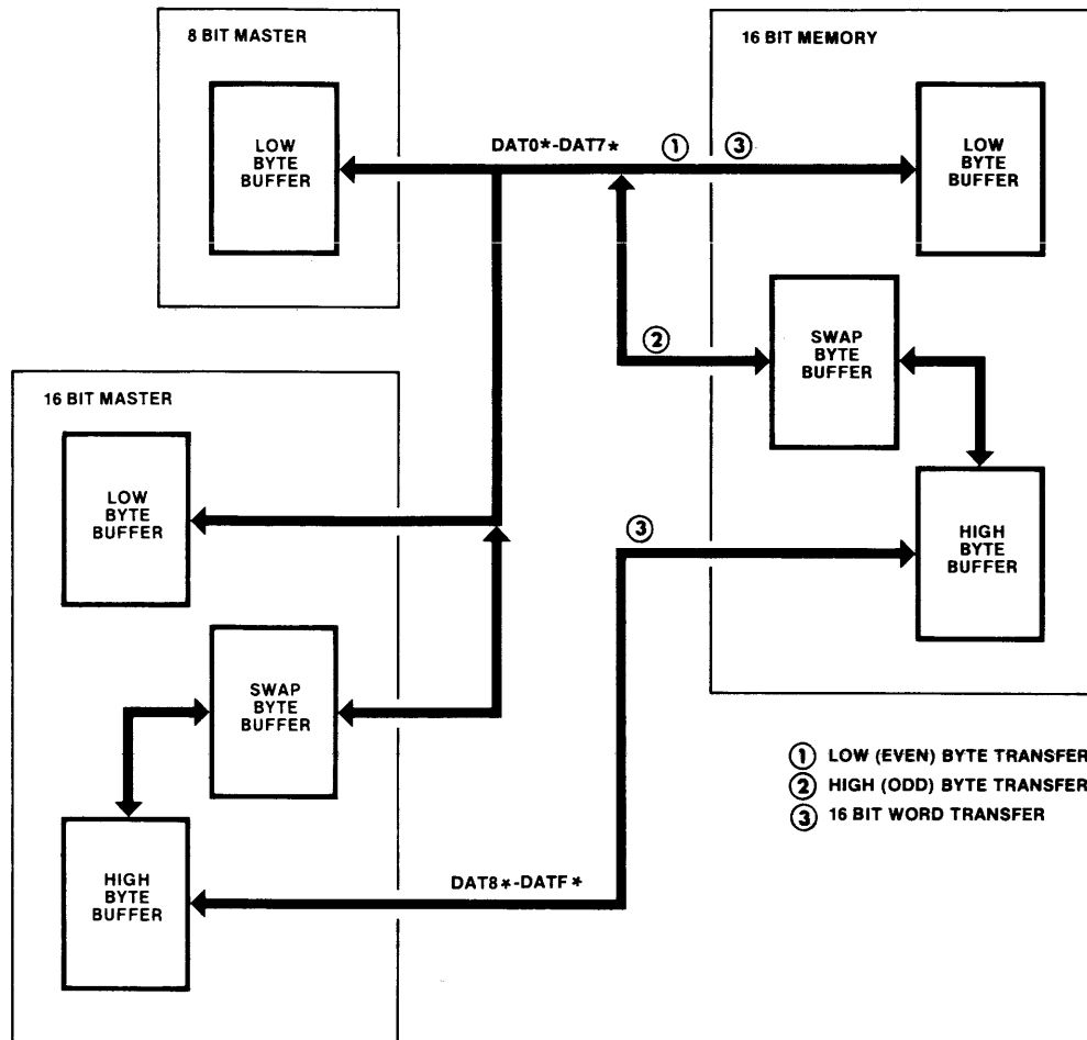
Fig. 6 796 Bus Data Line Usage
