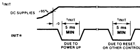
Fig. 28 Initialize AC Timing
