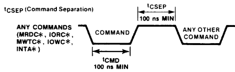
Fig. 27 Command Separation AC Timing
