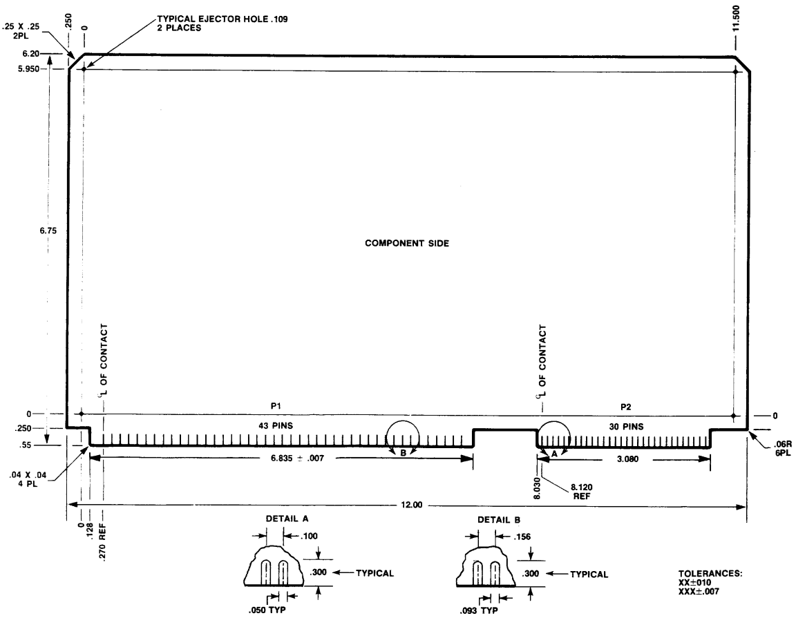
Fig. 33 Standard Printed Wiring Board Outline
