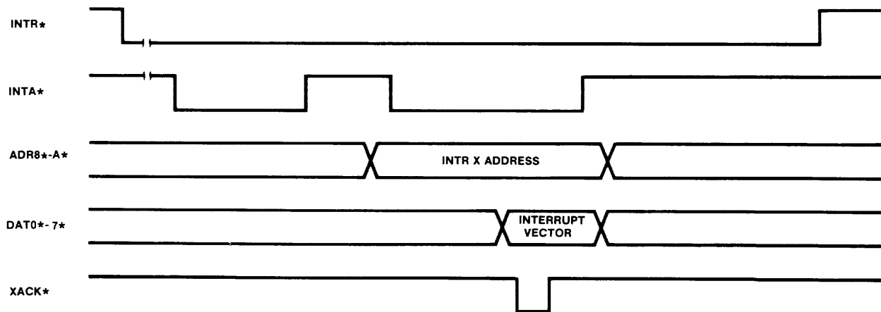
Fig. 13 Bus Vectored (BV) Interrupt Logic
