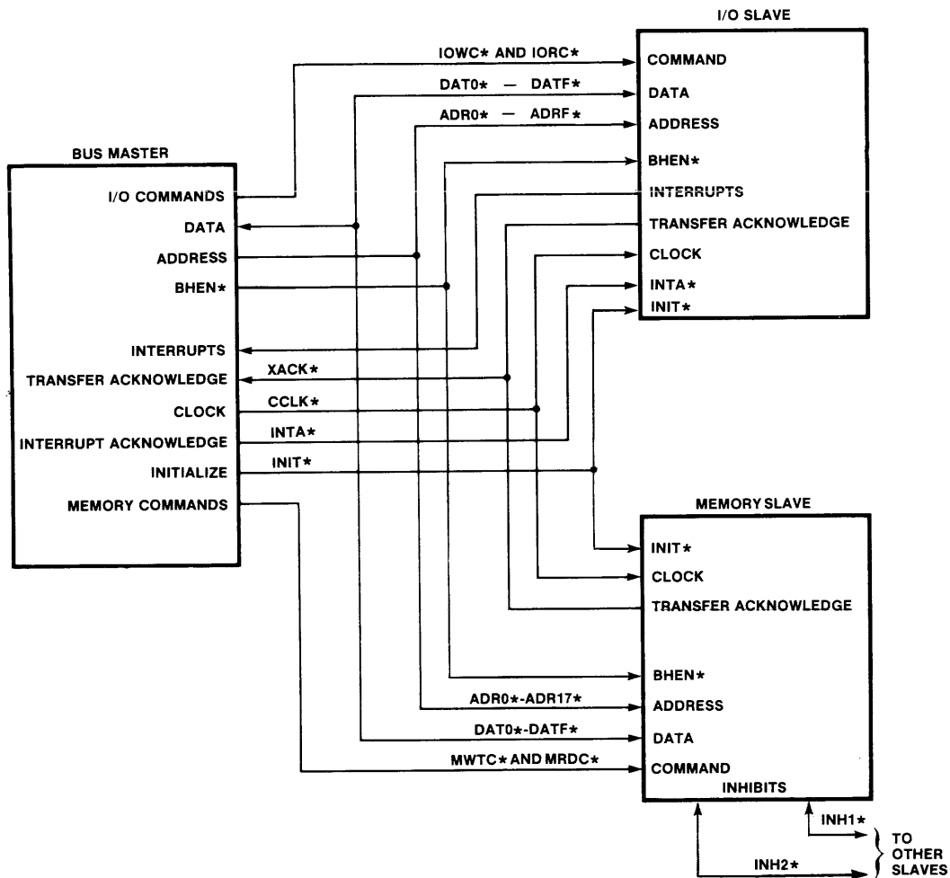
Fig. 2 796 Bus Interface Lines
