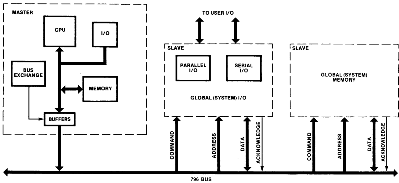
Fig. 1 796 Bus Master and Slave Example
