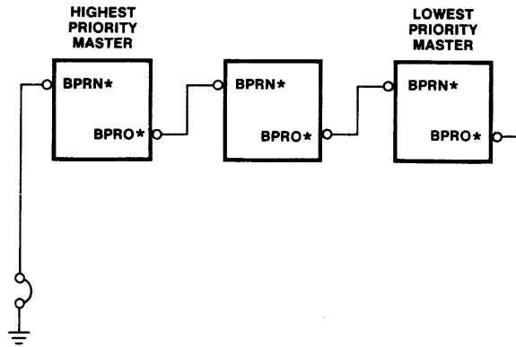
Fig. 14 Serial Priority Technique
