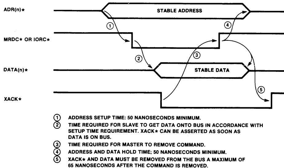
Fig. 7 Memory or I/O Read Timing
