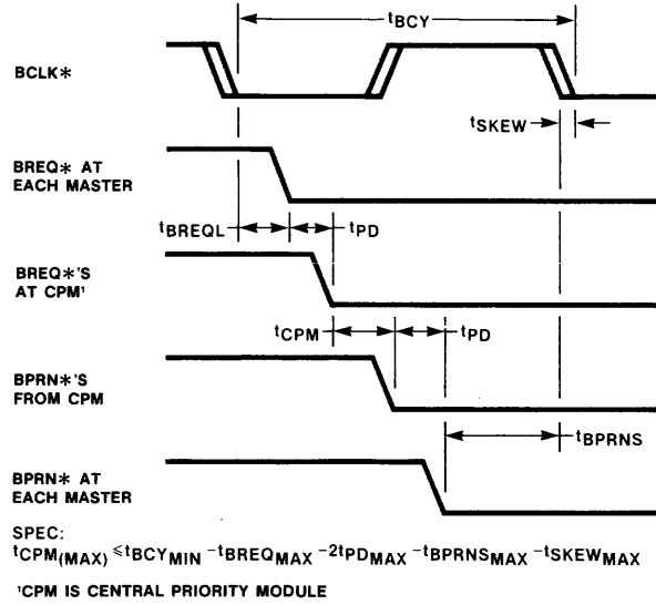
Fig. 25 Parallel Priority AC Timing
