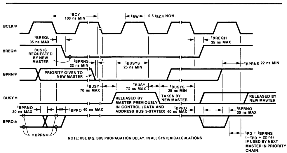
Fig. 22 Bus Exchange AC Timing
