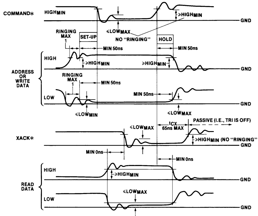
Fig. 16 Setup, Hold, and Command Ringing Summary
