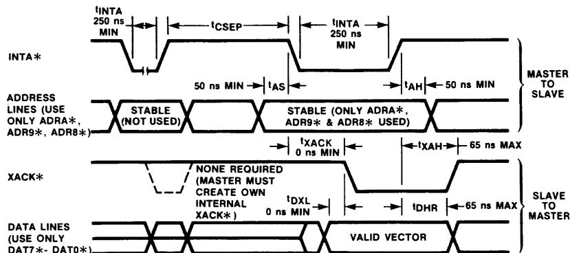
Fig. 21 Bus Vectored (BV) Interrupt AC Timing
