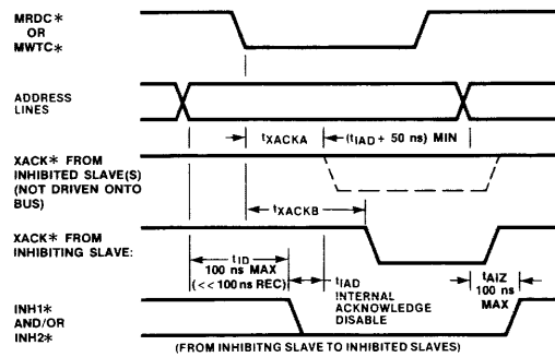
Fig. 20 Inhibit AC Timing
