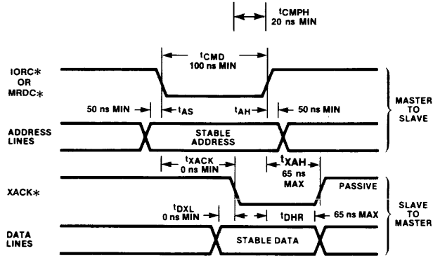
Fig. 18 Read AC Timing
