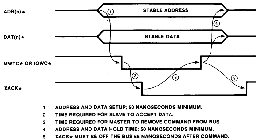
Fig. 8 Memory or I/O Write Timing
