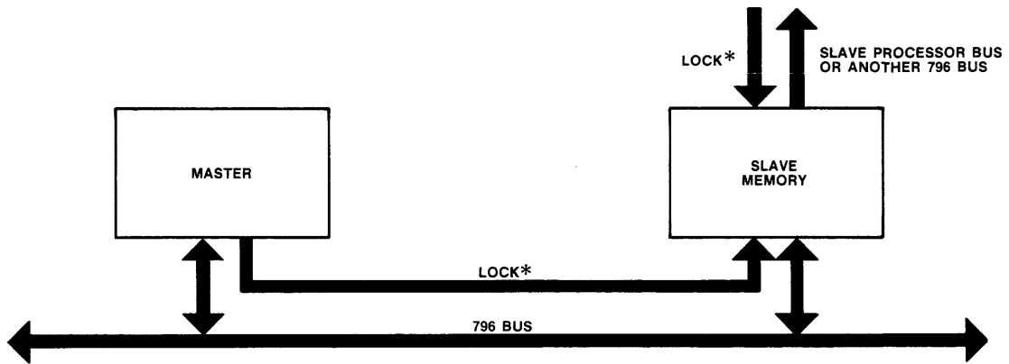
Fig. 10 796 Bus Lock Usage
