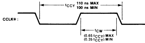
Fig. 26 Constant Clock AC Timing
