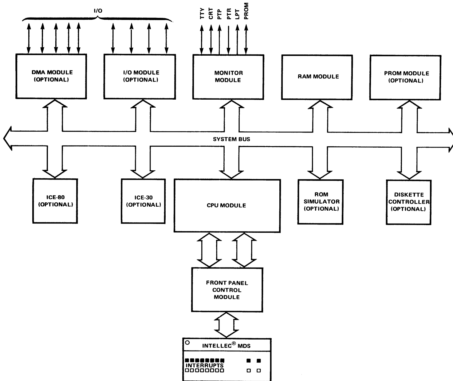
Figure 2-1. INTELLEC® MDS System Block Diagram
