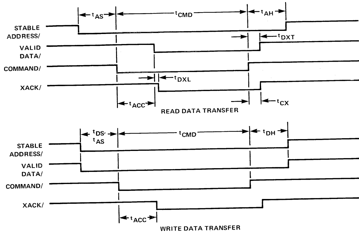
Figure 10-2. Data Transfer
