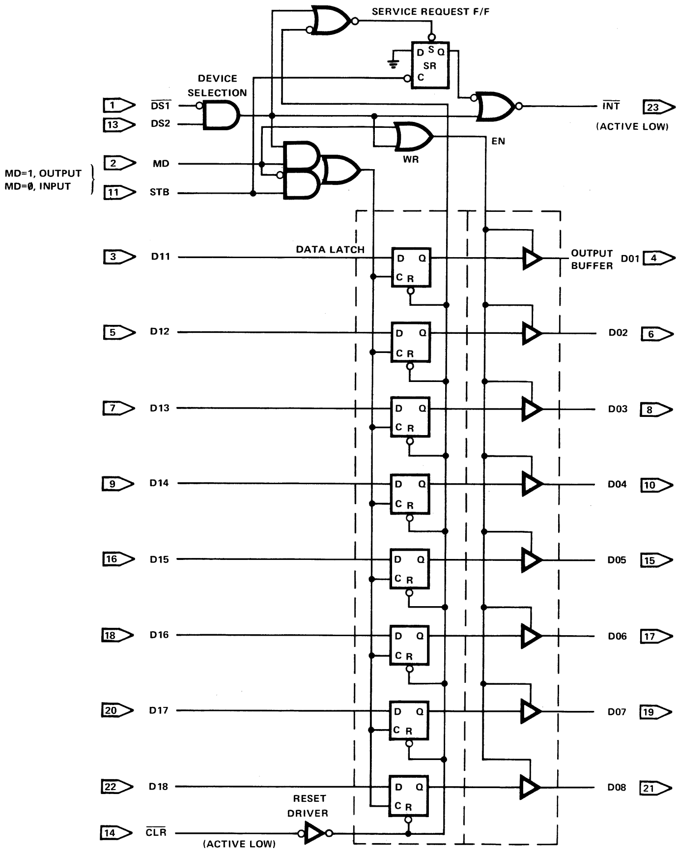
Figure 9-3. 8212 Logic Diagram
