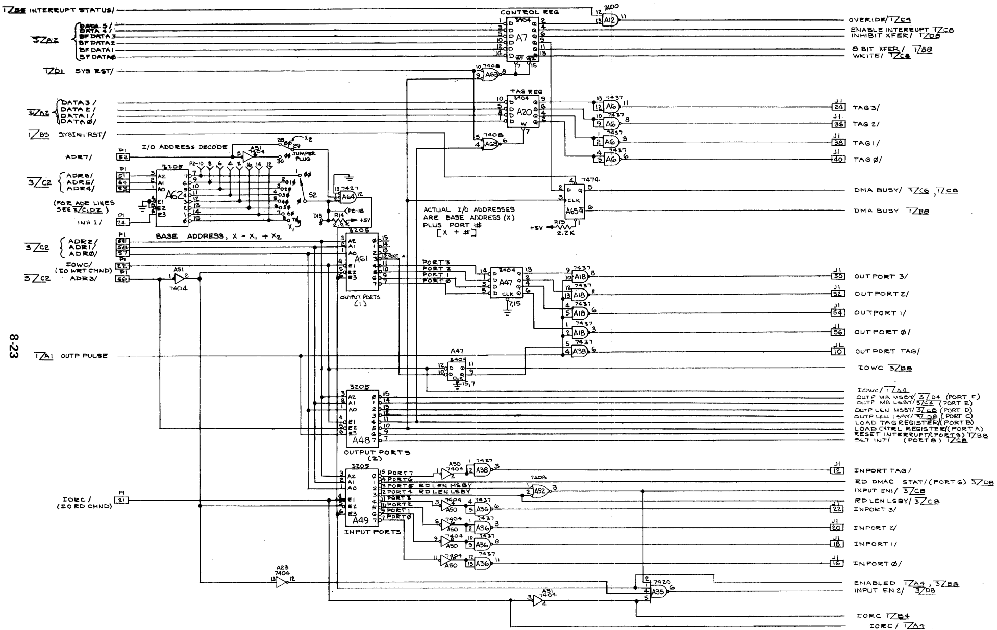
Figure 8-9. DMA Module Schematic (Sheet 2 of 3)
