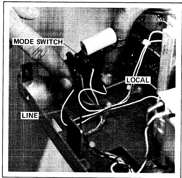
Figure 12-5. Mode Switch
