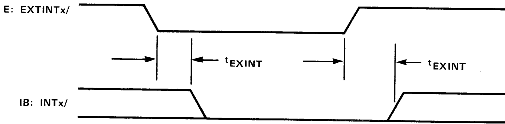
Figure 9-9b. Interrupt Timing
