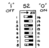
SETTING SHOWN IS FOR I/O2A DEVICE
