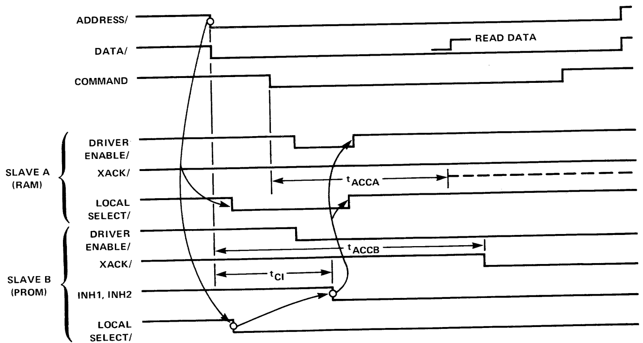
Figure 10-3. Inhibit Operation
