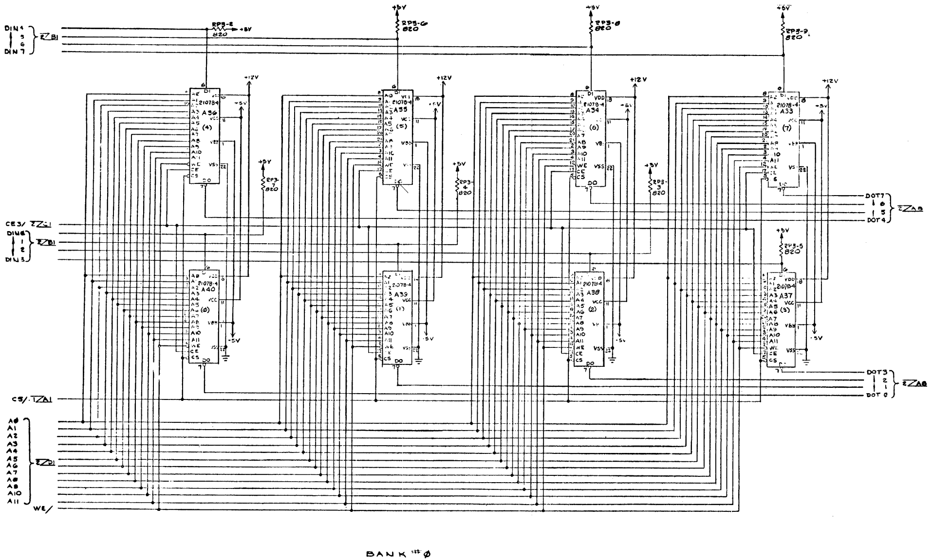
Figure 6-5. RAM Module Schematic (Sheet 3 of 6)
