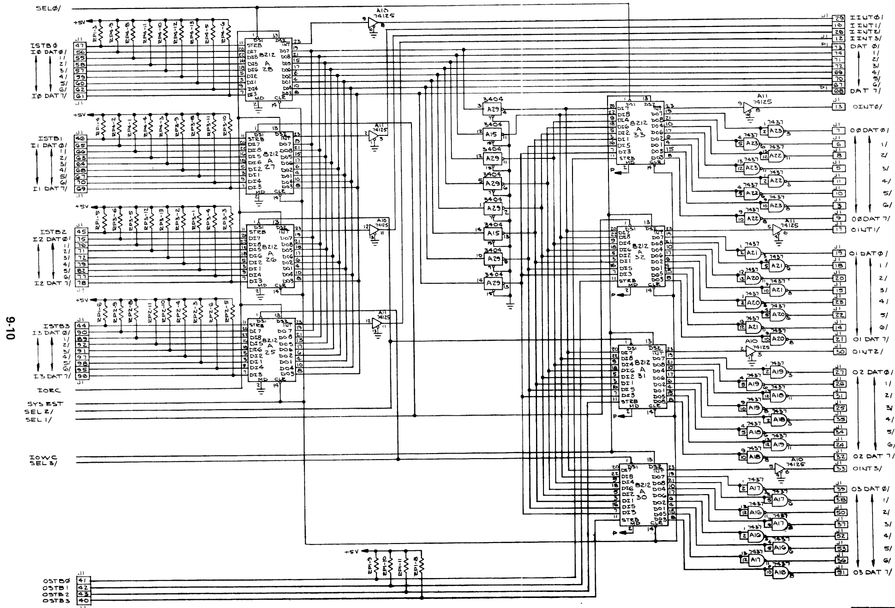
Figure 9-6. I/O Module Schematic (Sheet 2 of 2)
