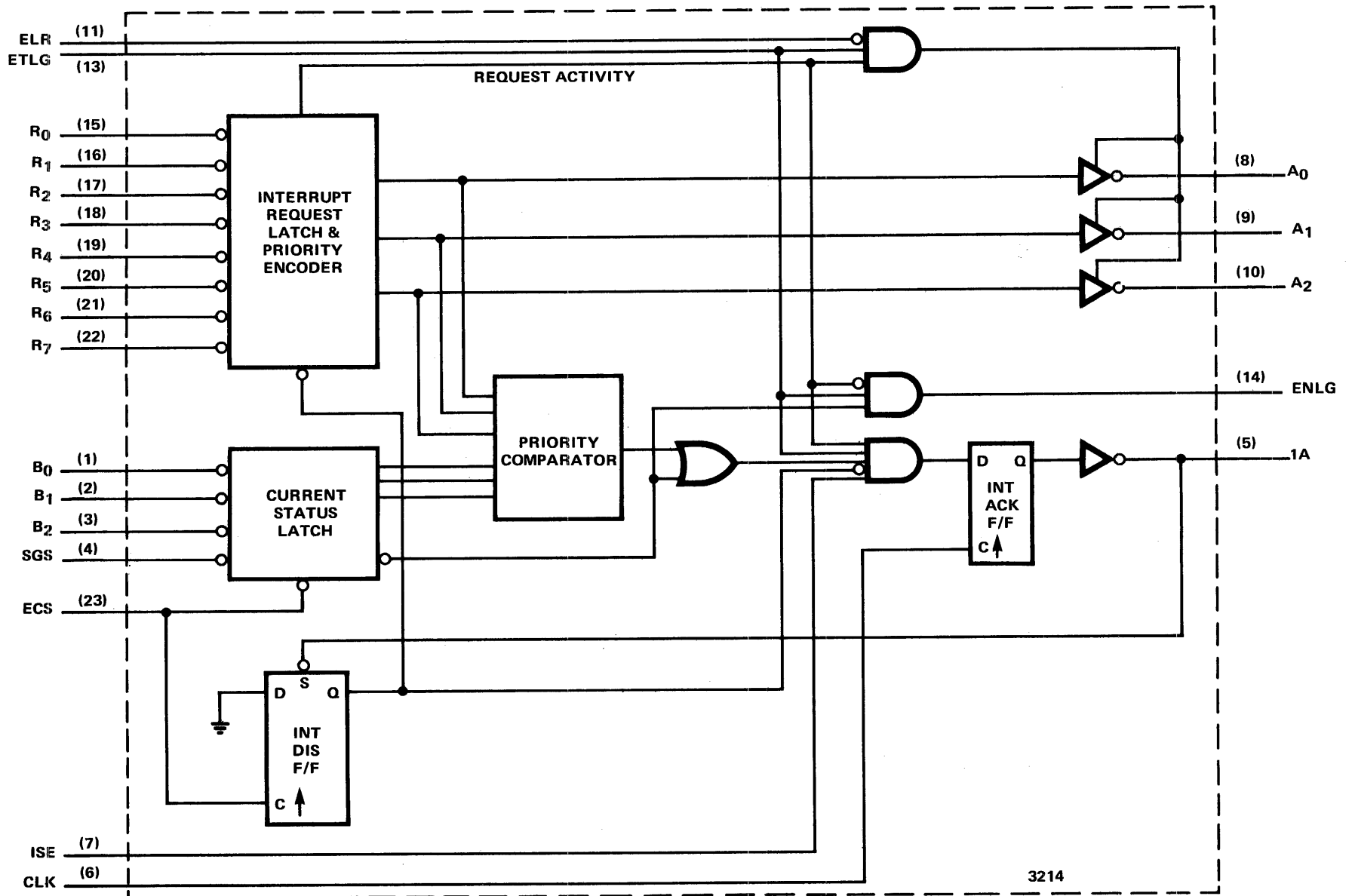
Figure 3-15. 3214 Block Diagram
