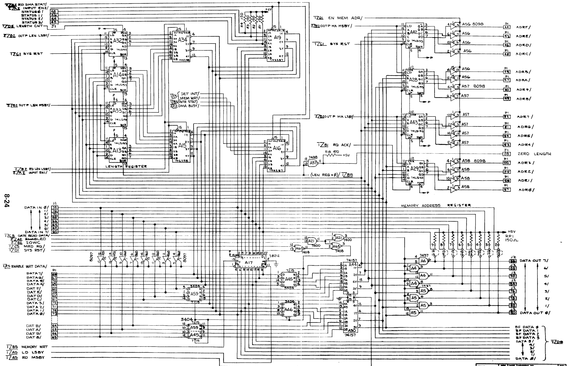
Figure 8-9. DMA Module Schematic (Sheet 3 of 3)
