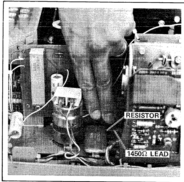
Figure 12-7. Current Source Resistor
