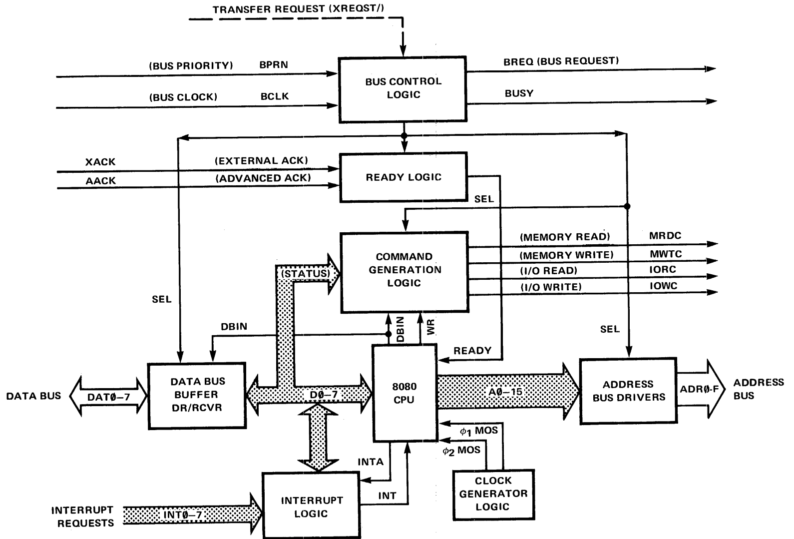
Figure 3-2. Central Processor Module Block Diagram
