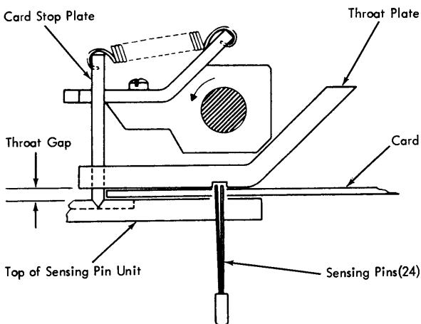
Figure 2-21. Registration (Read Station)
