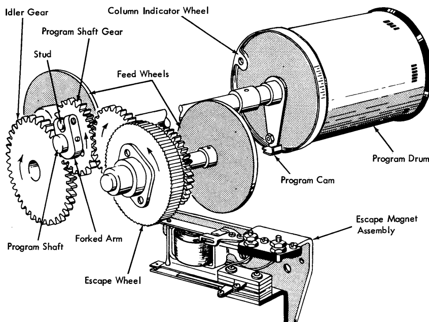
Figure 2-39. Program Shaft
