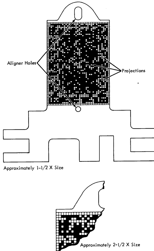
Figure 2-57. Code Plate
