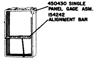
** 450430 GAUGE ASM, CONTROL PANEL SINGLE, 159 X 270 MM 154242 ALIGNMENT BAR
