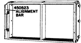
**450531 GAUGE ASM, CONTROL PANEL, 101, 286 X 505 MM 450523 ALIGNMENT BAR
